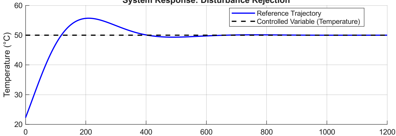
System Response: Disturbance Rejection
