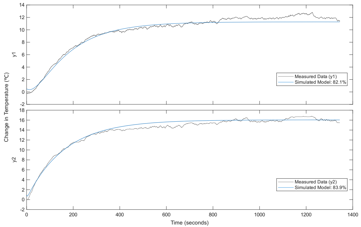
Figure 8: Comparison of the physical sensor data for a 50% duty cycle test case against the simulated SIMO transfer function model for PWM 2.
