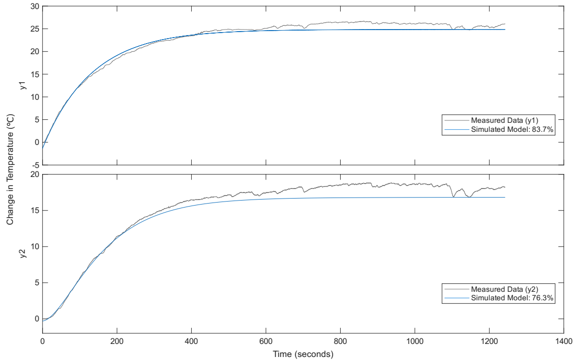
Figure 7: Comparison of the physical sensor data for a 50% duty cycle test case against the simulated SIMO transfer function model for PWM 1.
