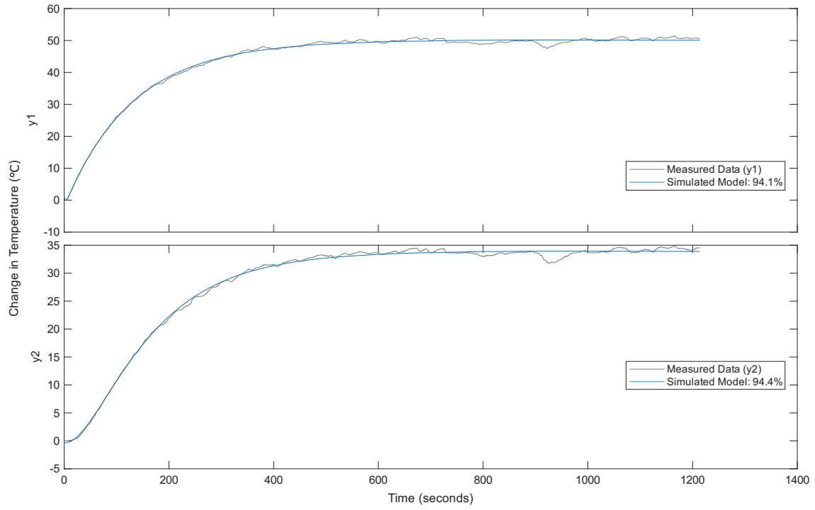
Figure 5: Comparison of the physical sensor data against the simulated SIMO transfer function model for PWM 1.
