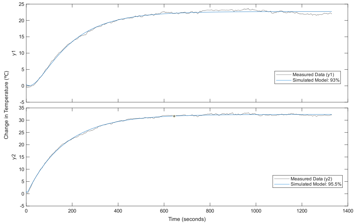
Figure 6: Comparison of the physical sensor data against the simulated SIMO transfer function model for PWM 2.
