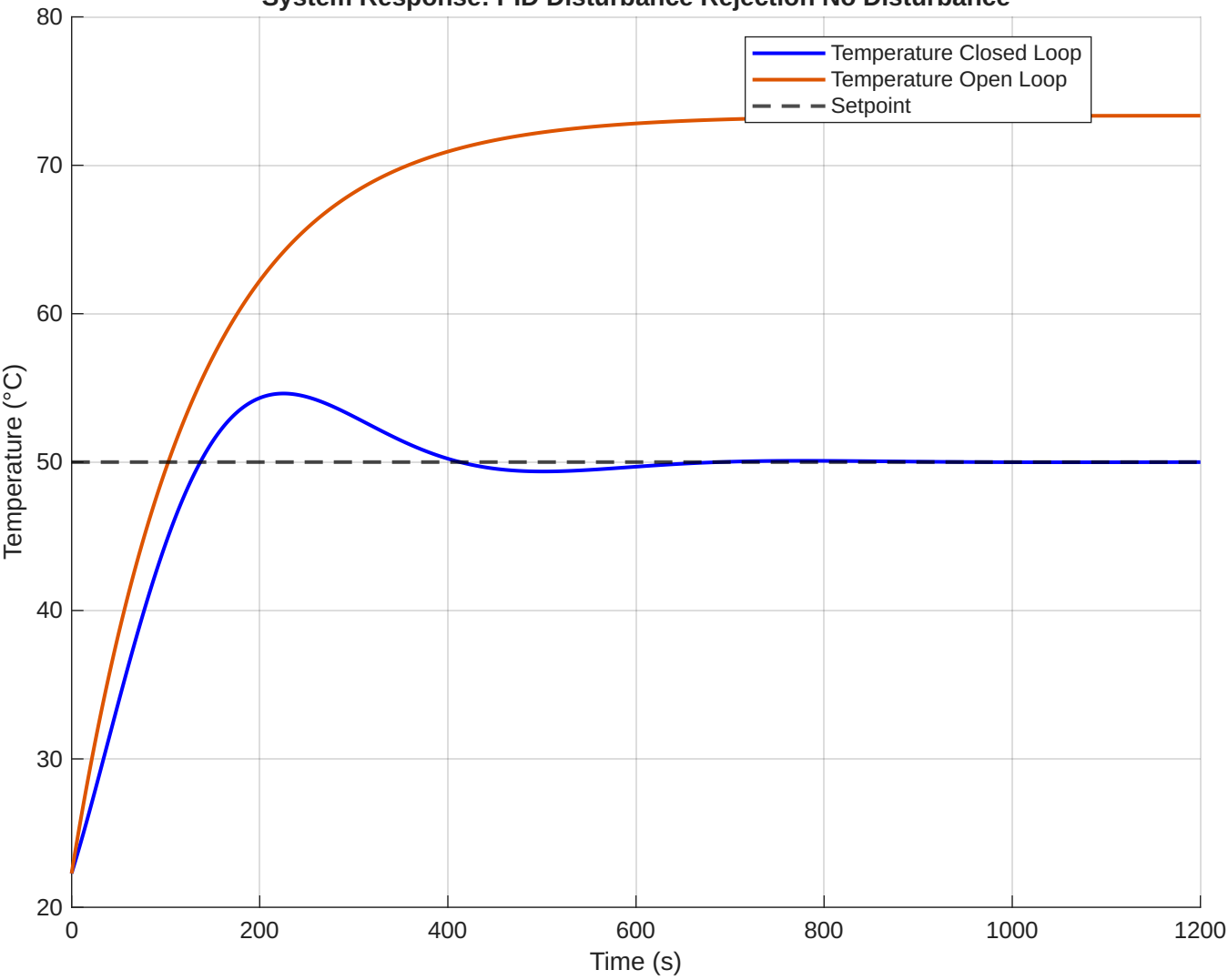
System Response: PID Disturbance Rejection No Disturbance
