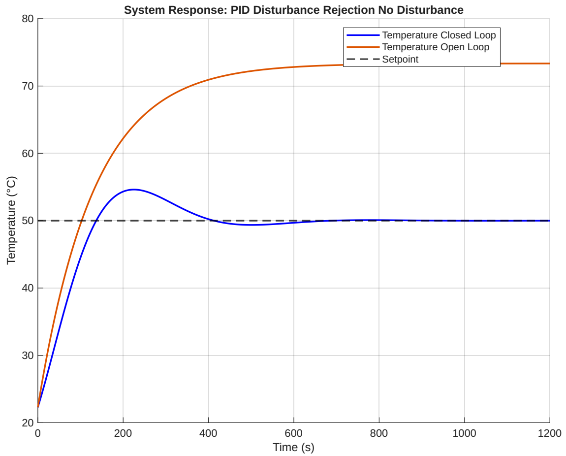
Figure 18: Comparing the closed loop step response of the PID disturbance rejection controller to the open loop step response
