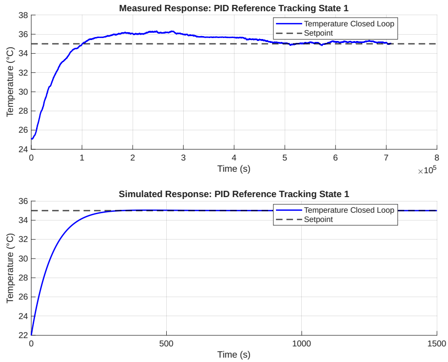
Figure 21: Measured Results for PID reference tracking for state 1
