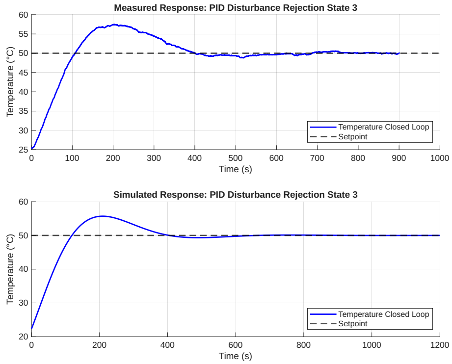
Figure 27: Measured Results for PID disturbance rejection tracking for state 3
