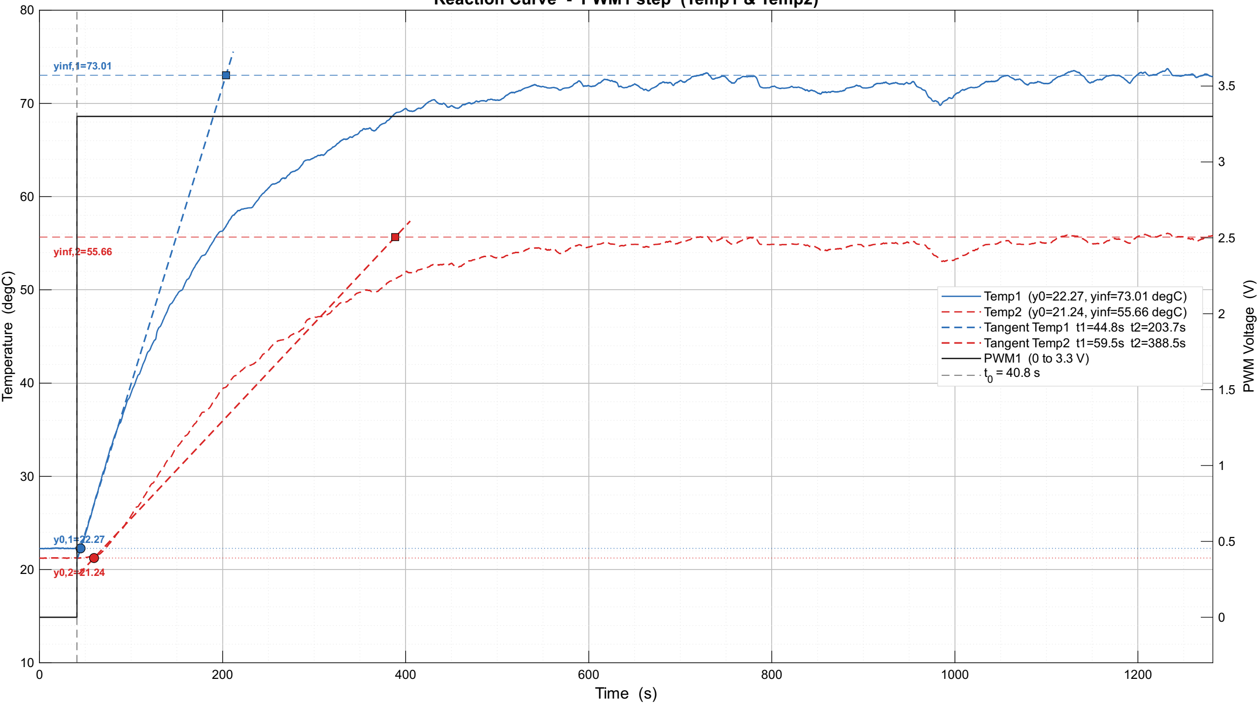
Reaction Curve - PWM1 step (Temp1 & Temp2)
