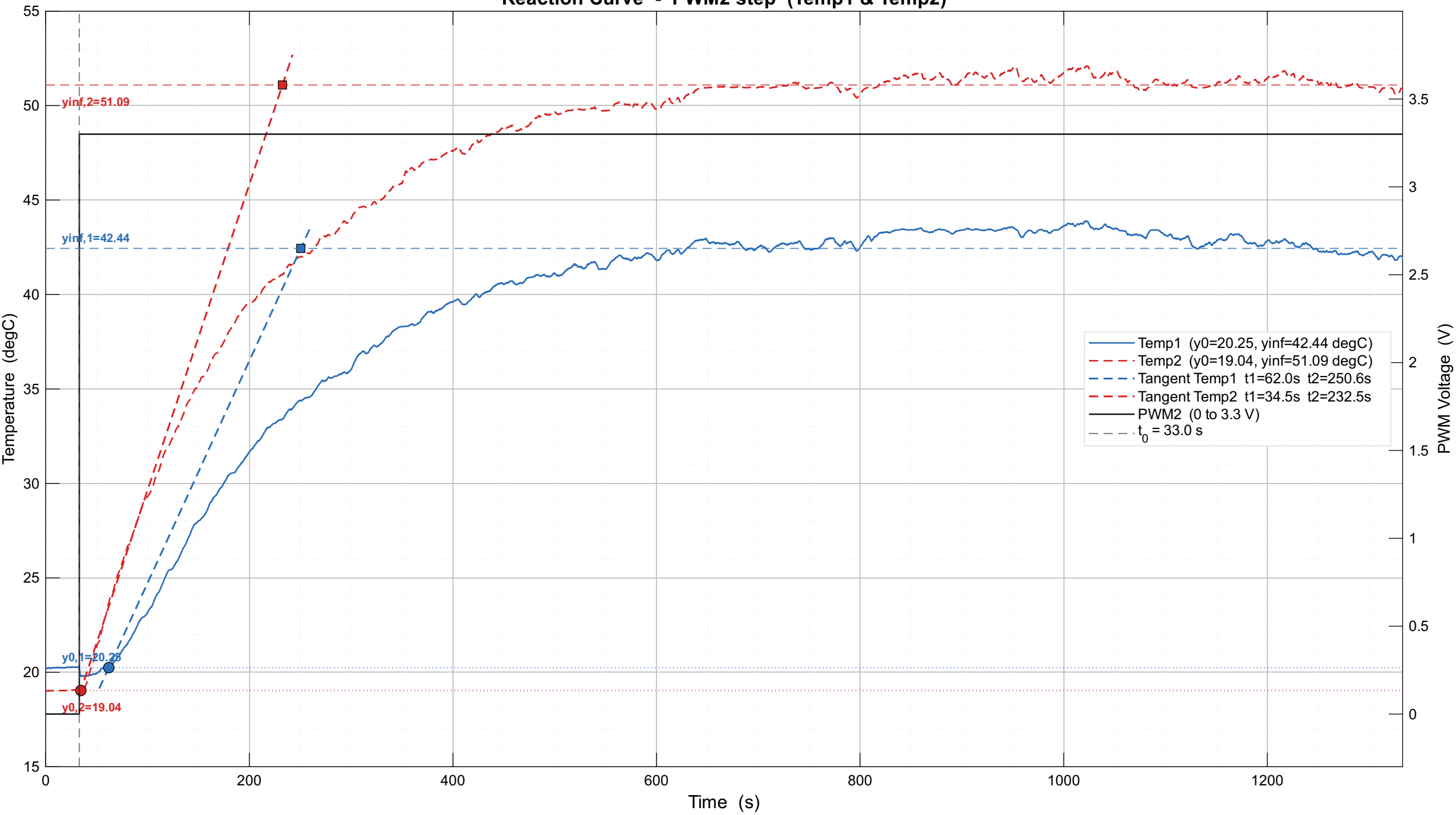
Reaction Curve - PWM2 step (Temp1 & Temp2)
