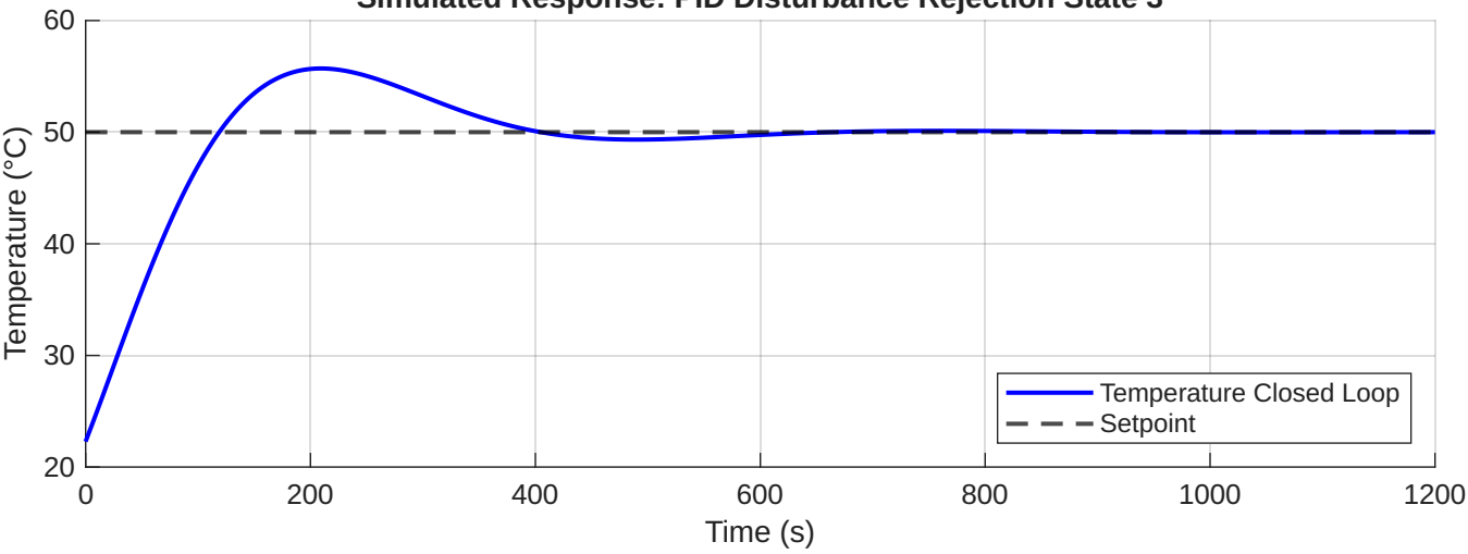
Simulated Response: PID Disturbance Rejection State 3
