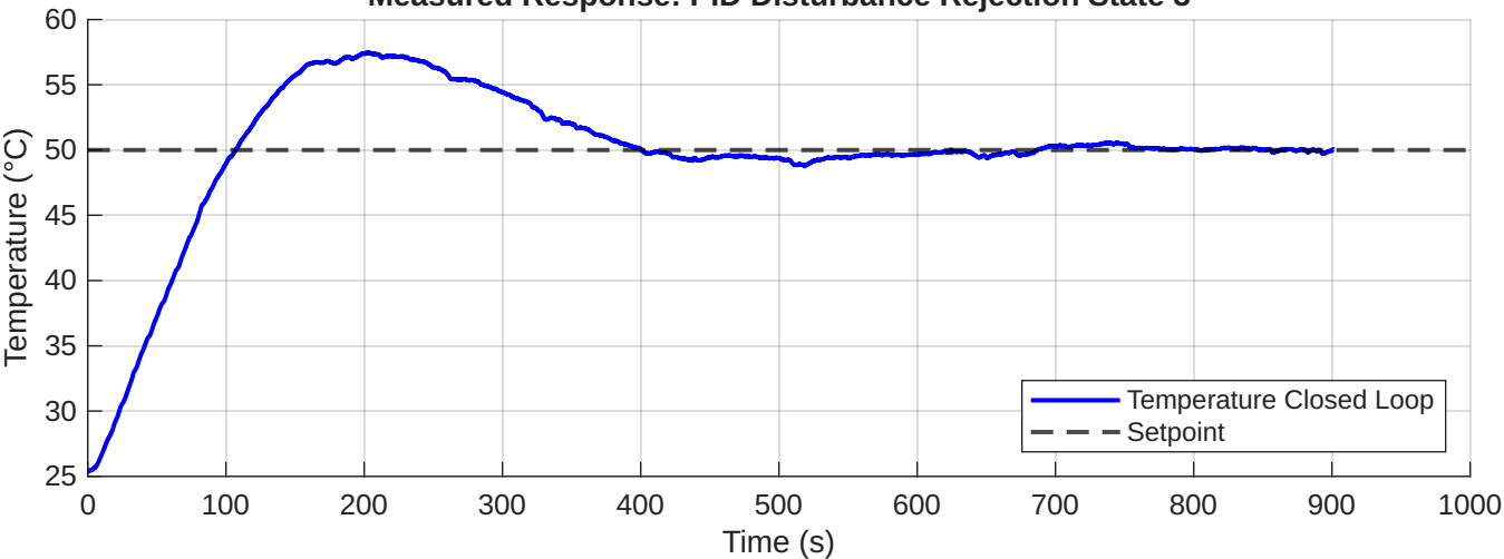
Measured Response: PID Disturbance Rejection State 3
