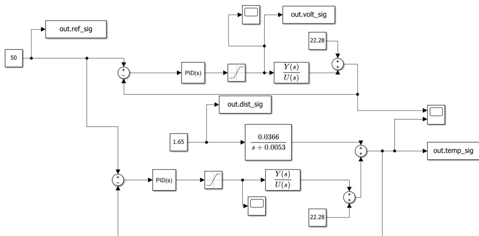
Figure 6: Simulink model for the disturbance rejection PID controller.
