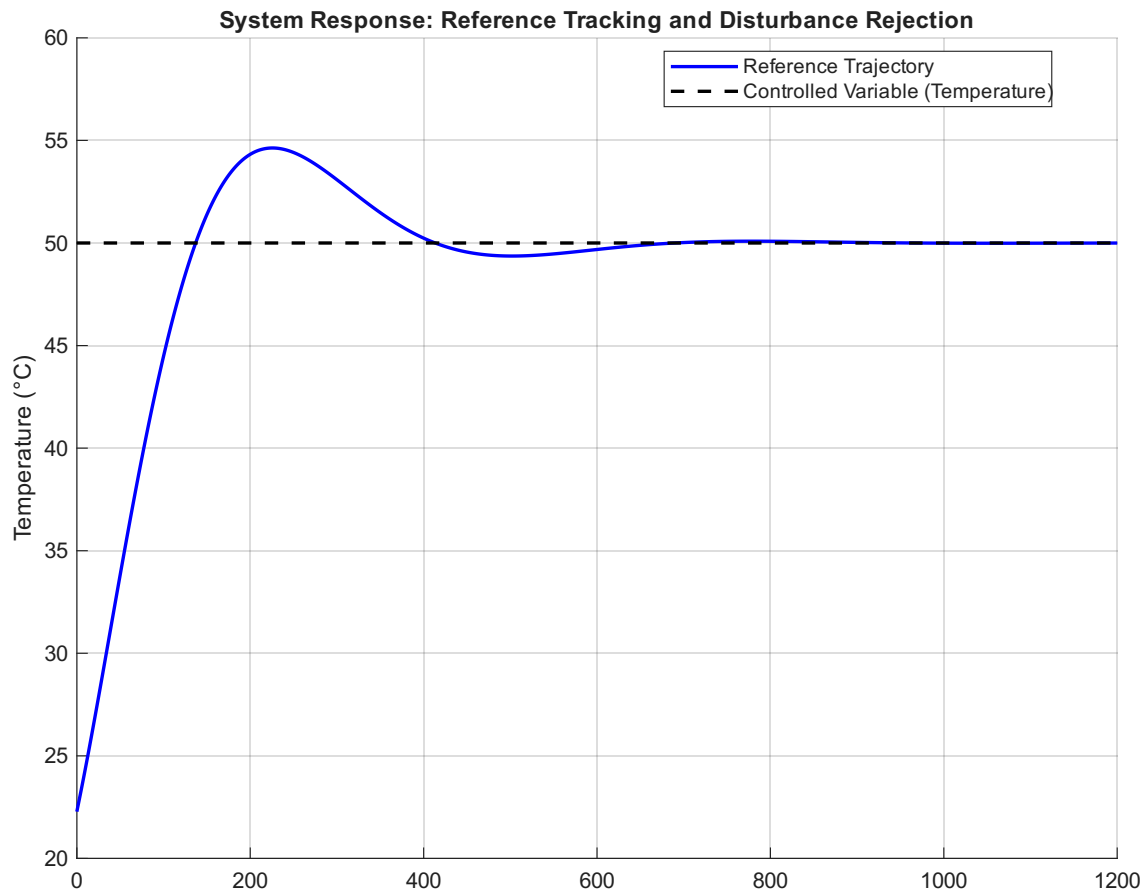
Figure 5: Closed Loop response of PID Disturbance Rejection Controller
