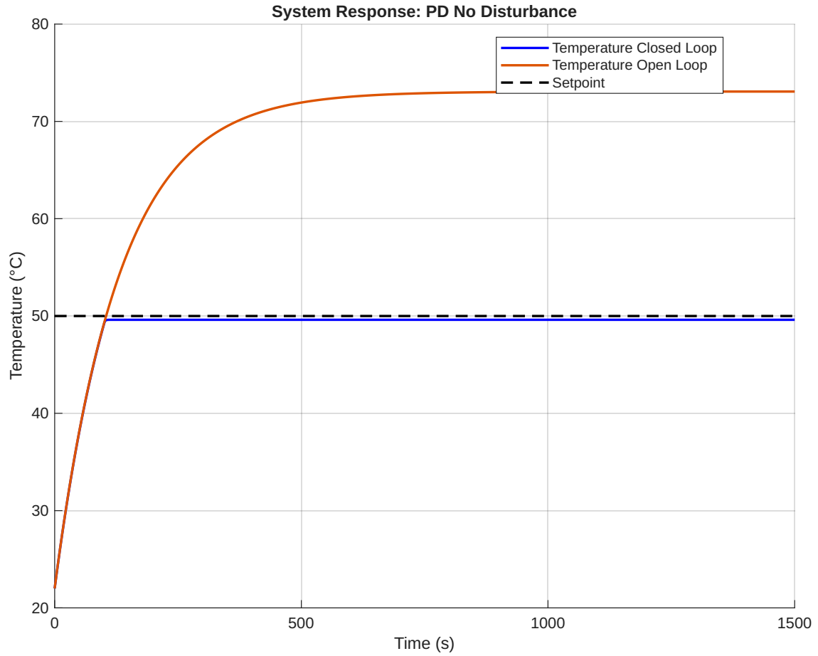
Figure 2: Closed Loop vs Open Loop response of PD Controller
