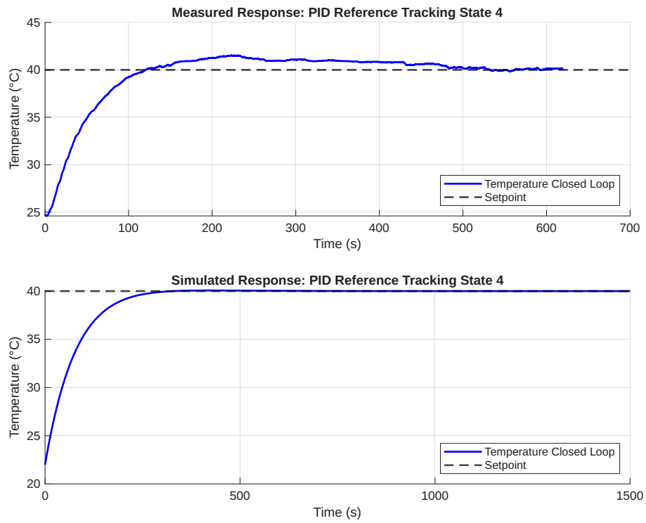
Figure 11: Measured Results for PID reference tracking for state 4
