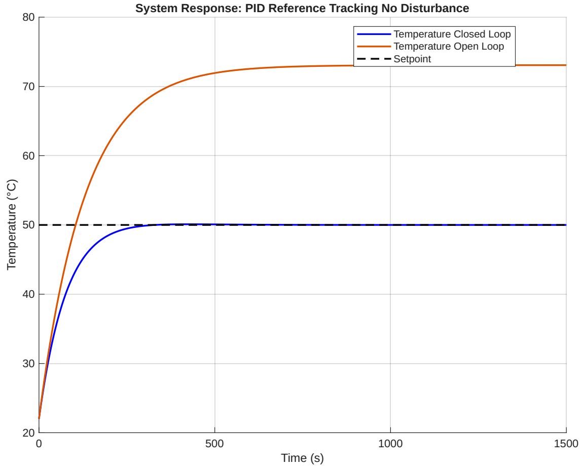
Figure 3: Closed Loop vs Open Loop response of PID Reference Tracking Controller
