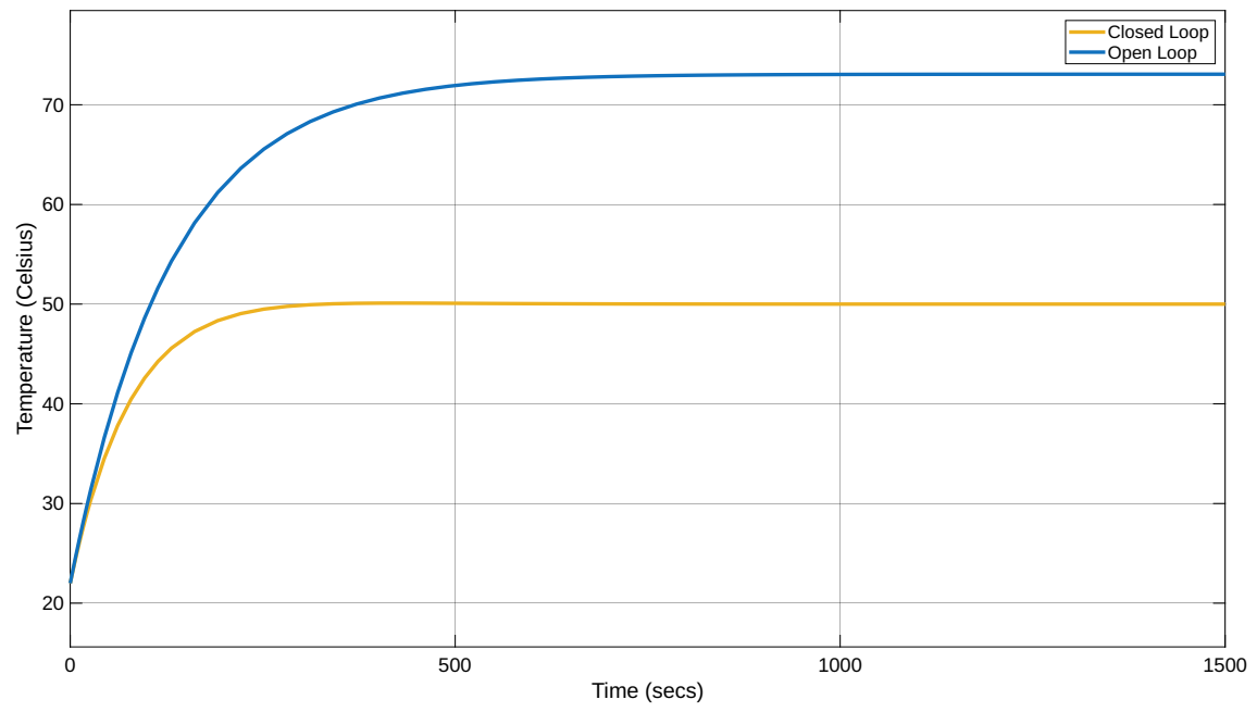
Figure 2: Closed Loop vs Open Loop response of PID Reference Tracking Controller
