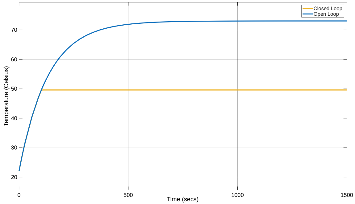
Figure 1: Closed Loop vs Open Loop response of PD Controller
