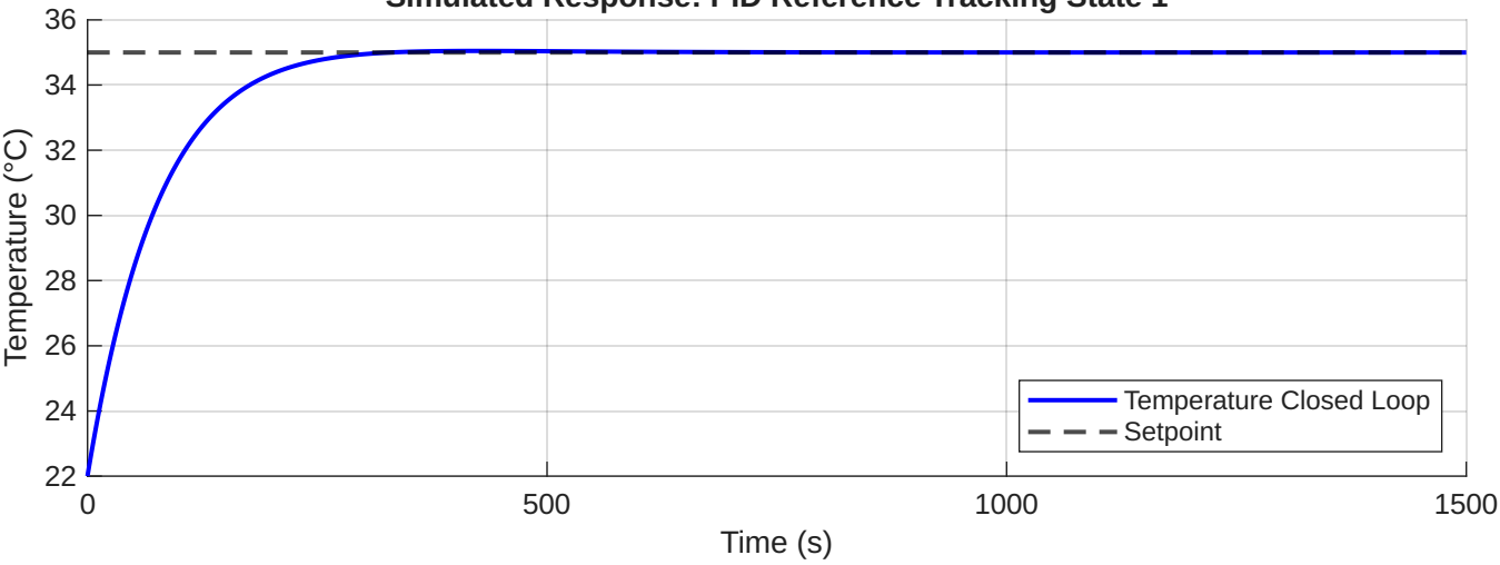
Simulated Response: PID Reference Tracking State 1
