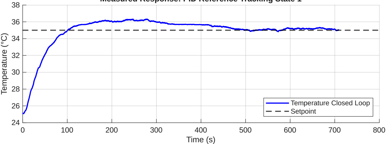
Measured Response: PID Reference Tracking State 1
