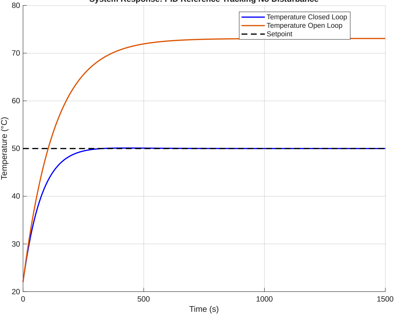
System Response: PID Reference Tracking No Disturbance
