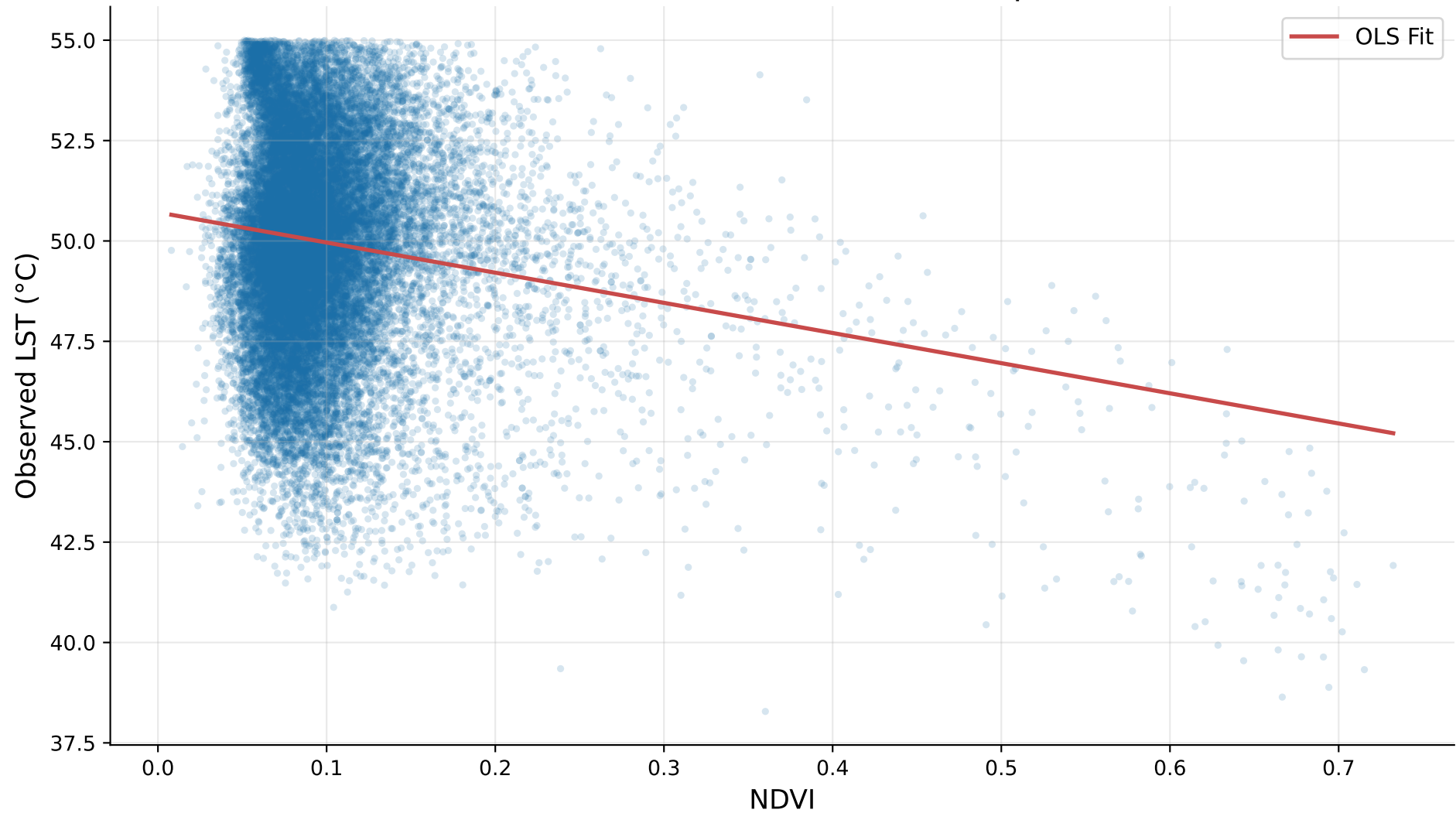
Observed NDVI vs Land Surface Temperature
