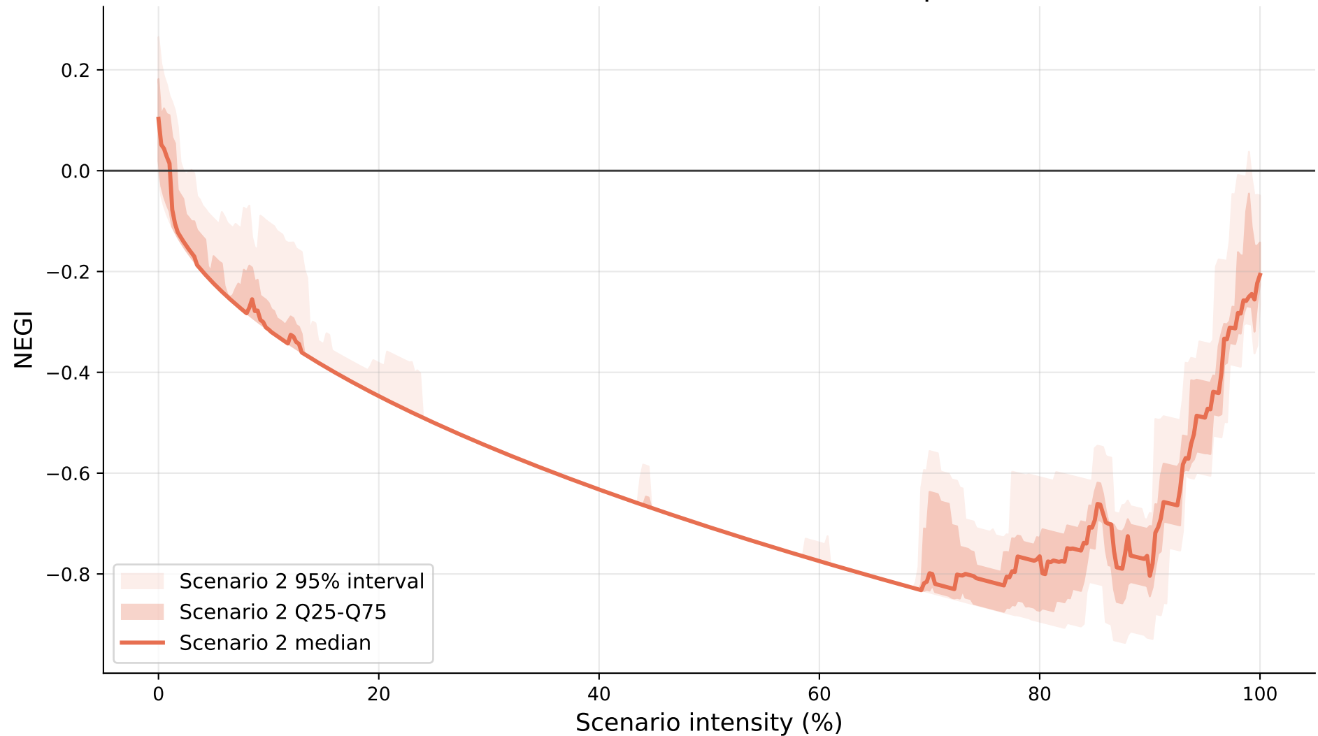
Scenario 2 NEGI Robustness Across 10 Spatial Refits
