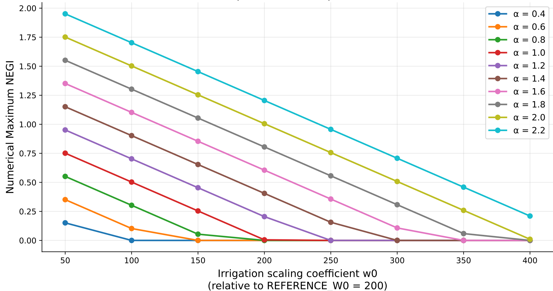
Supplementary Diagnostic: Sensitivity of Numerical Maximum NEGI (exponent = 0.5, \beta = 1.0 )
