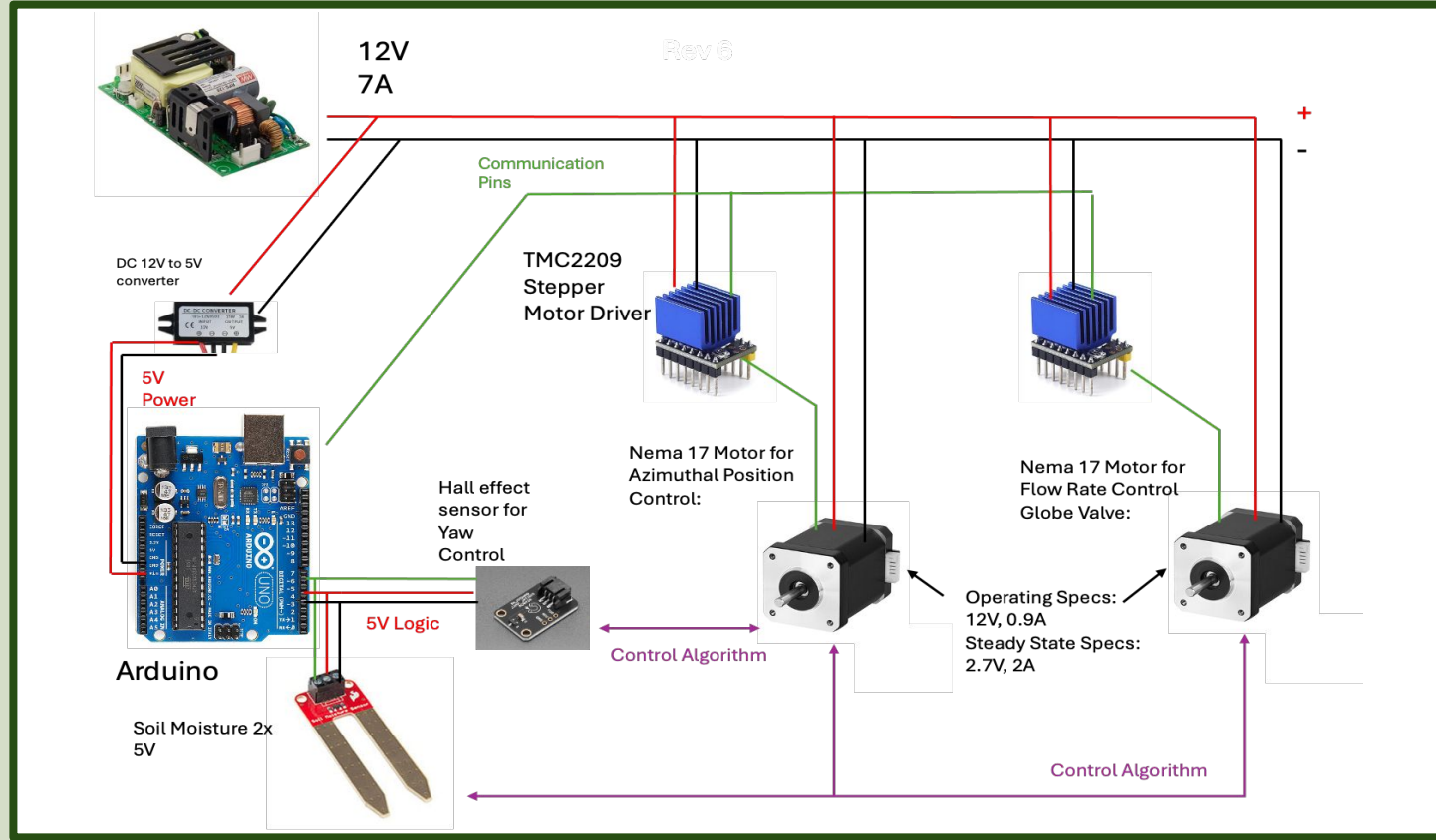
Electrical System Diagram
