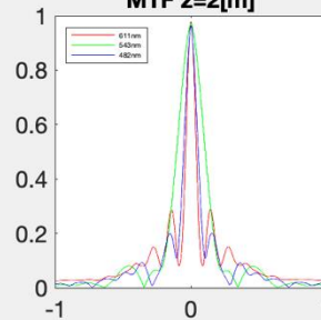
MTF z=2[m]
