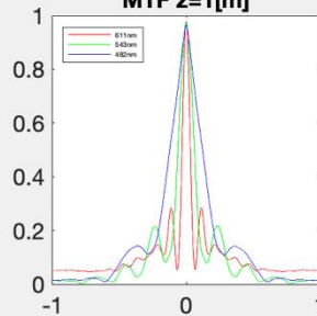
MTF z=1[m]
