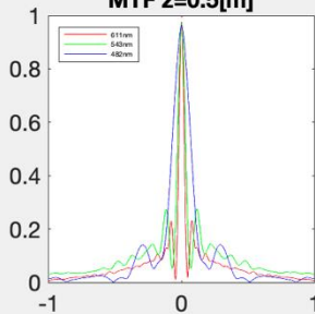
MTF z=0.5[m]
