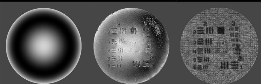
A Zernike Primary spherical
