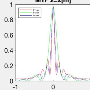
MTF z=2[m]
