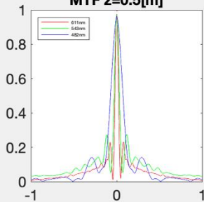
MTF z=0.5[m]
