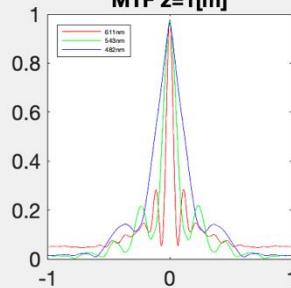
MTF z=1[m]
