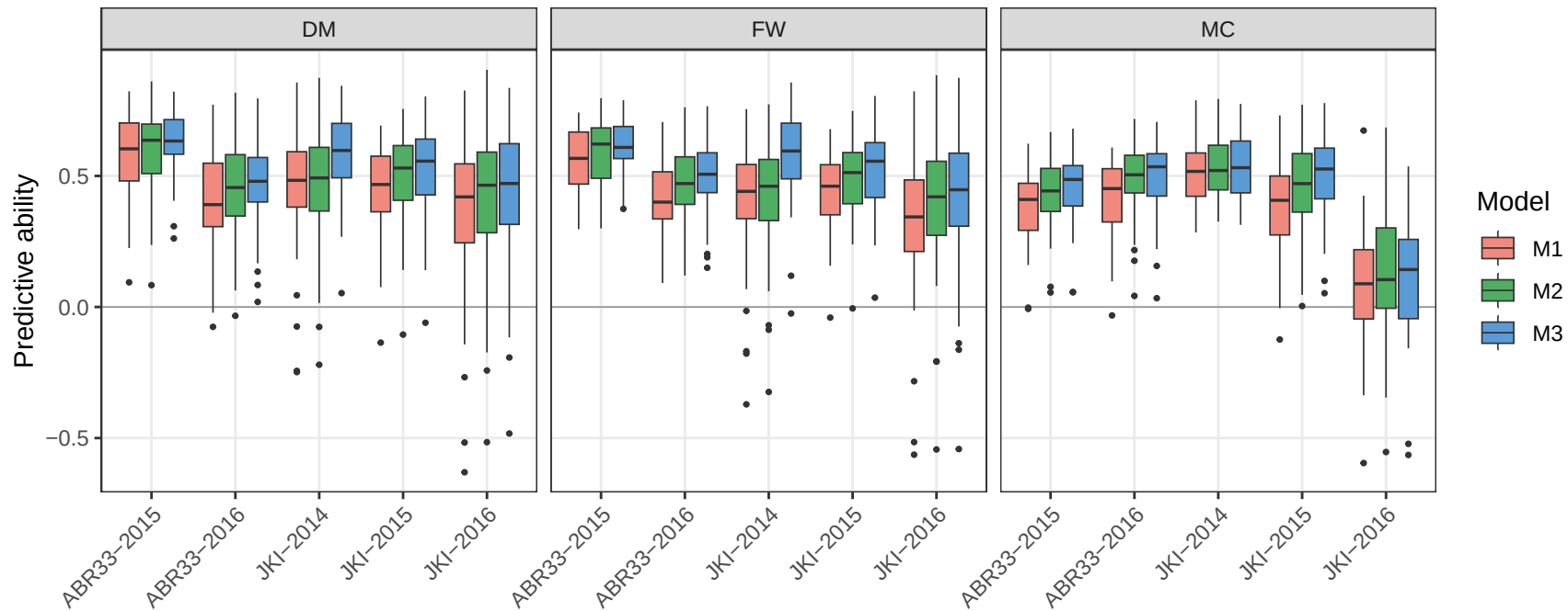
CV1 – population group fitted as a fixed effect
