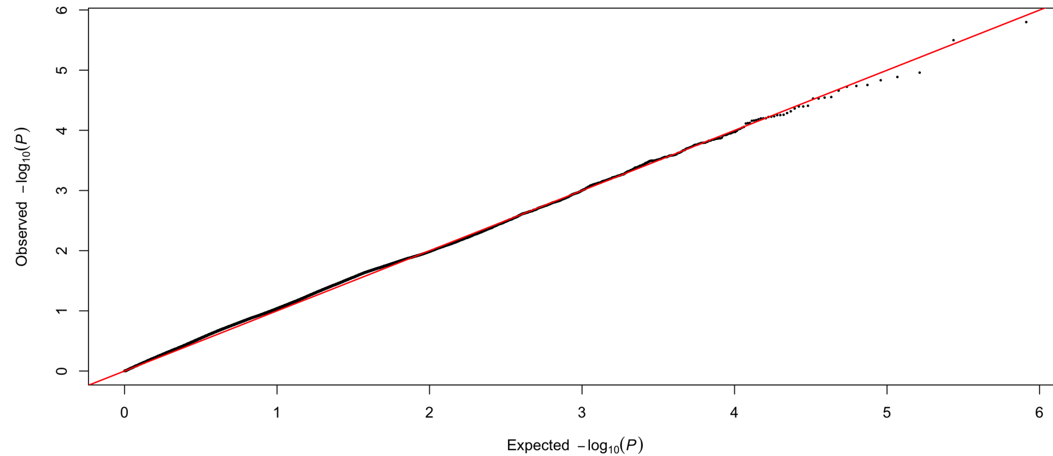
PPP CV1 partition 1 fold 1: Q-Q
