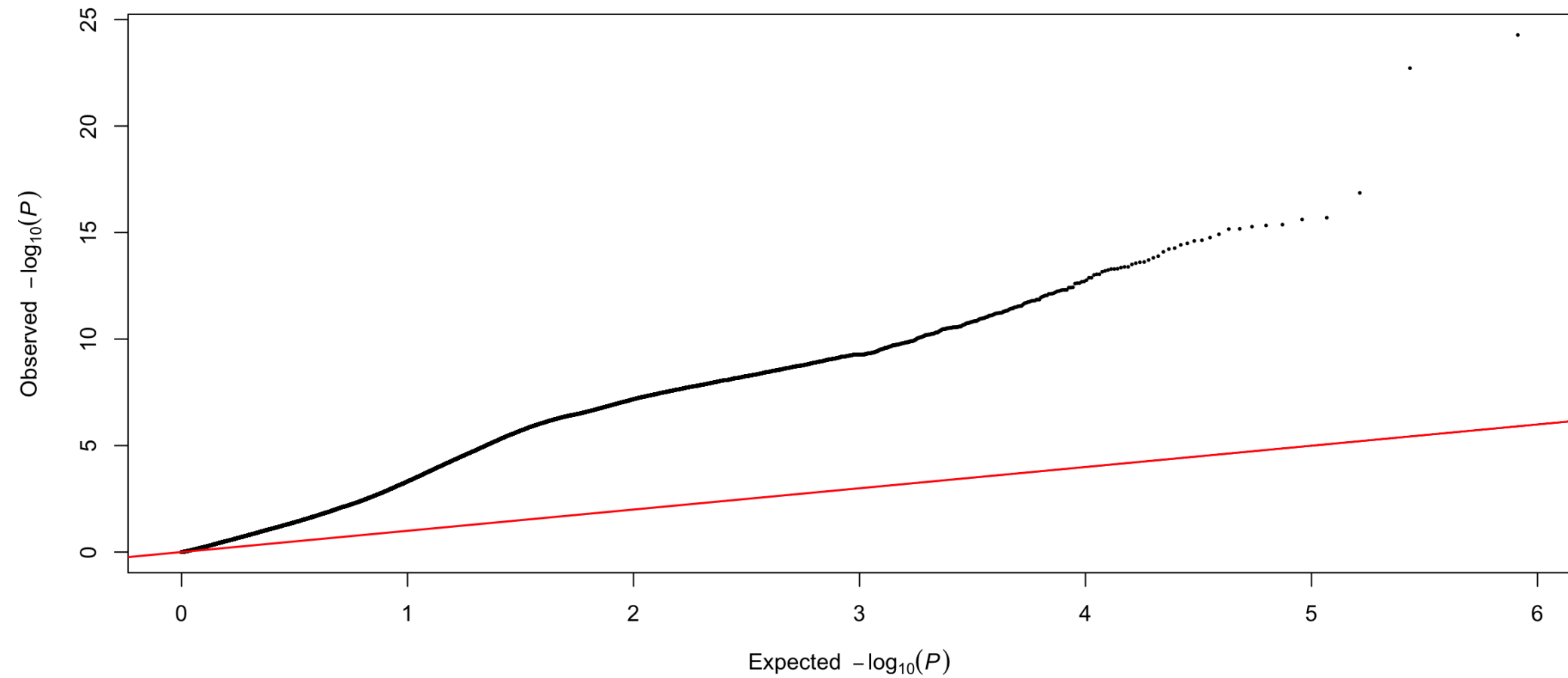
DTF CV1 partition 1 fold 1: Q-Q
