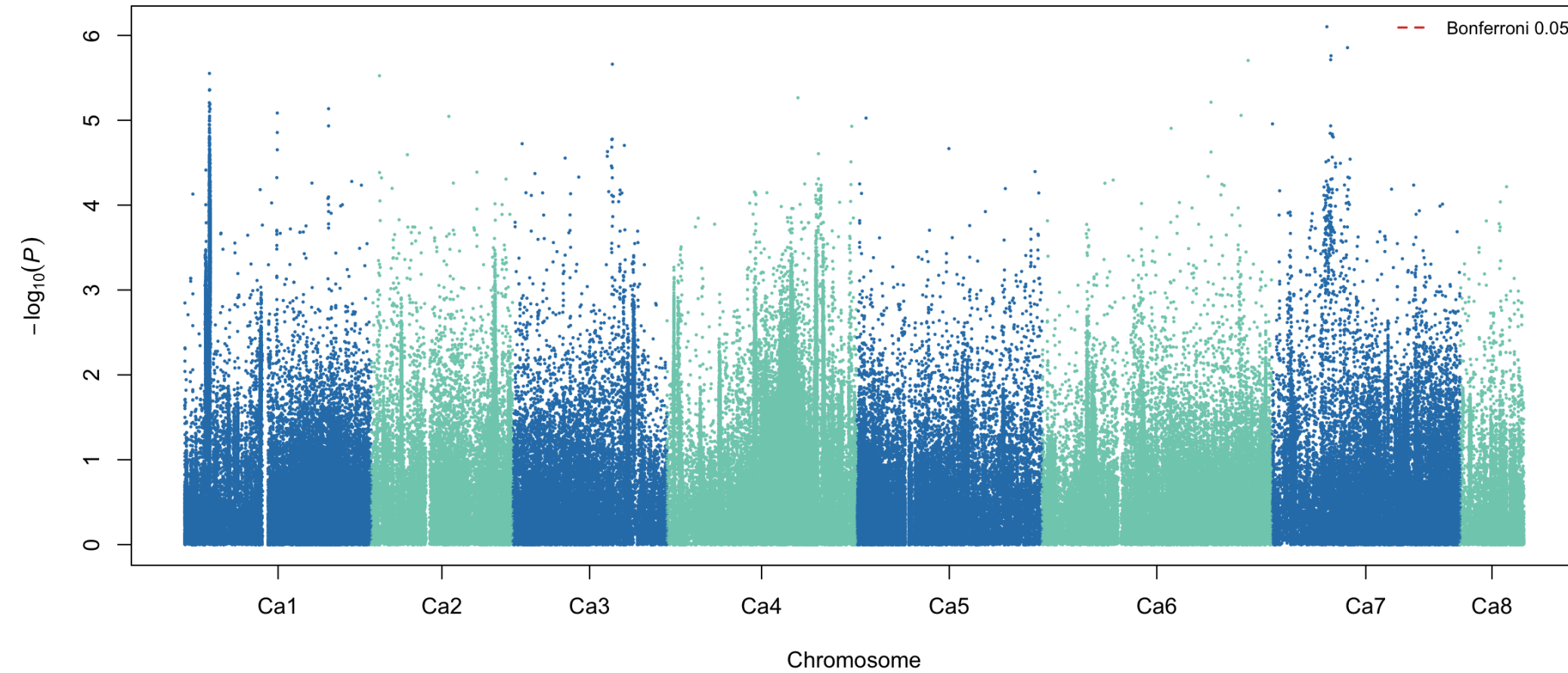
YPP CV2 partition 1 fold 1: meta-GWAS
