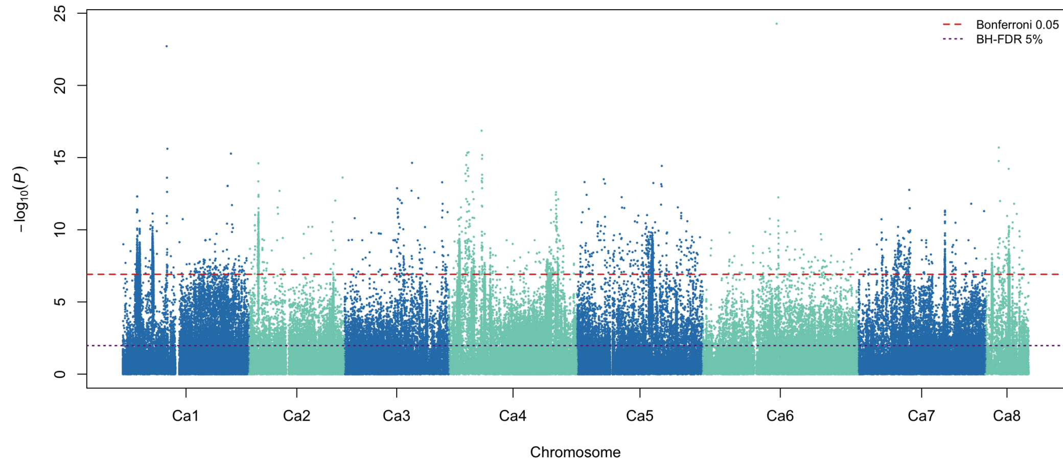
DTF CV1 partition 1 fold 1: meta-GWAS
