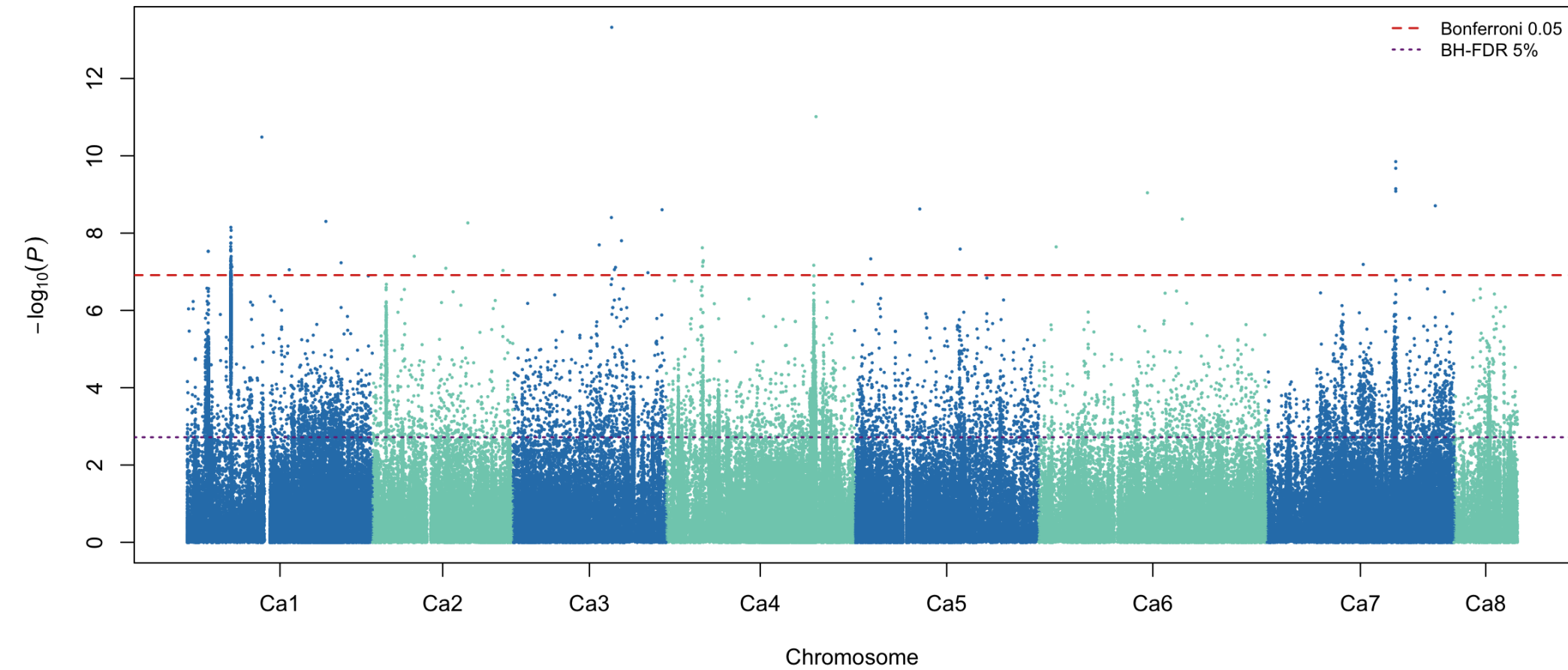
DTM CV00 partition 1 fold 1: meta-GWAS
