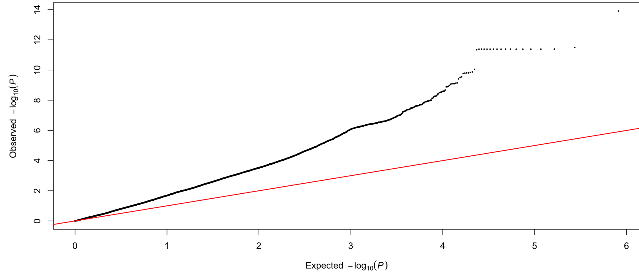
PH CV1 partition 1 fold 1: Q-Q
