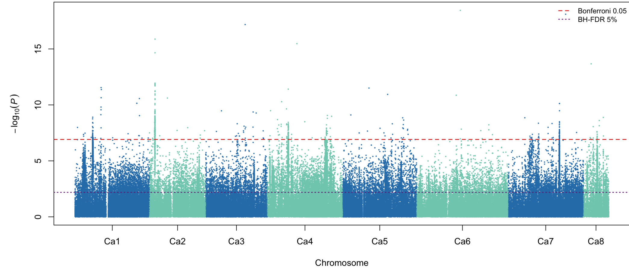
DTF CV0 partition 1 fold 1: meta-GWAS
