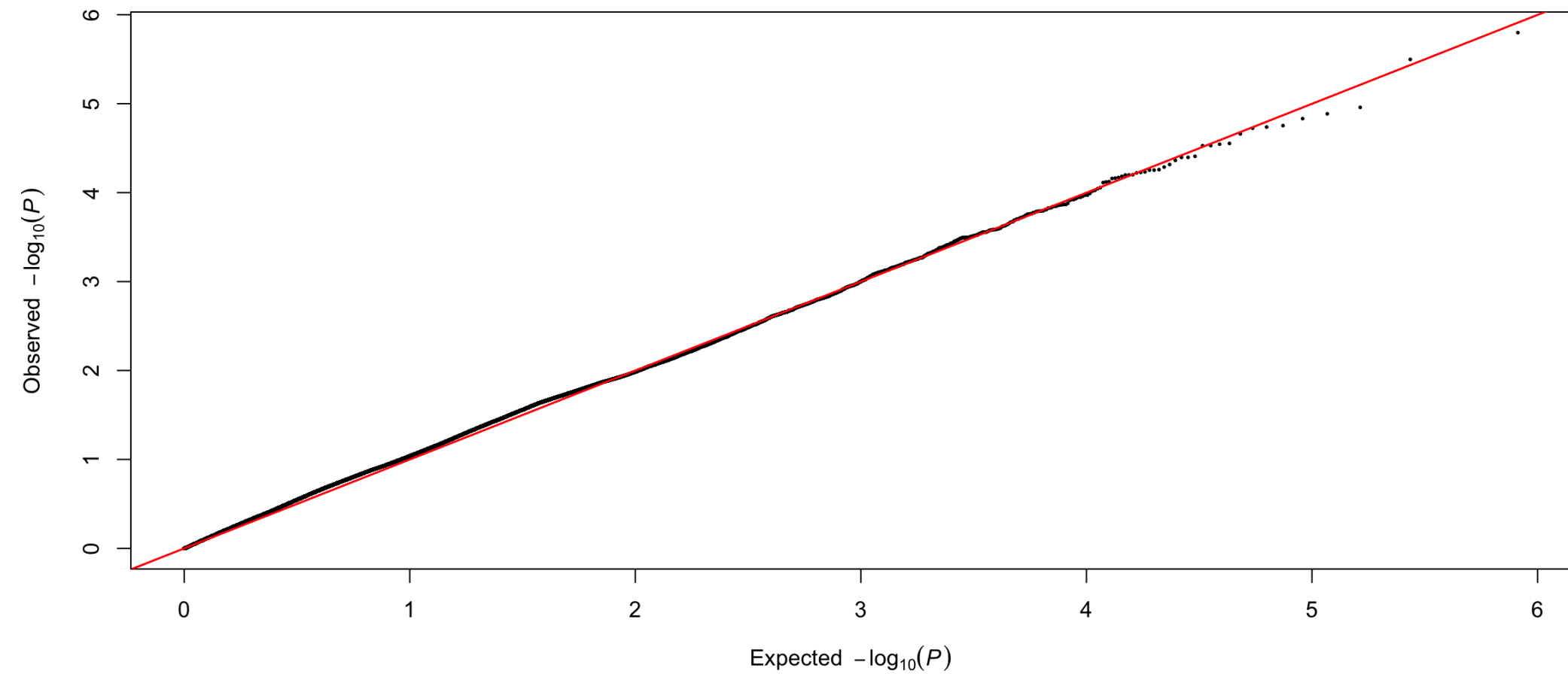
PPP CV1 partition 1 fold 1: Q-Q
