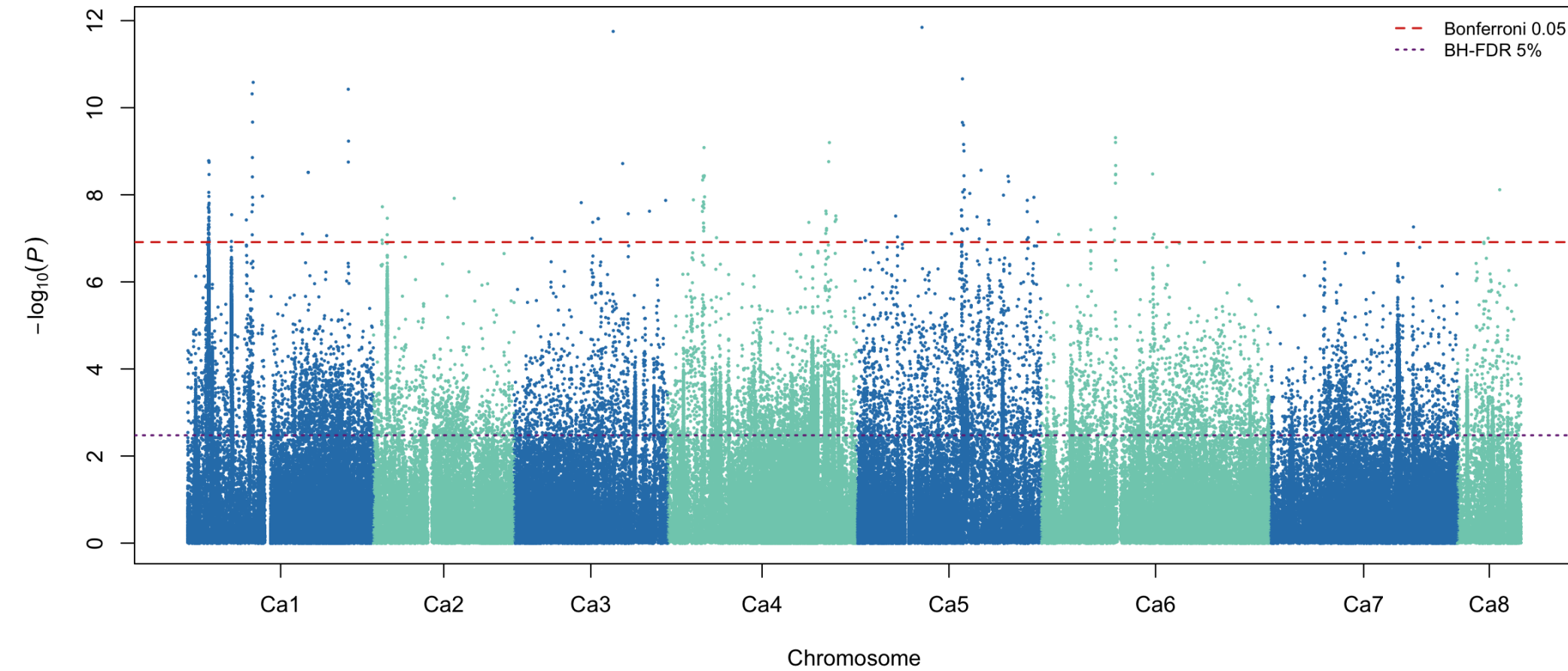
DTM CV2 partition 1 fold 1: meta-GWAS
