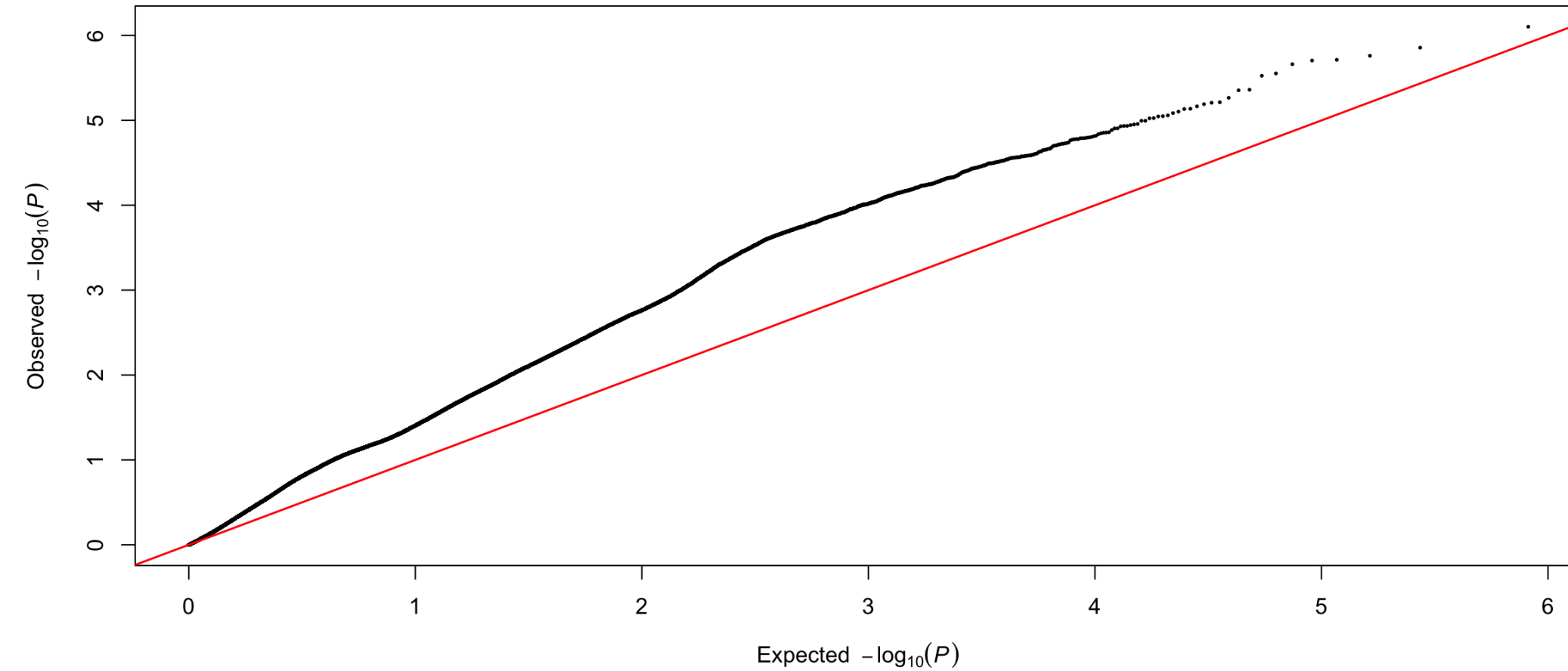
YPP CV2 partition 1 fold 1: Q-Q
