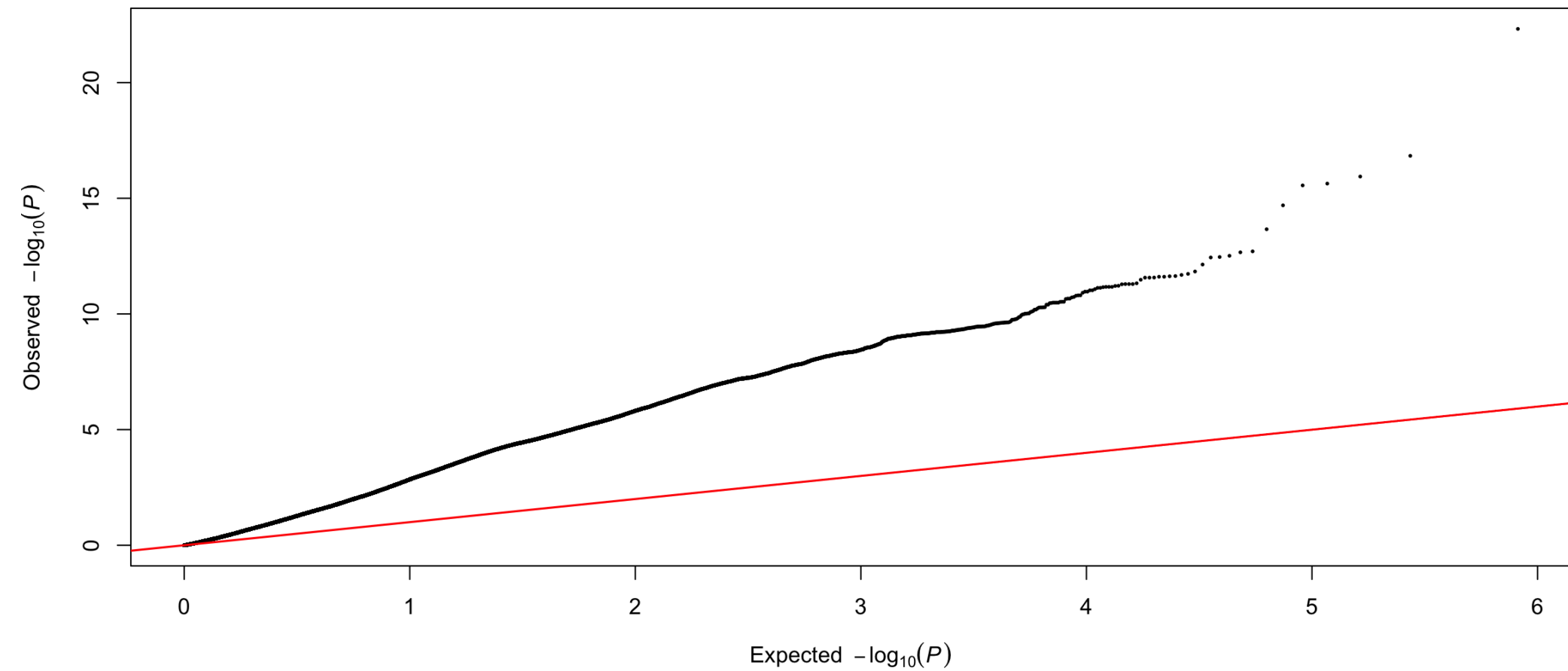
DTF CV00 partition 1 fold 1: Q-Q
