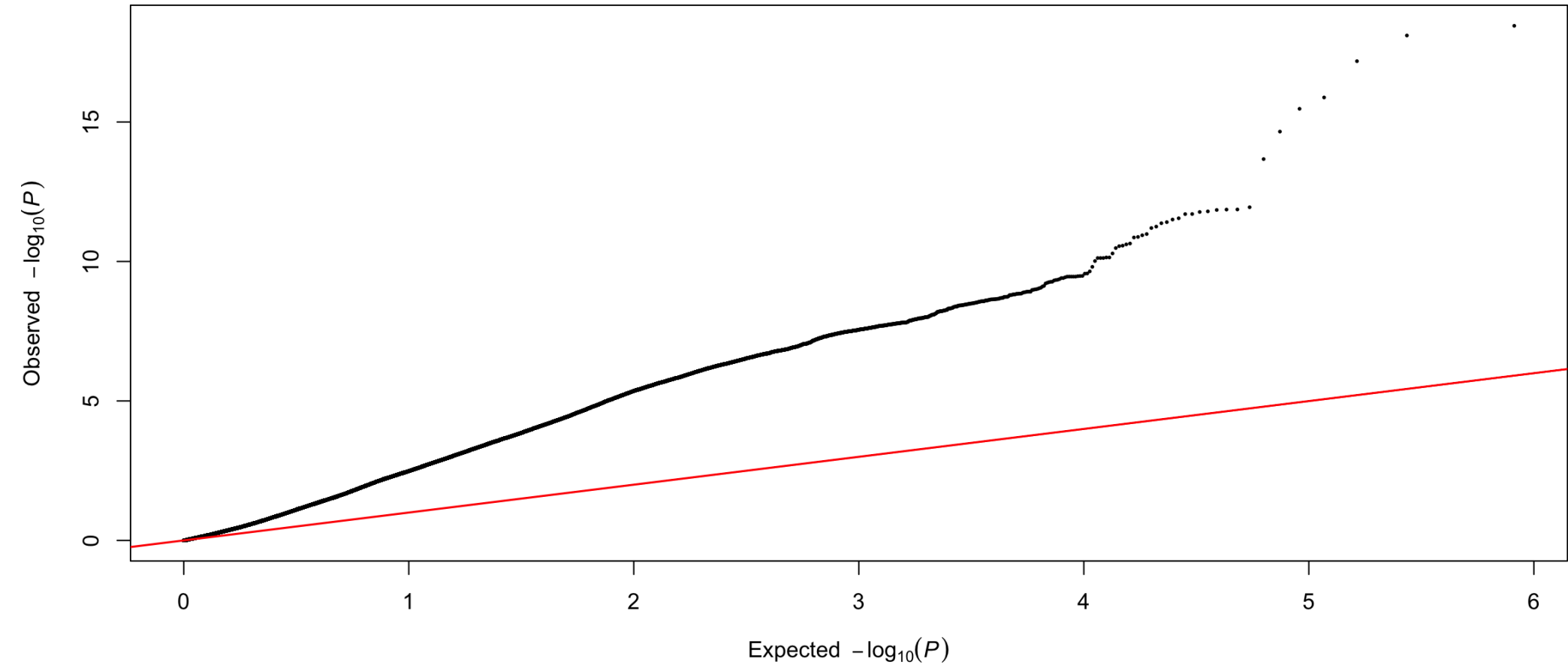
DTF CV0 partition 1 fold 1: Q-Q
