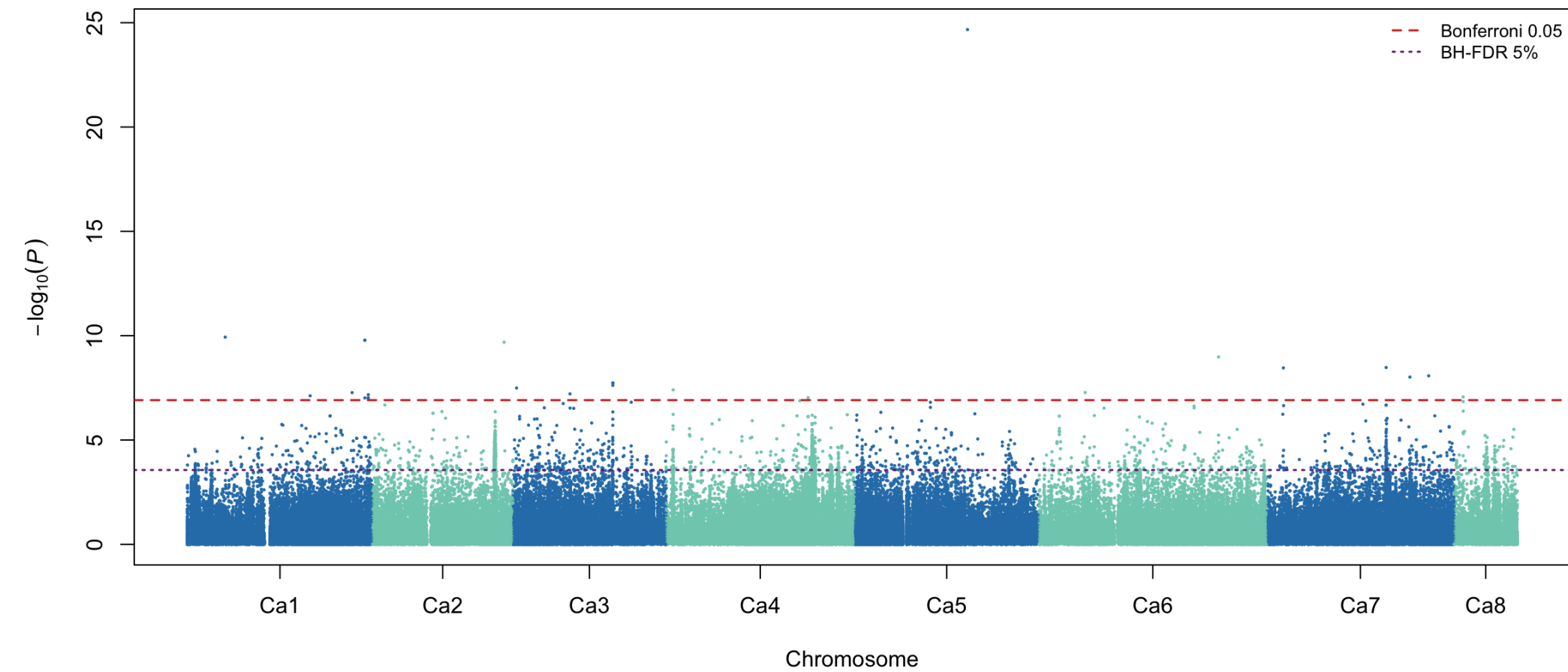
PH CV00 partition 1 fold 1: meta-GWAS
