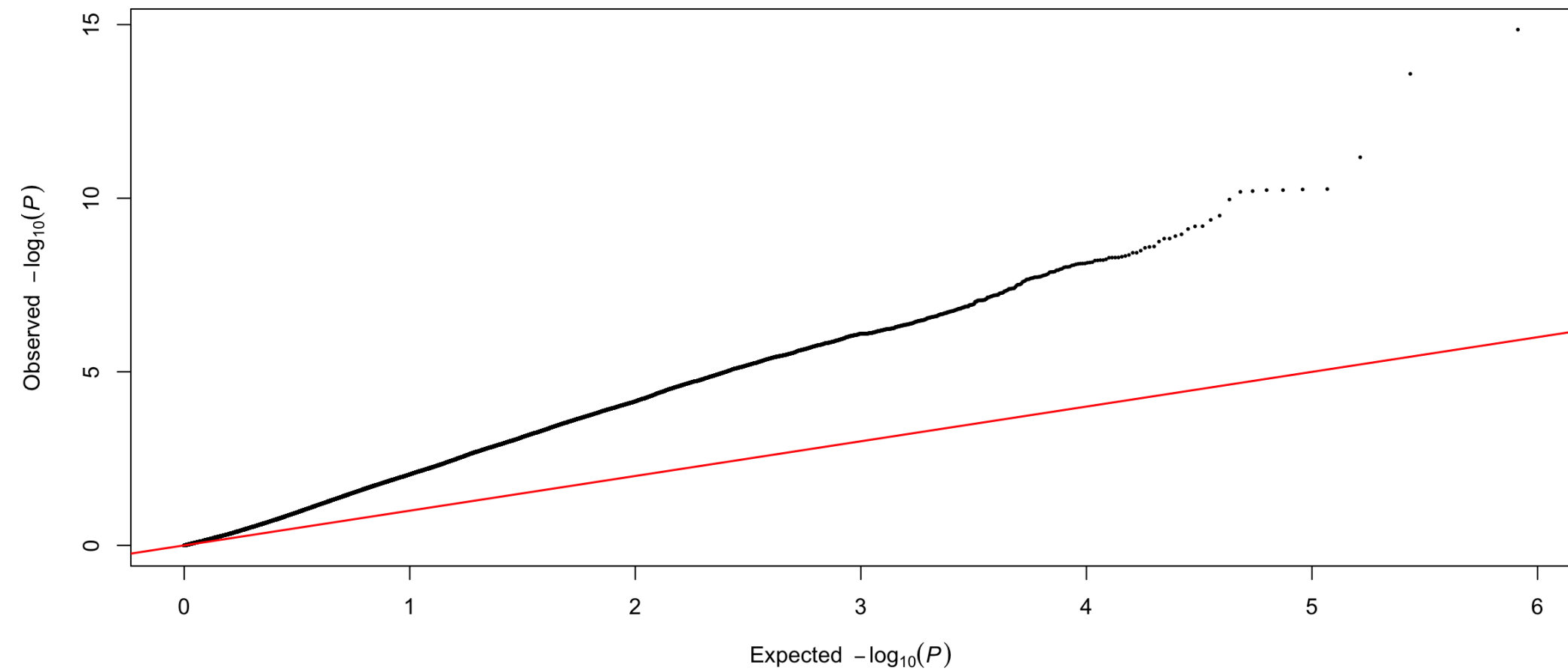
DTM CV0 partition 1 fold 1: Q-Q
