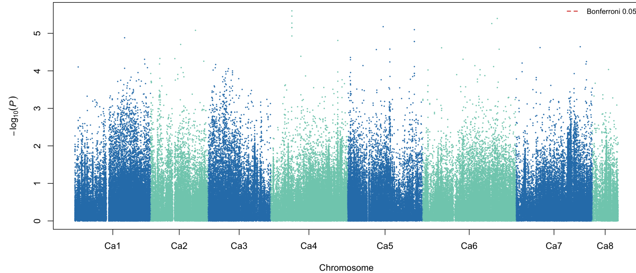
PPP CV2 partition 1 fold 1: meta-GWAS
