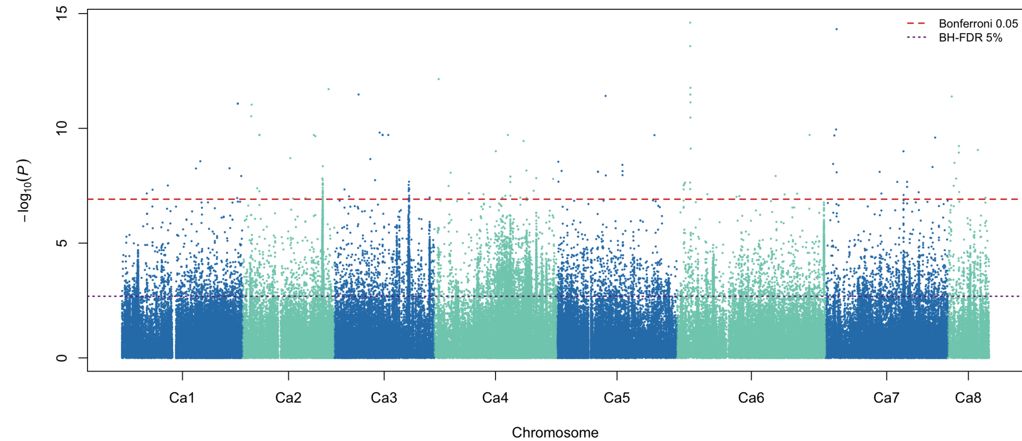
PH CV0 partition 1 fold 1: meta-GWAS
