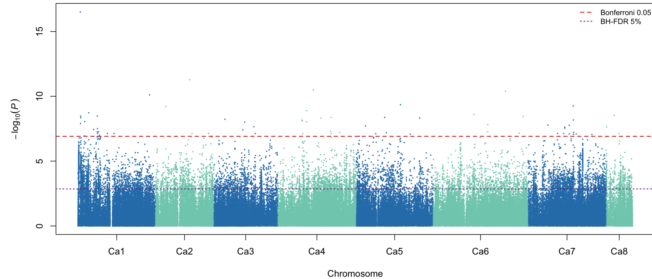
HSW CV00 partition 1 fold 1: meta-GWAS
