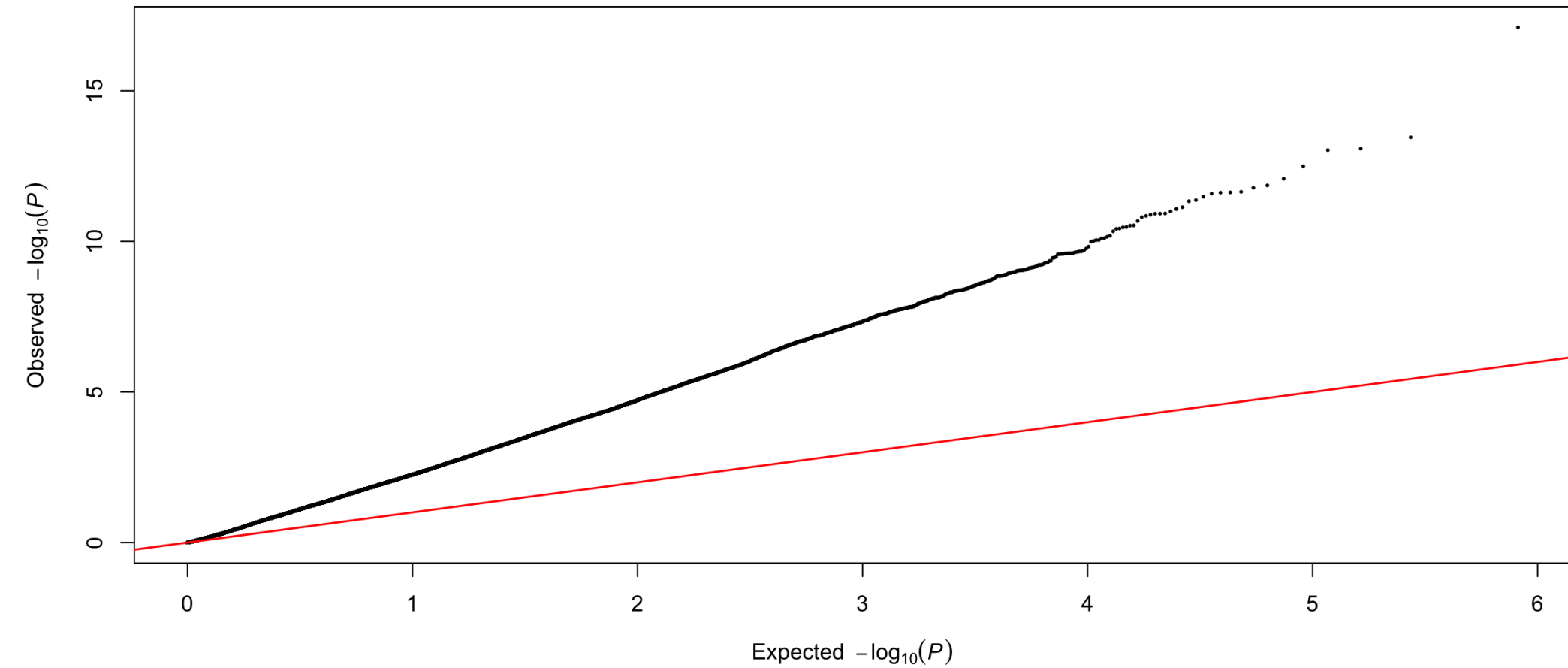
HSW CV1 partition 1 fold 1: Q-Q
