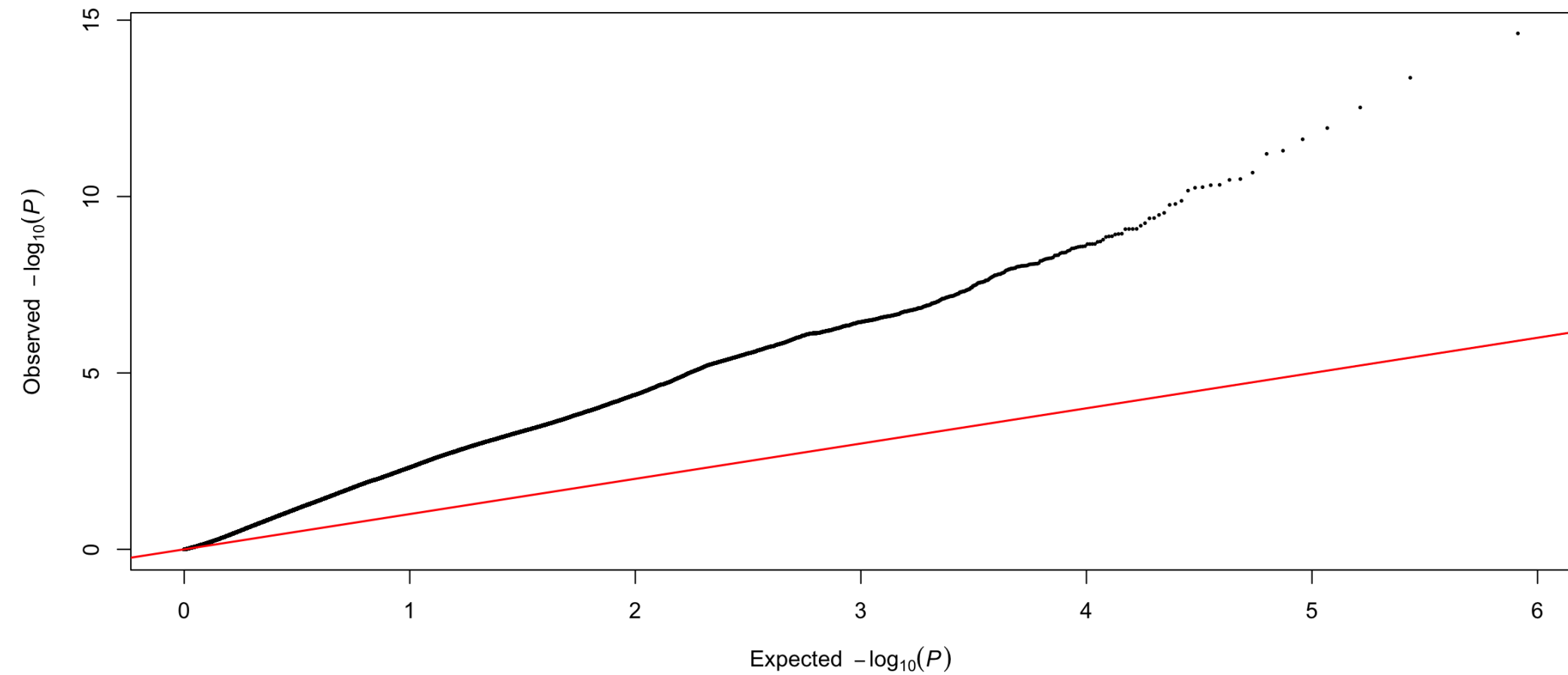
DTM CV1 partition 1 fold 1: Q-Q
