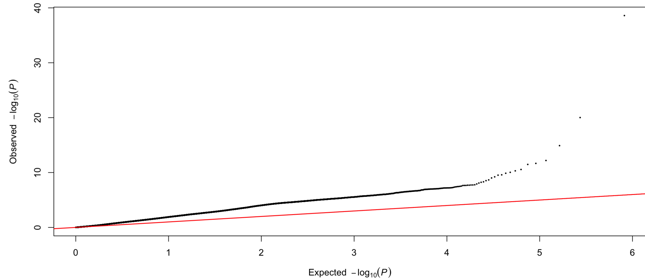
HSW CV0 partition 1 fold 1: Q-Q
