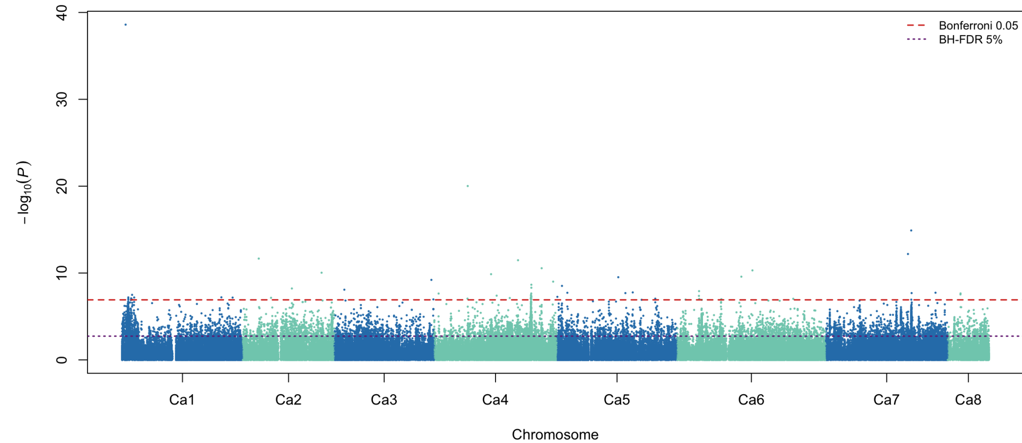
HSW CV0 partition 1 fold 1: meta-GWAS
