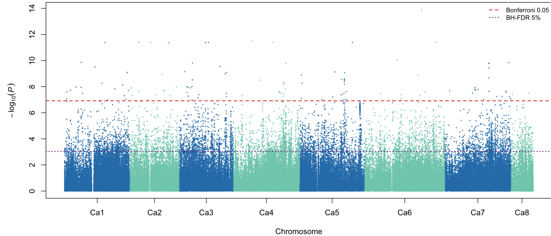
PH CV1 partition 1 fold 1: meta-GWAS
