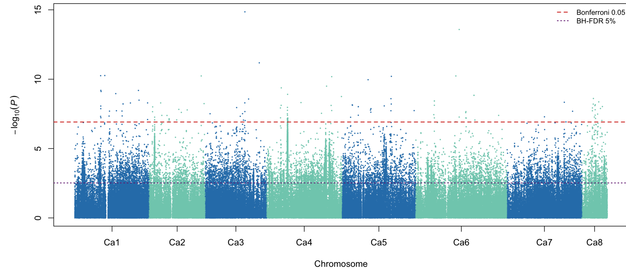
DTM CV0 partition 1 fold 1: meta-GWAS
