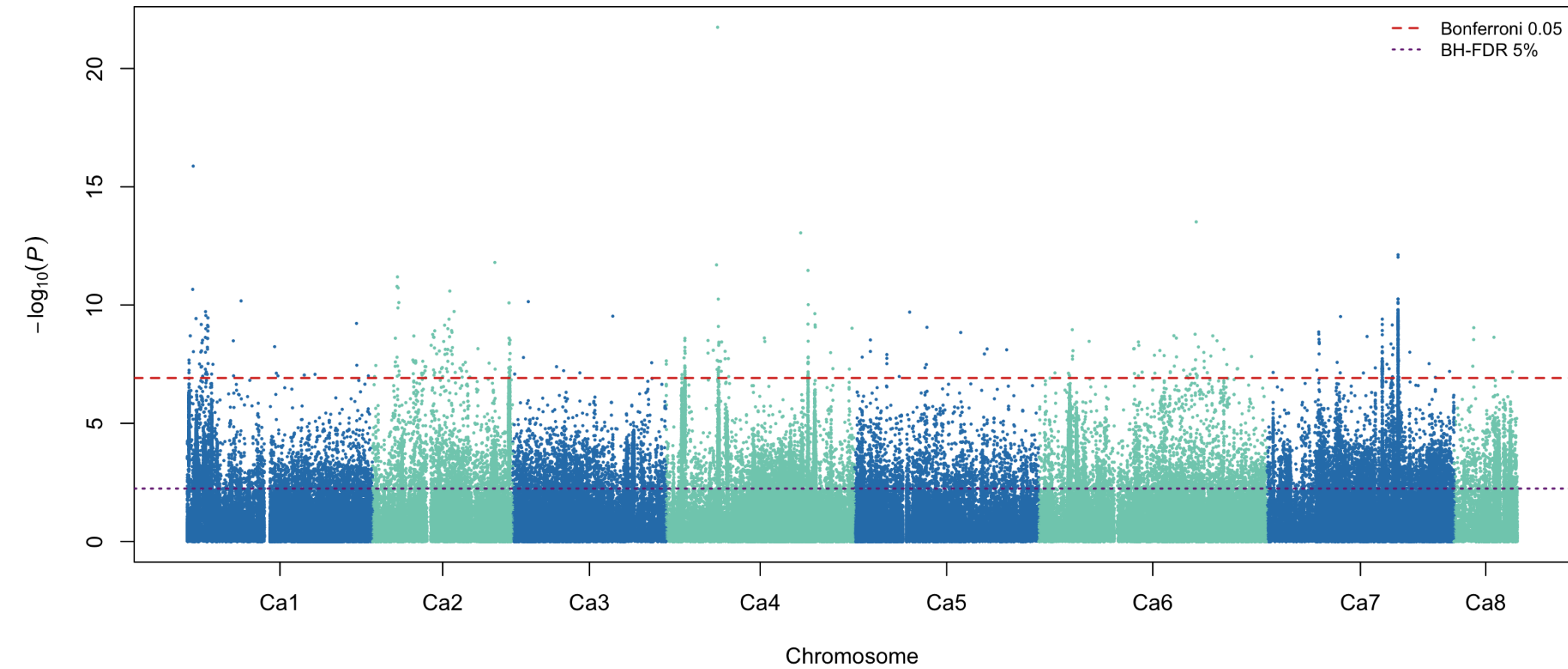
HSW CV2 partition 1 fold 1: meta-GWAS
