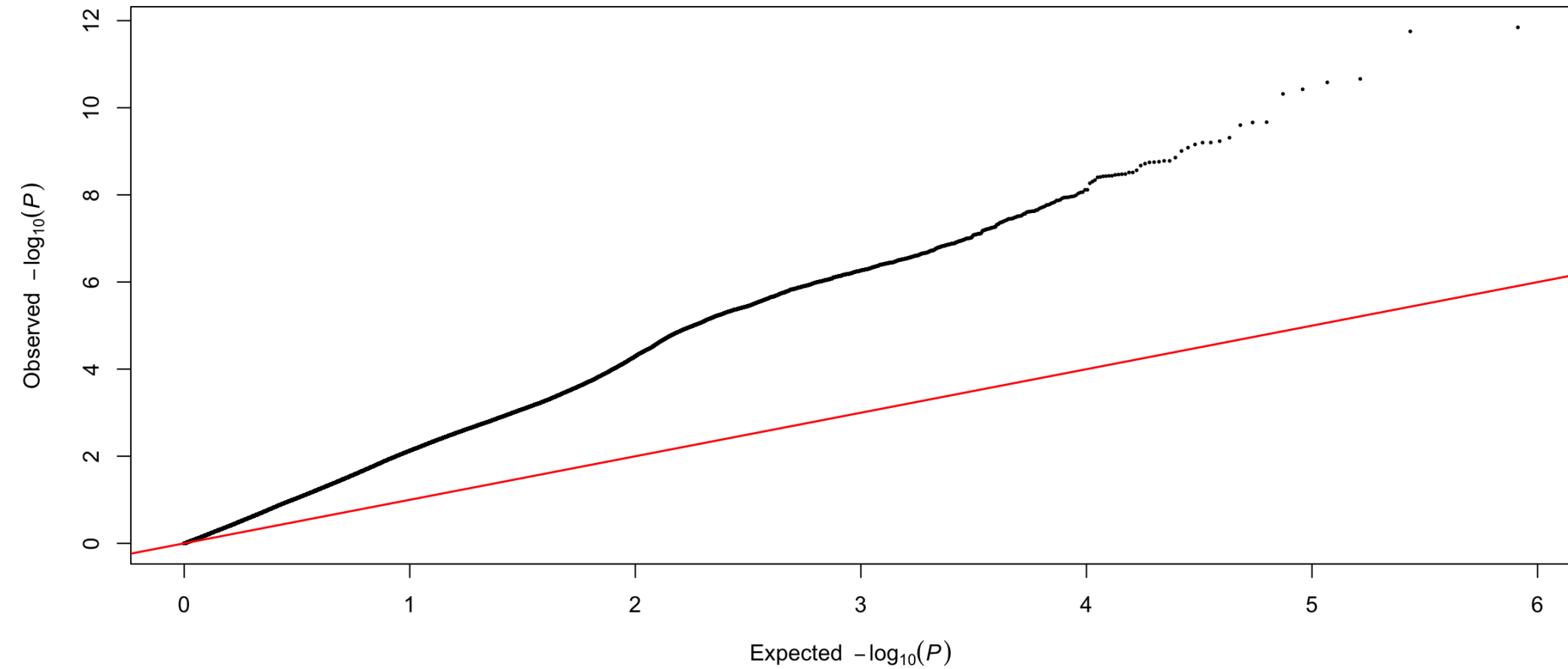
DTM CV2 partition 1 fold 1: Q-Q
