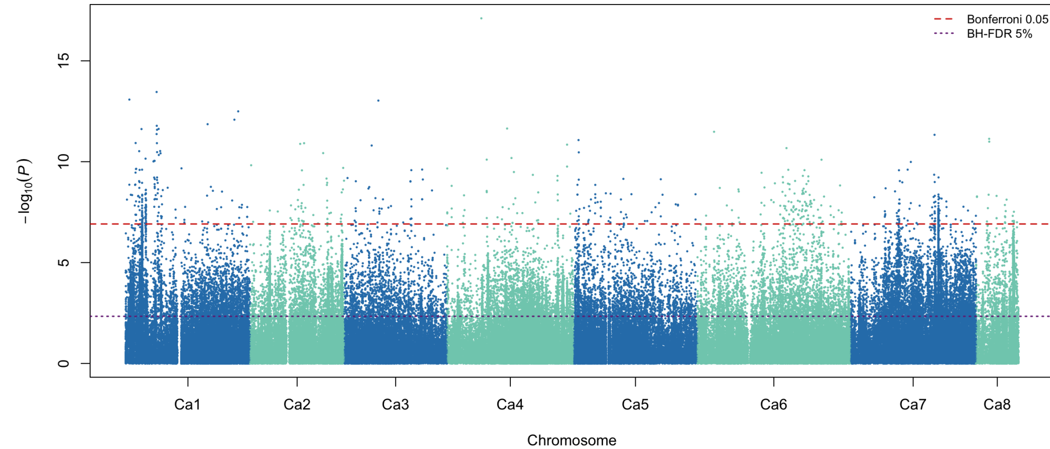
HSW CV1 partition 1 fold 1: meta-GWAS
