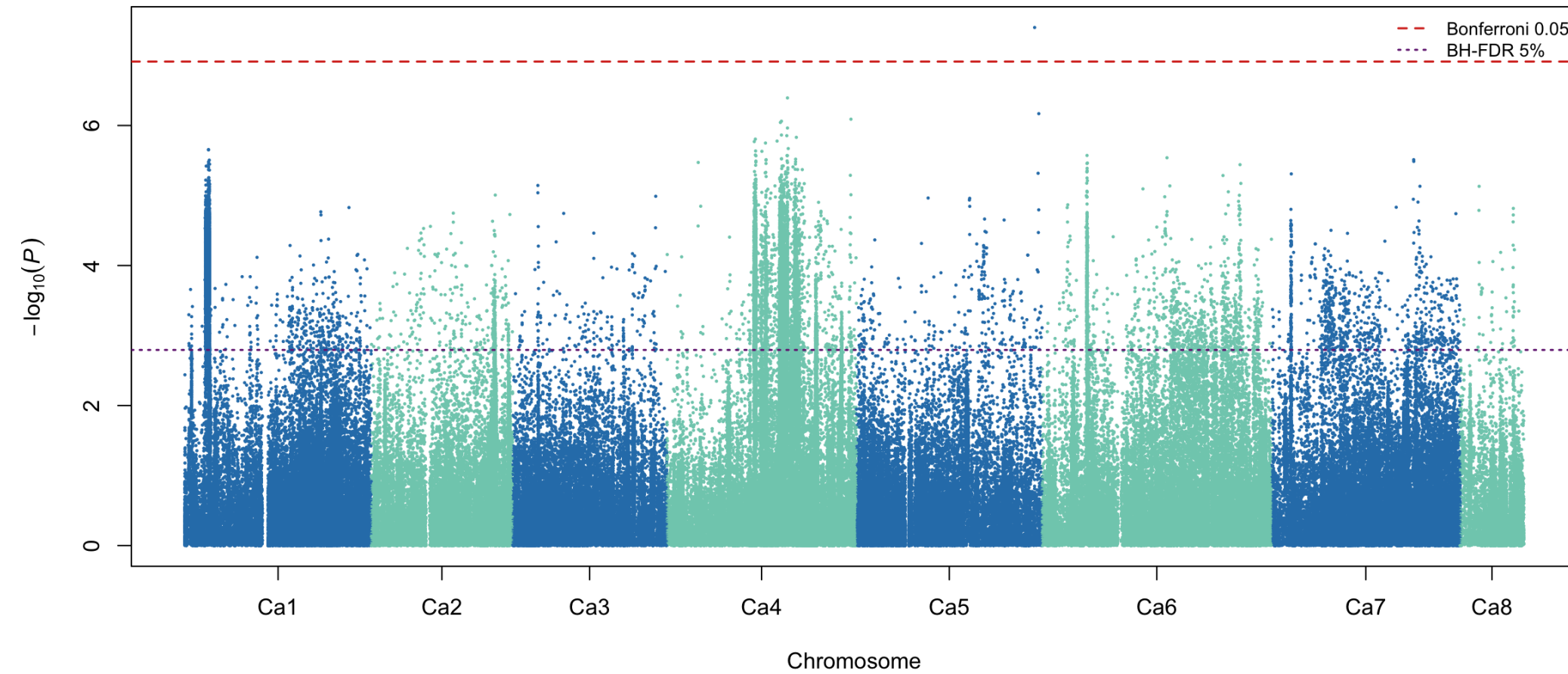
YPP CV1 partition 1 fold 1: meta-GWAS
