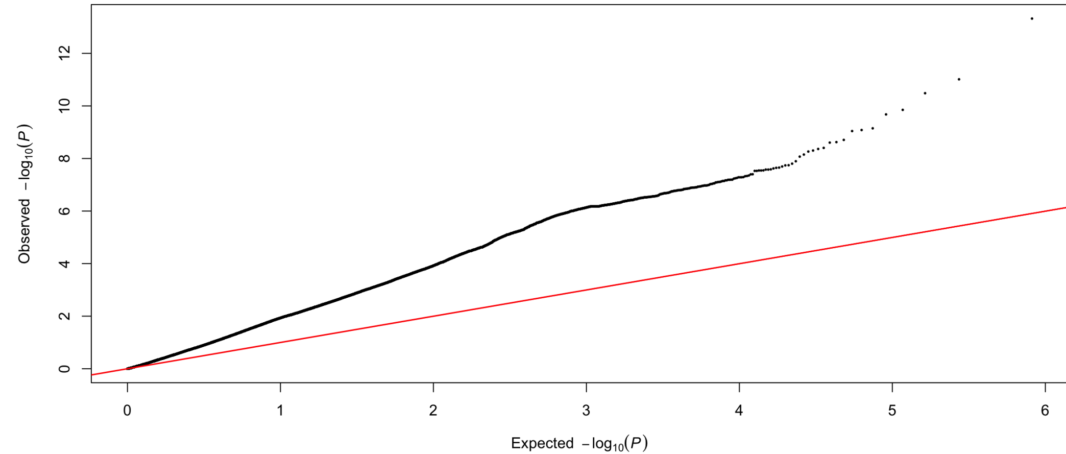
DTM CV00 partition 1 fold 1: Q-Q
