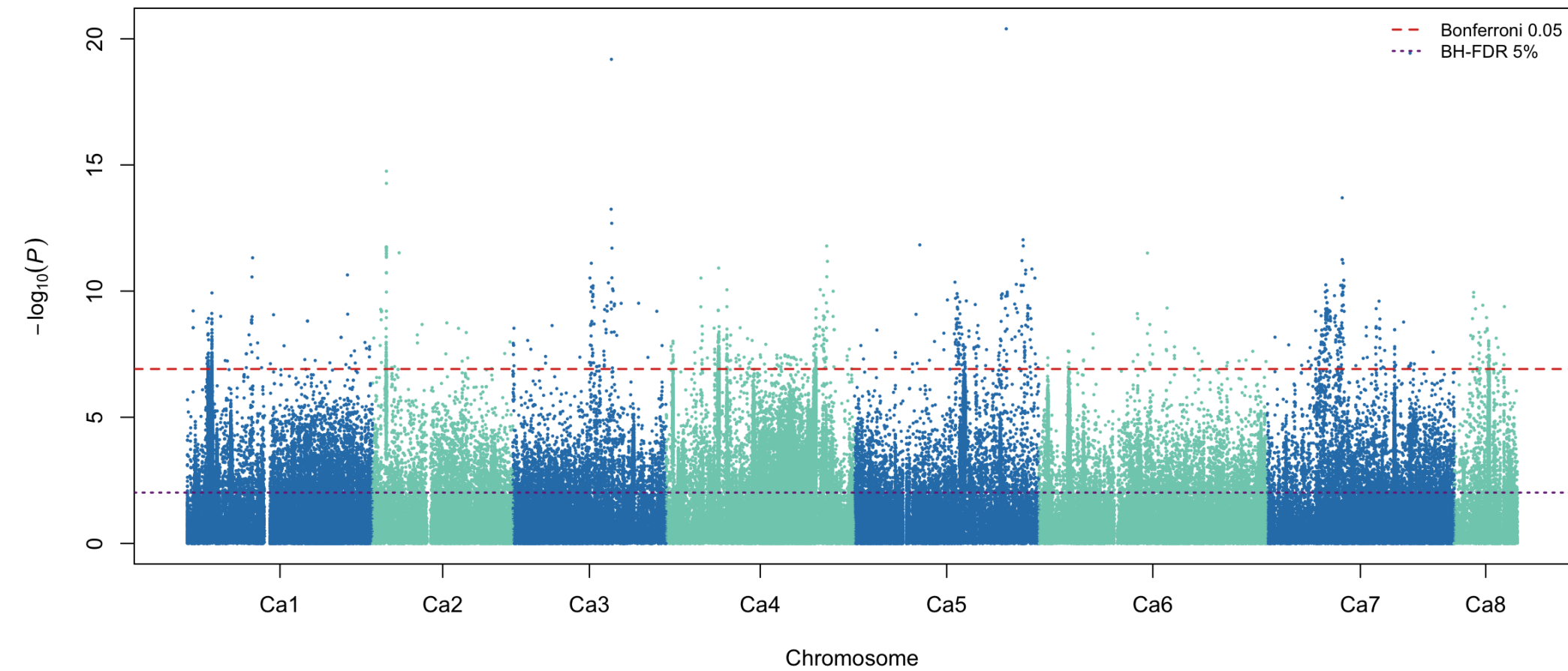
DTF CV2 partition 1 fold 1: meta-GWAS
