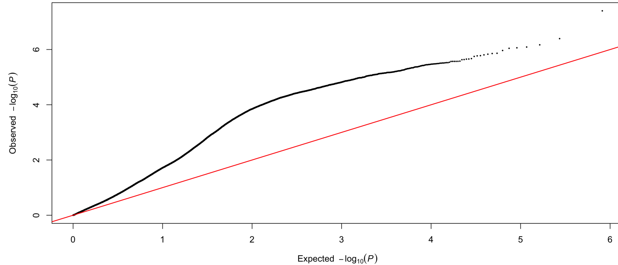
YPP CV1 partition 1 fold 1: Q-Q
