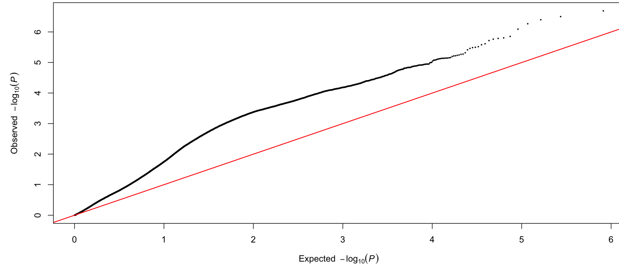
YPP CV00 partition 1 fold 1: Q-Q
