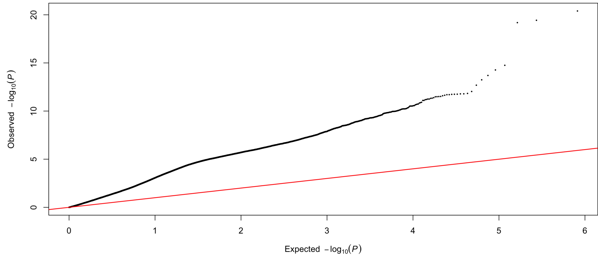
DTF CV2 partition 1 fold 1: Q-Q
