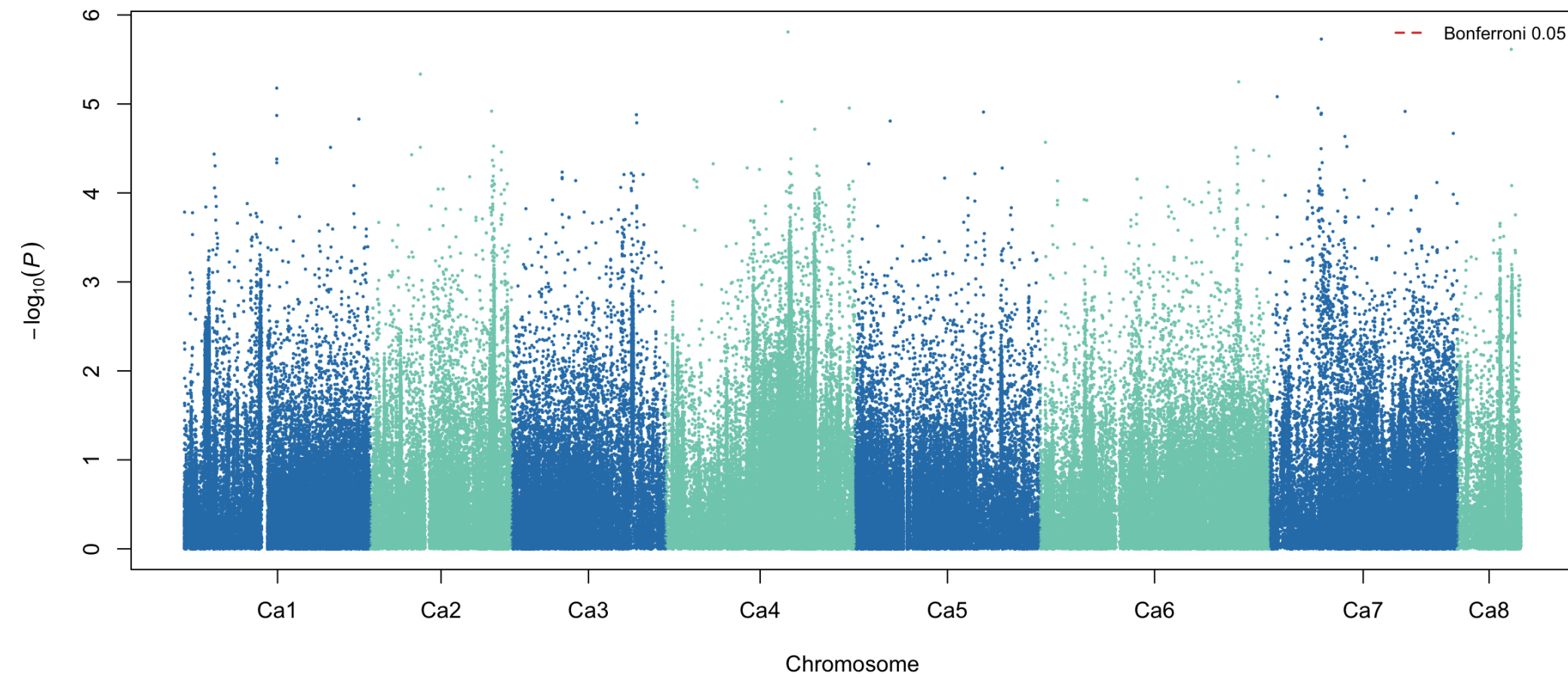
YPP CV0 partition 1 fold 1: meta-GWAS
