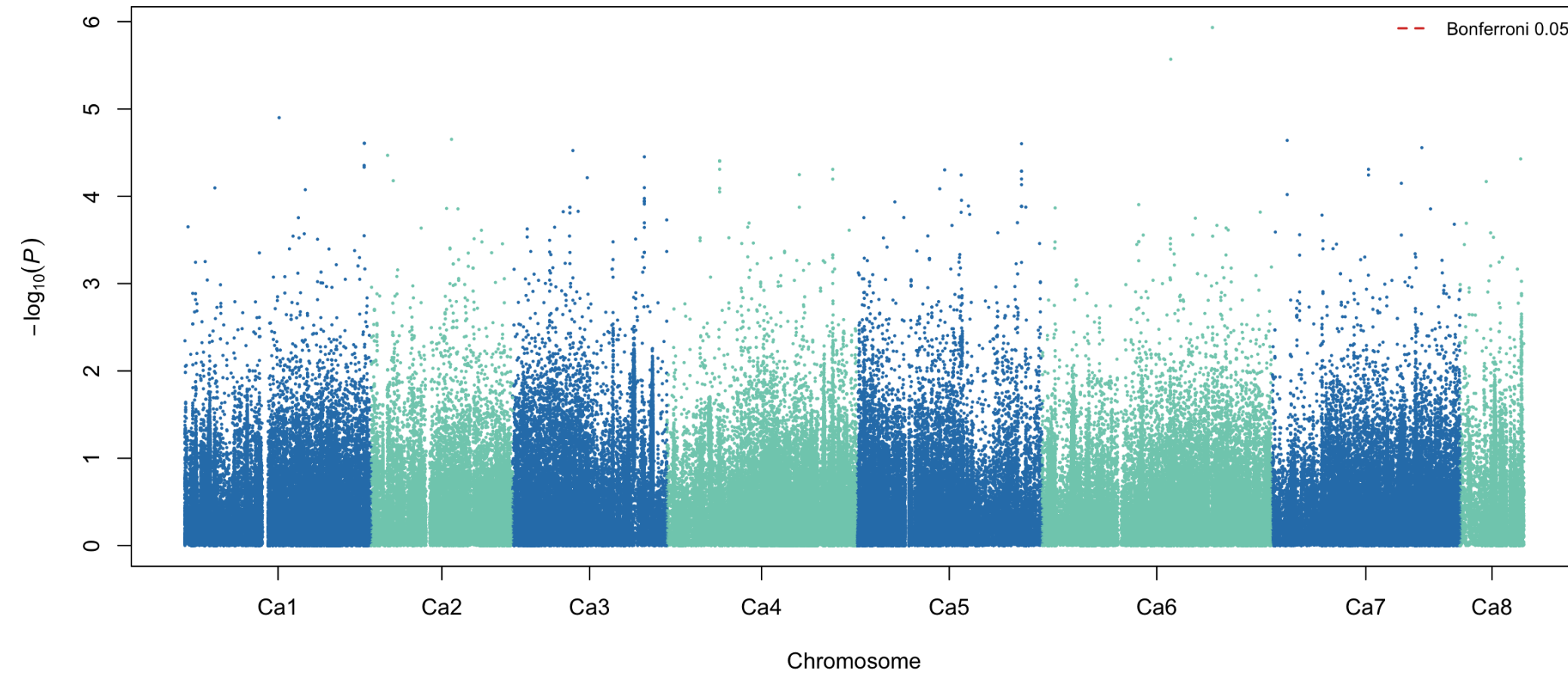
PPP CV0 partition 1 fold 1: meta-GWAS
