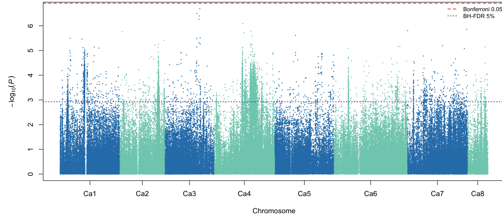
YPP CV00 partition 1 fold 1: meta-GWAS
