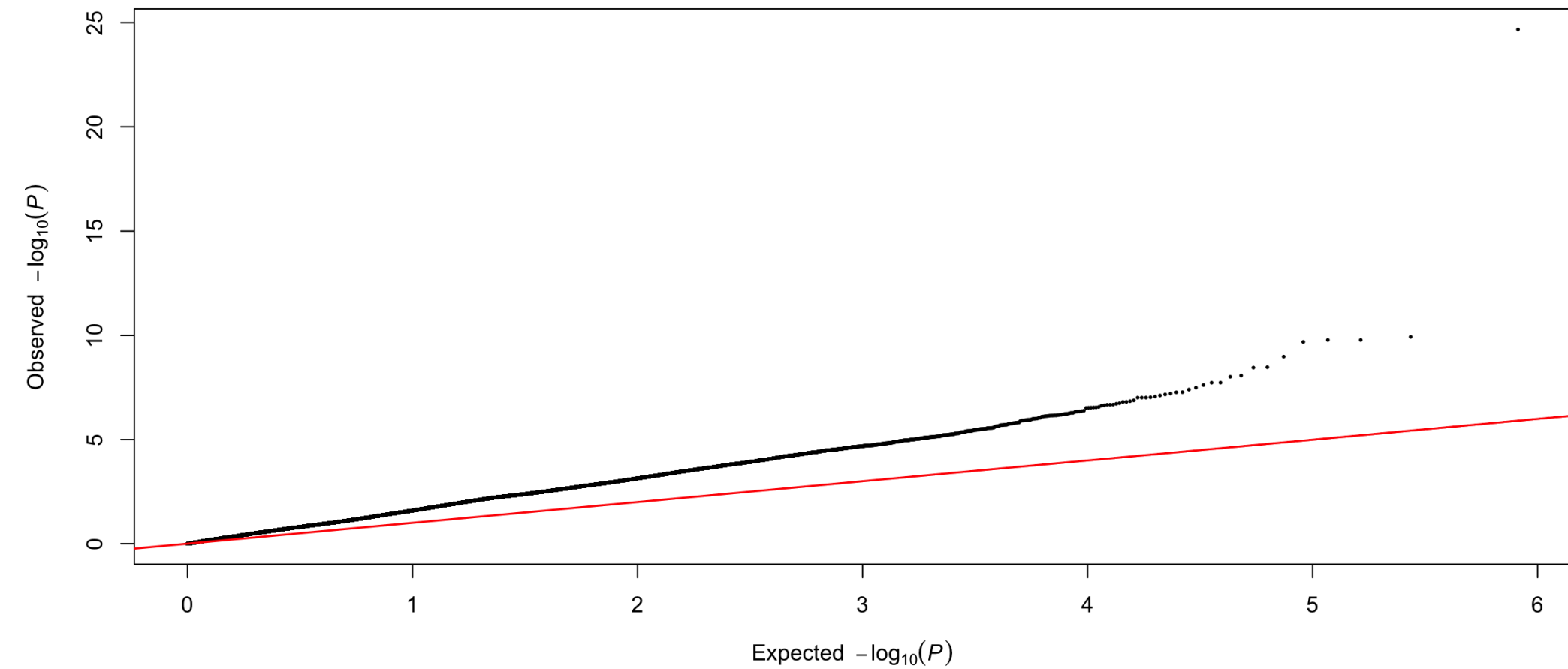
PH CV00 partition 1 fold 1: Q-Q
