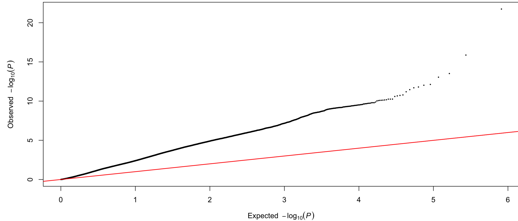
HSW CV2 partition 1 fold 1: Q-Q
