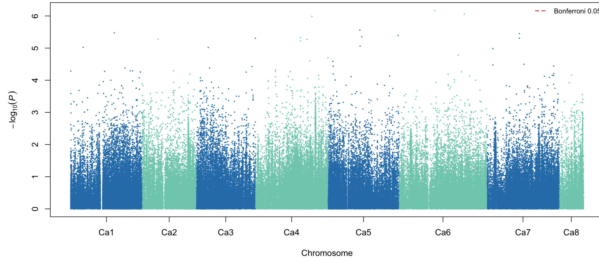
PPP CV00 partition 1 fold 1: meta-GWAS
