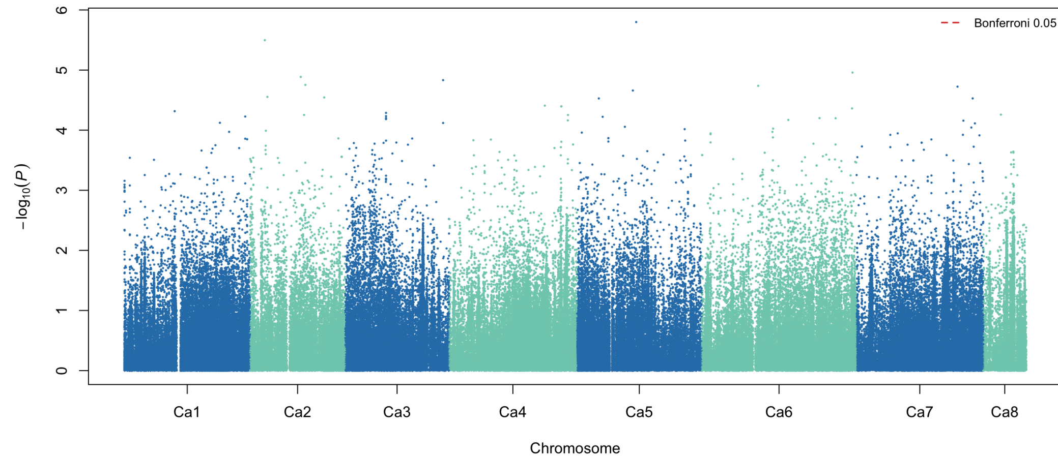
PPP CV1 partition 1 fold 1: meta-GWAS
