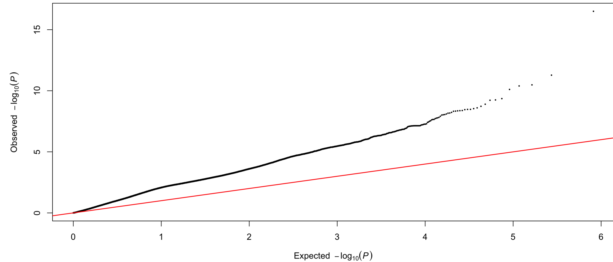
HSW CV00 partition 1 fold 1: Q-Q
