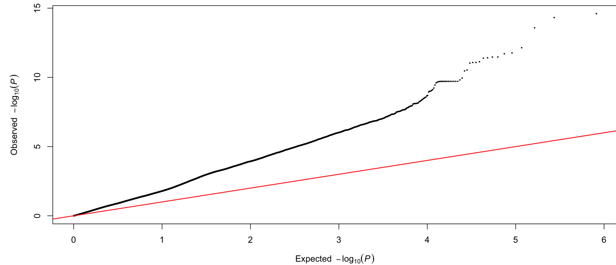
PH CV0 partition 1 fold 1: Q-Q
