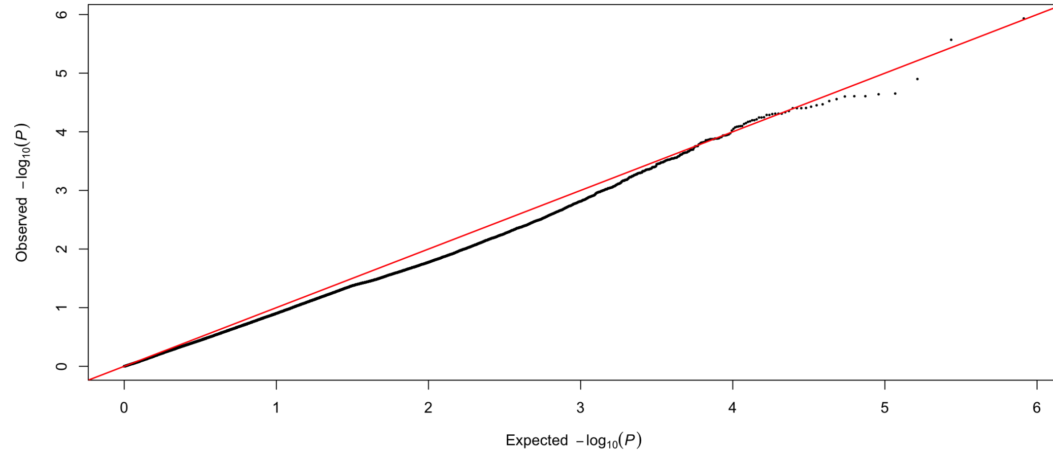
PPP CV0 partition 1 fold 1: Q-Q
