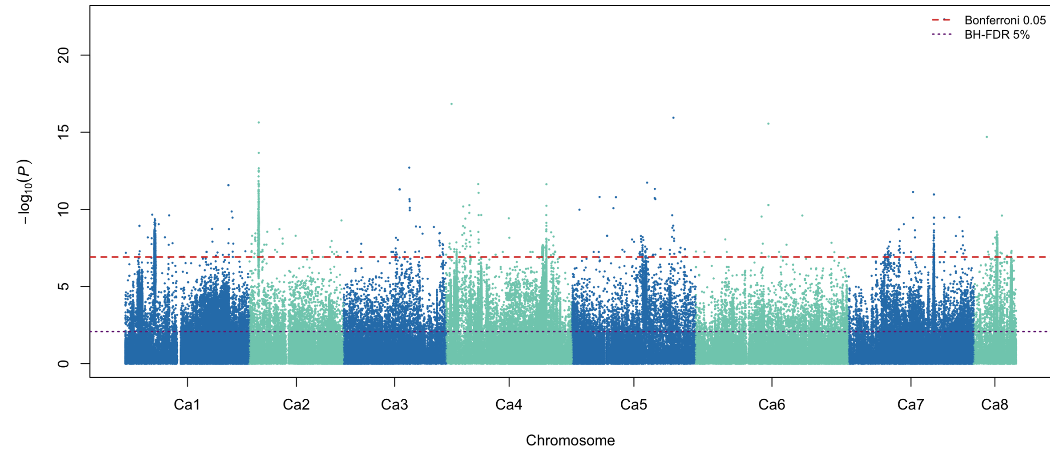
DTF CV00 partition 1 fold 1: meta-GWAS
