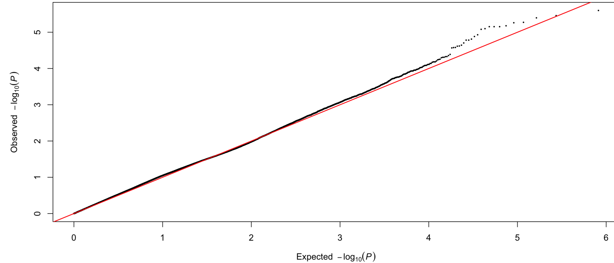
PPP CV2 partition 1 fold 1: Q-Q
