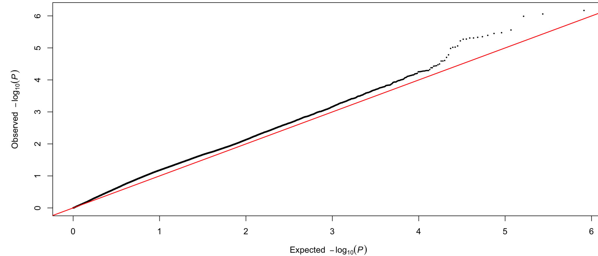
PPP CV00 partition 1 fold 1: Q-Q
