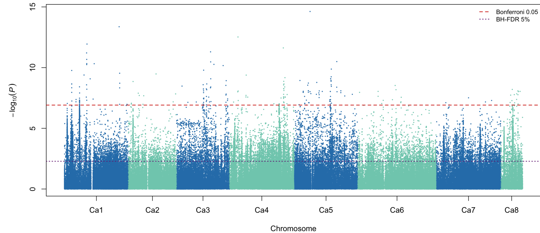
DTM CV1 partition 1 fold 1: meta-GWAS
