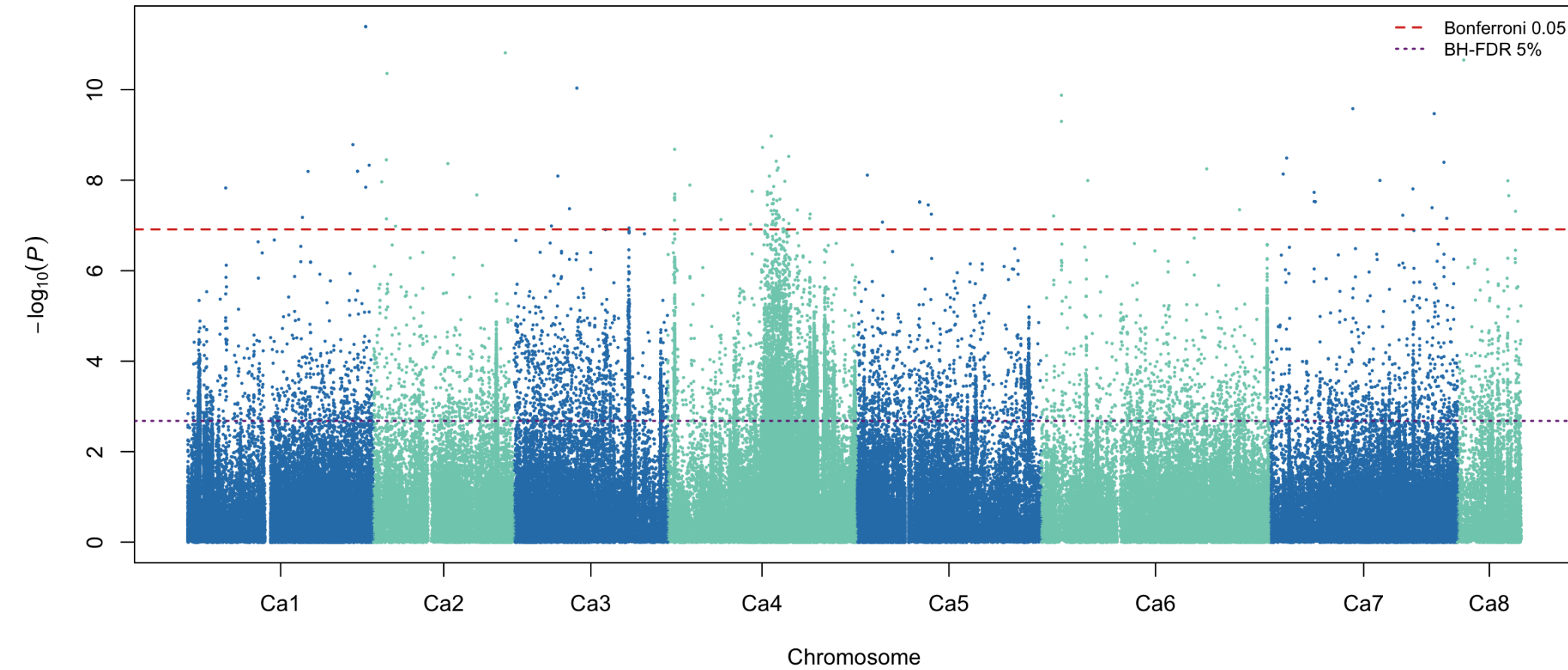
PH CV2 partition 1 fold 1: meta-GWAS
