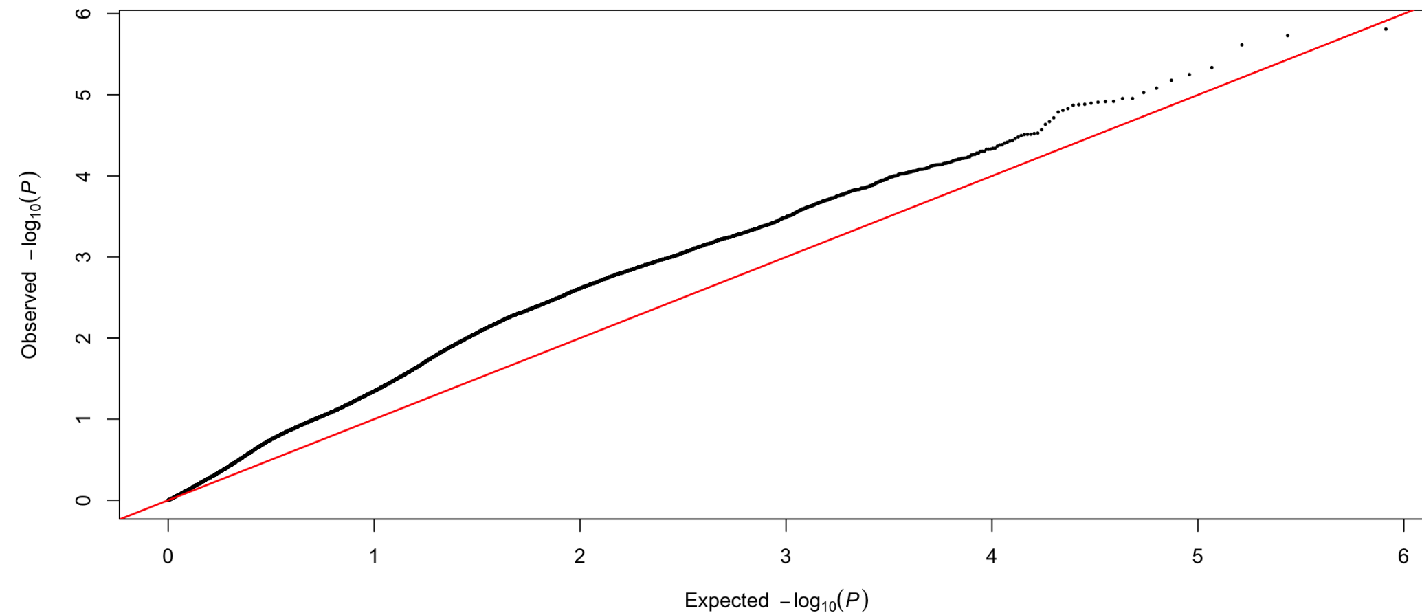
YPP CV0 partition 1 fold 1: Q-Q
