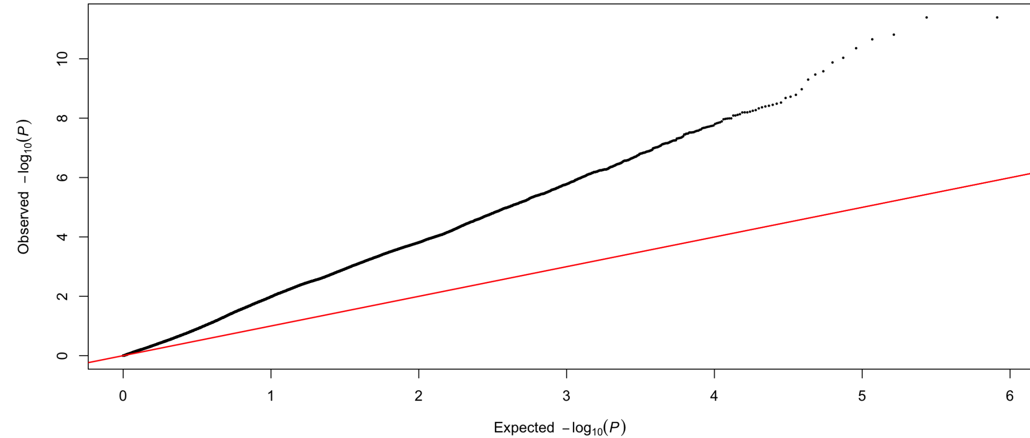
PH CV2 partition 1 fold 1: Q-Q
