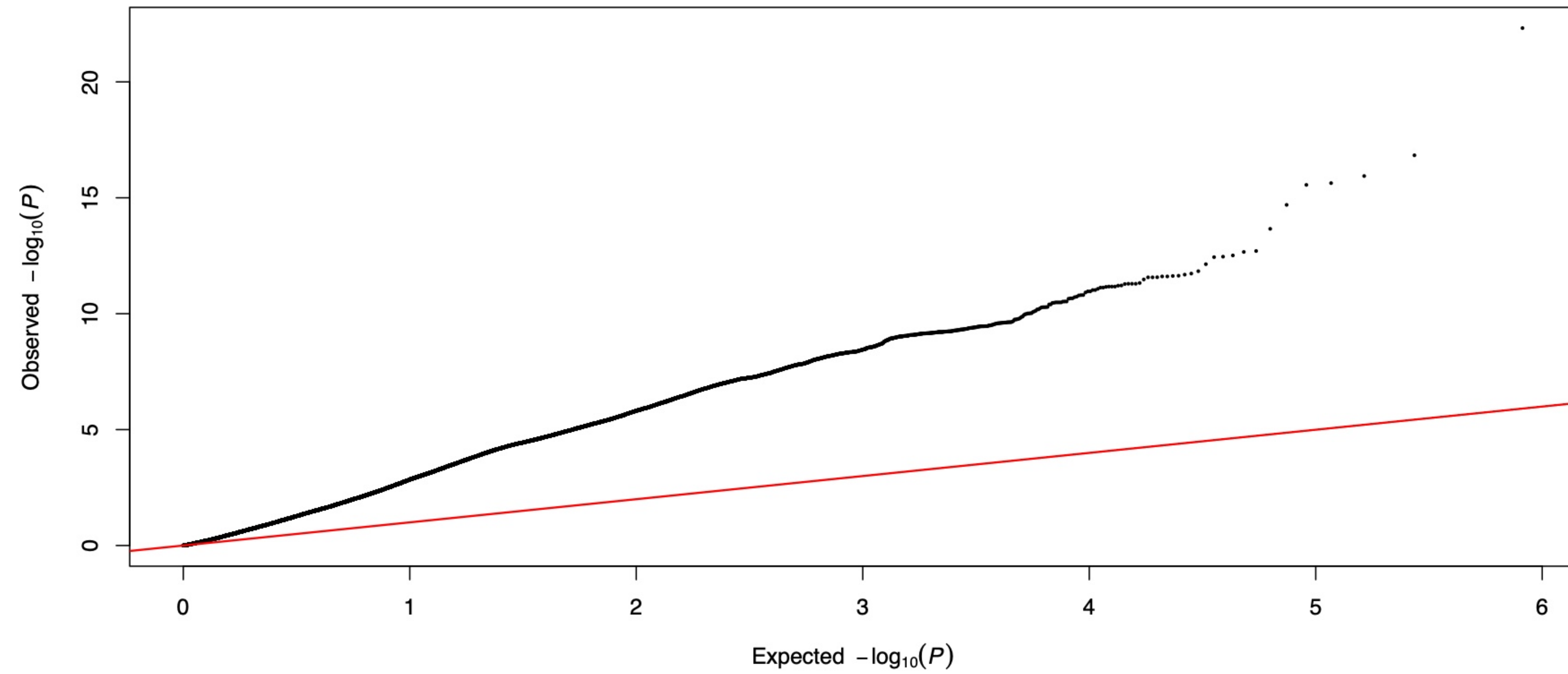
DTF CV00 partition 1 fold 1: Q-Q
