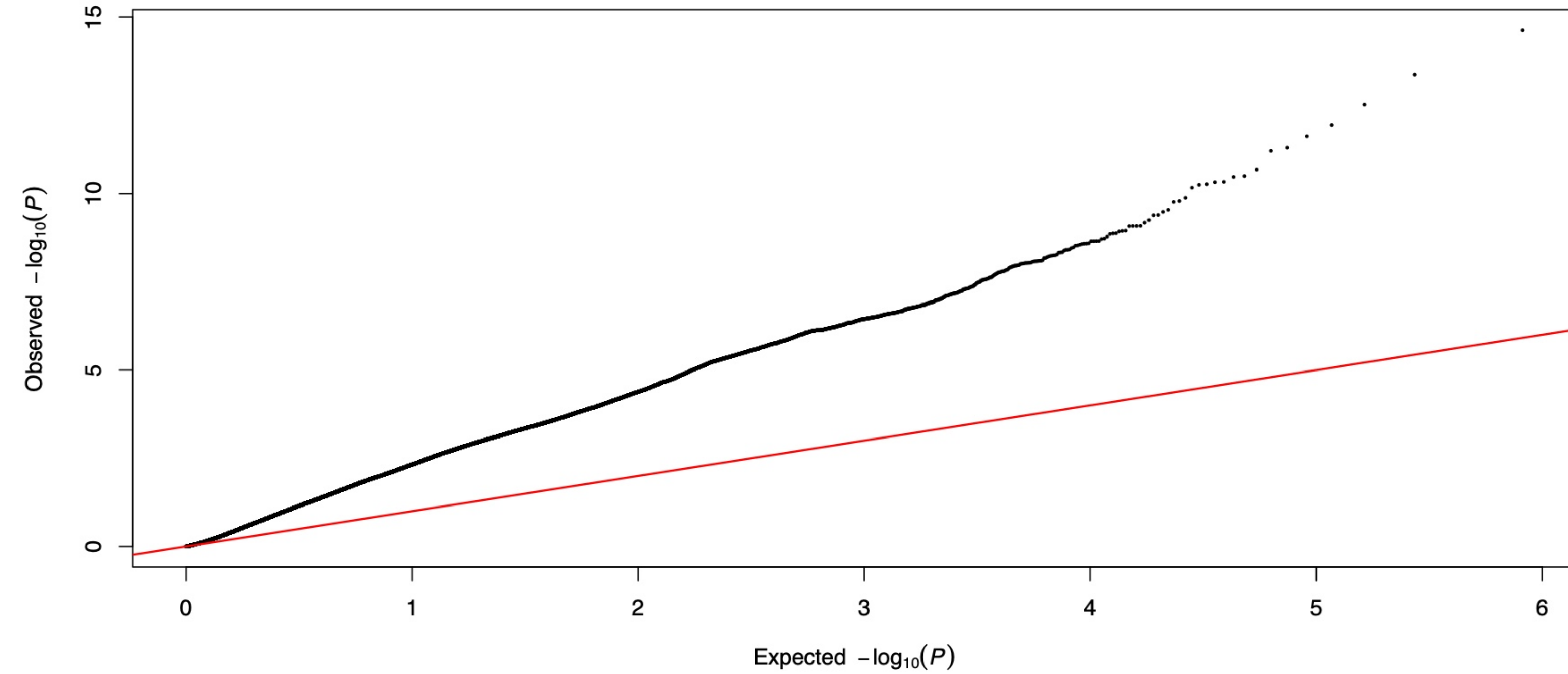
DTM CV1 partition 1 fold 1: Q-Q
