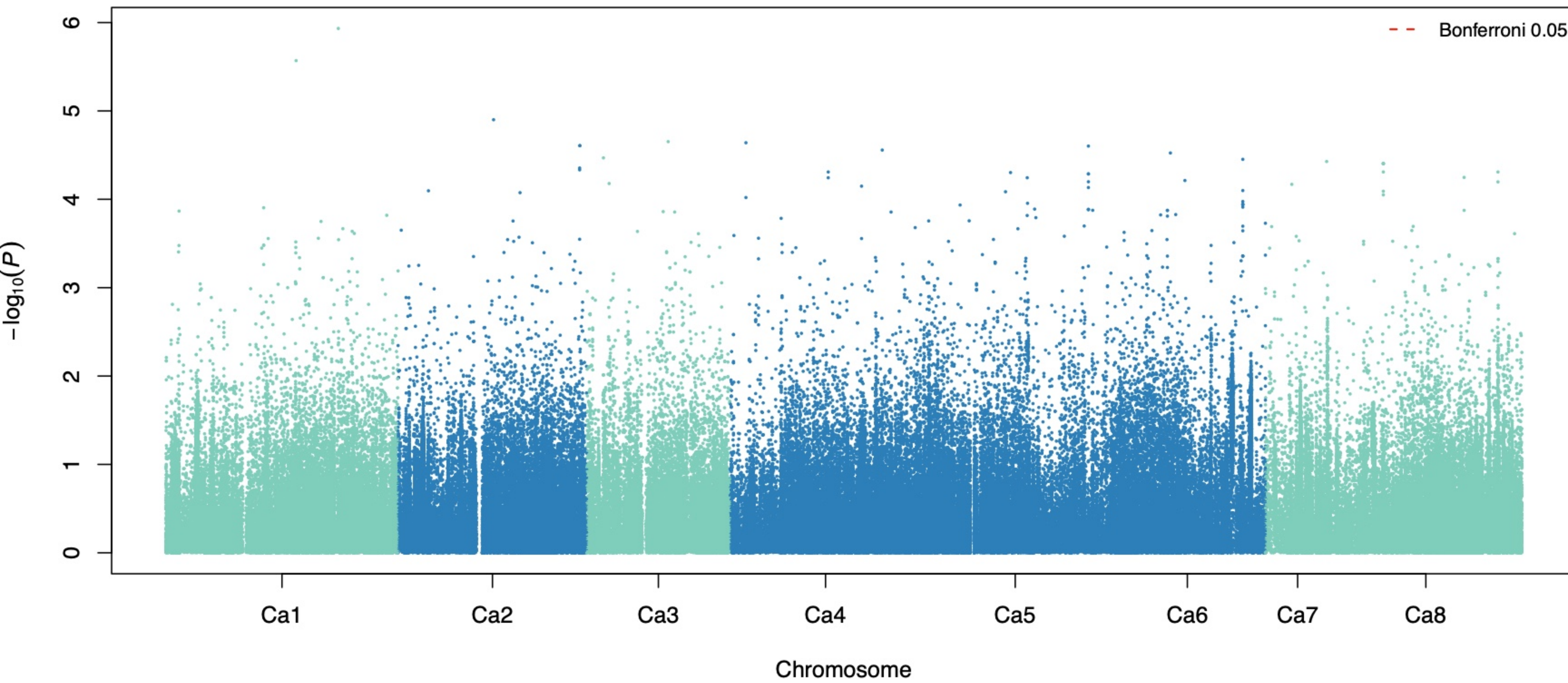
PPP CV0 partition 1 fold 1: meta-GWAS
