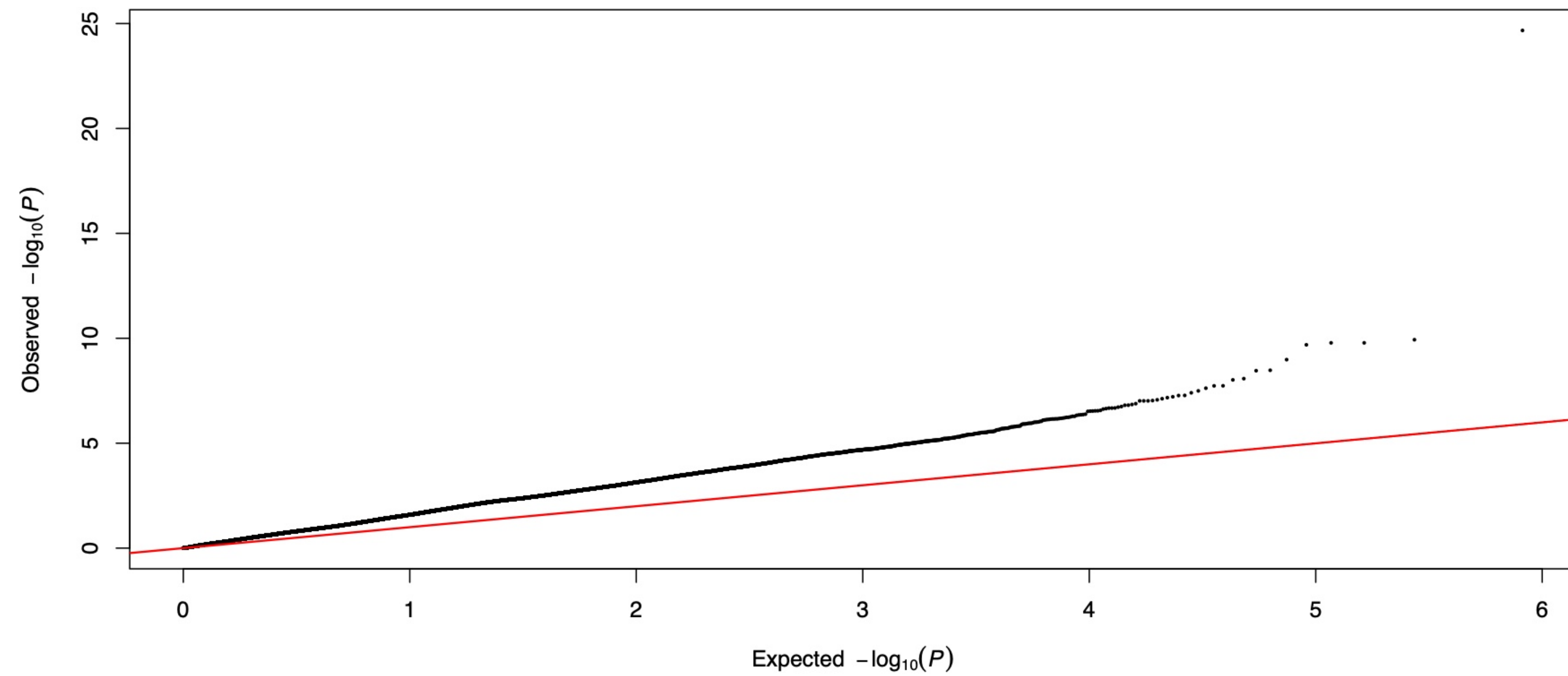
PH CV00 partition 1 fold 1: Q-Q
