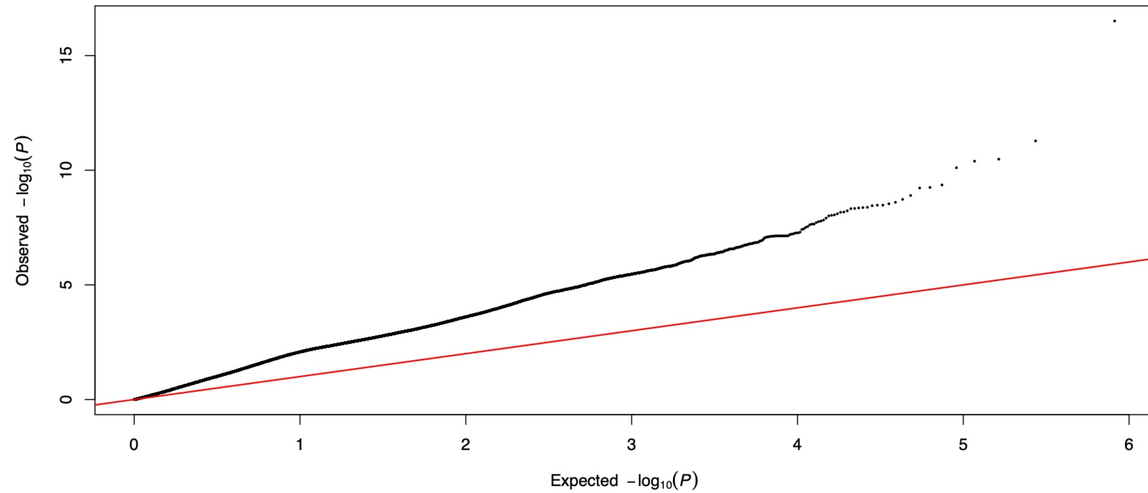
HSW CV00 partition 1 fold 1: Q-Q
