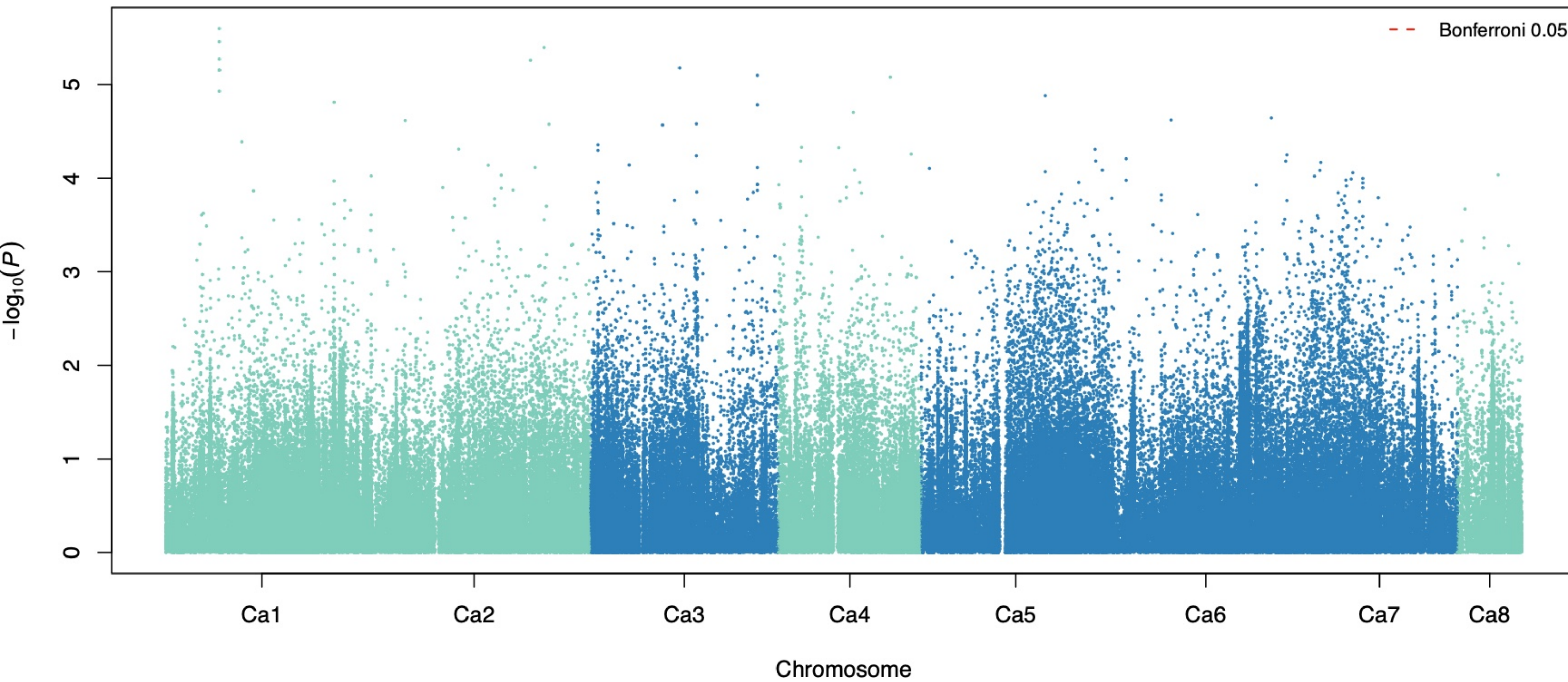
PPP CV2 partition 1 fold 1: meta-GWAS
