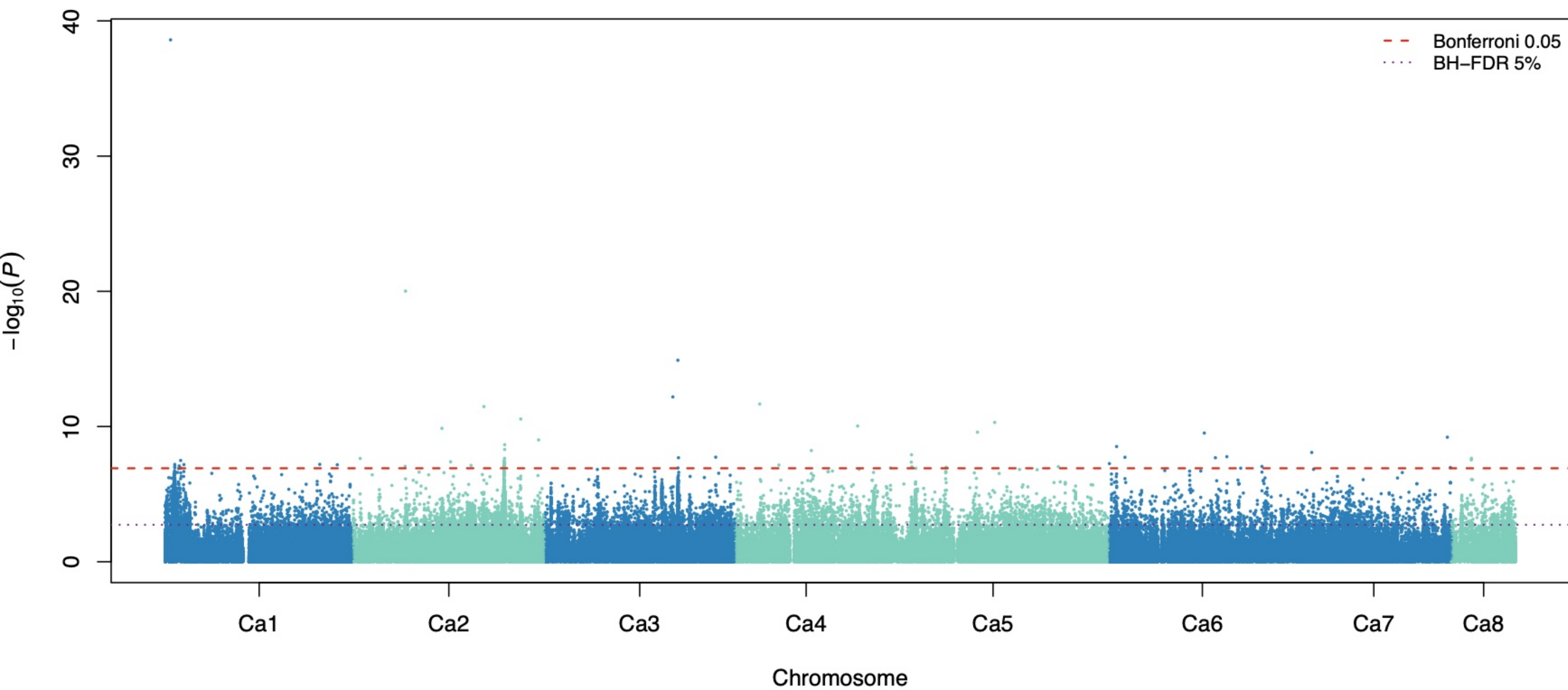
HSW CV0 partition 1 fold 1: meta-GWAS
