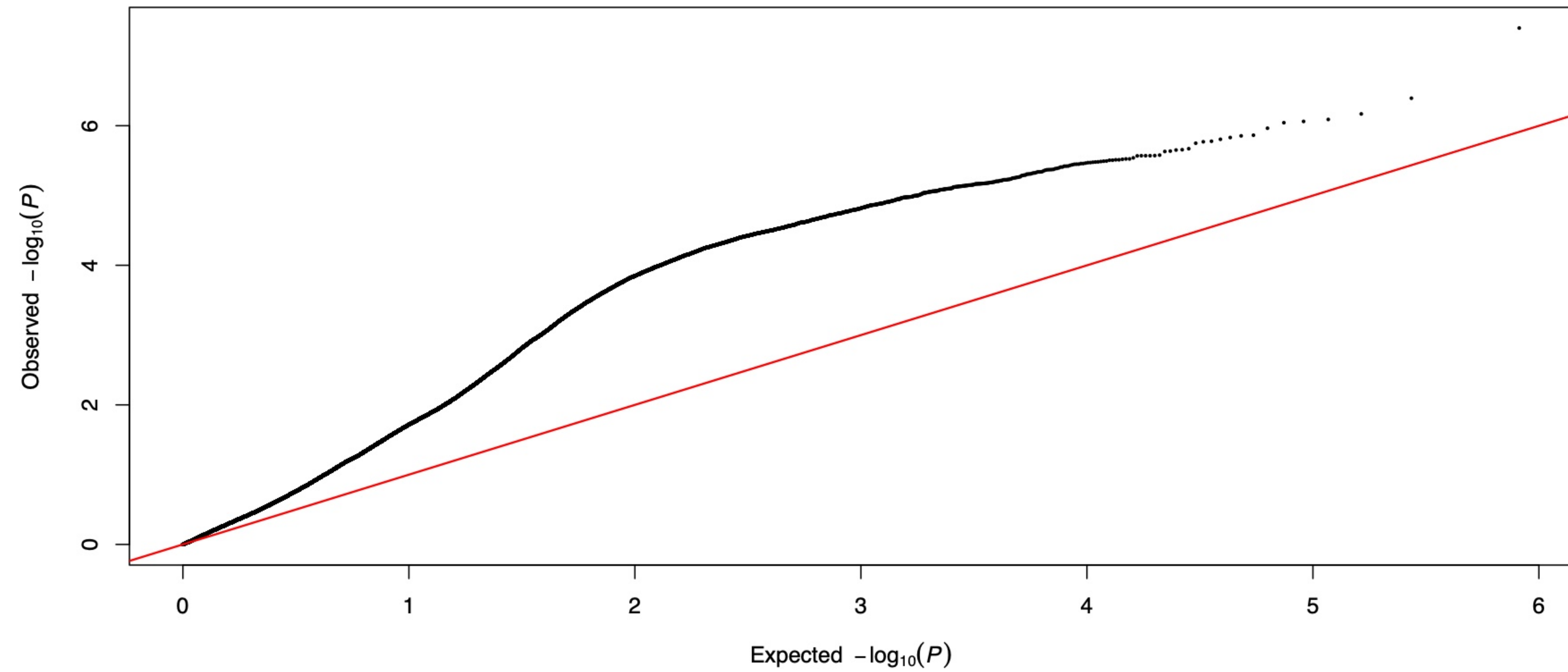
YPP CV1 partition 1 fold 1: Q-Q
