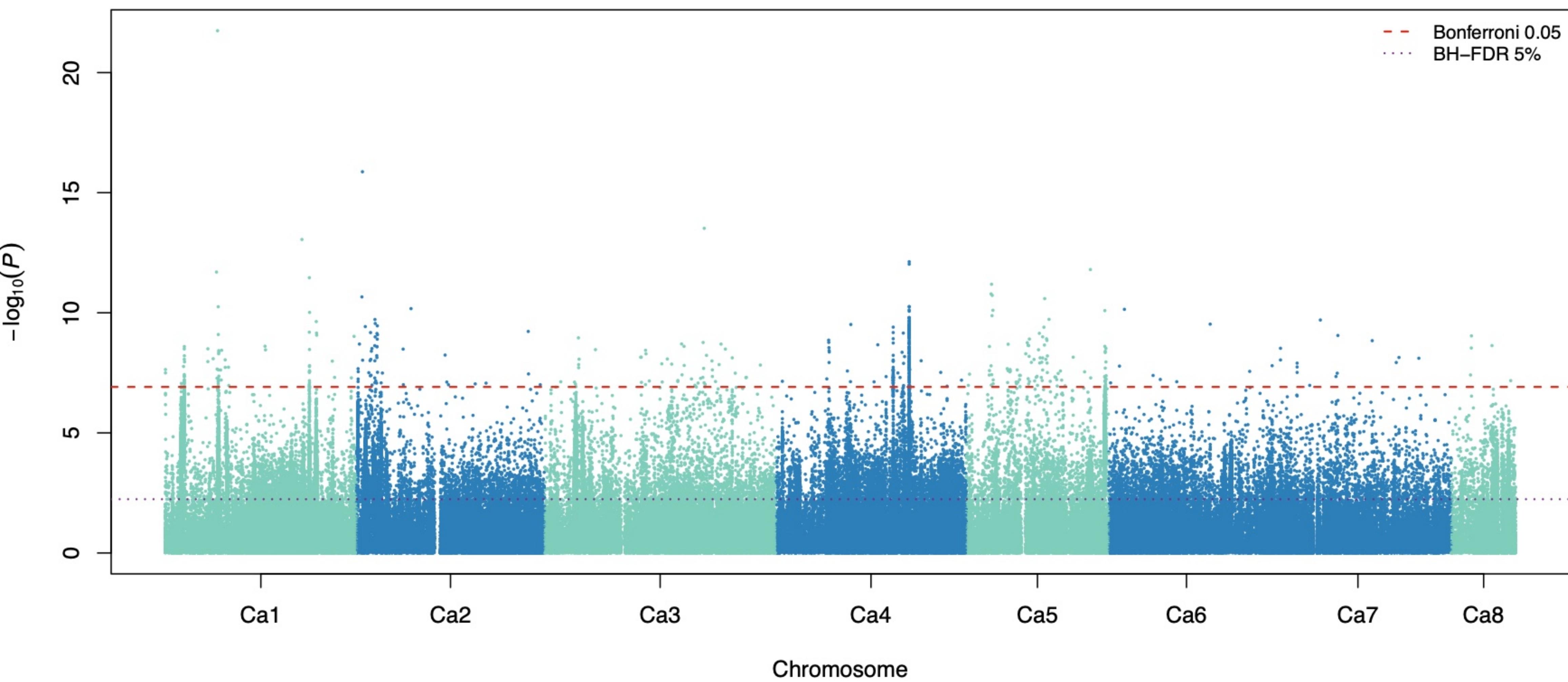
HSW CV2 partition 1 fold 1: meta-GWAS
