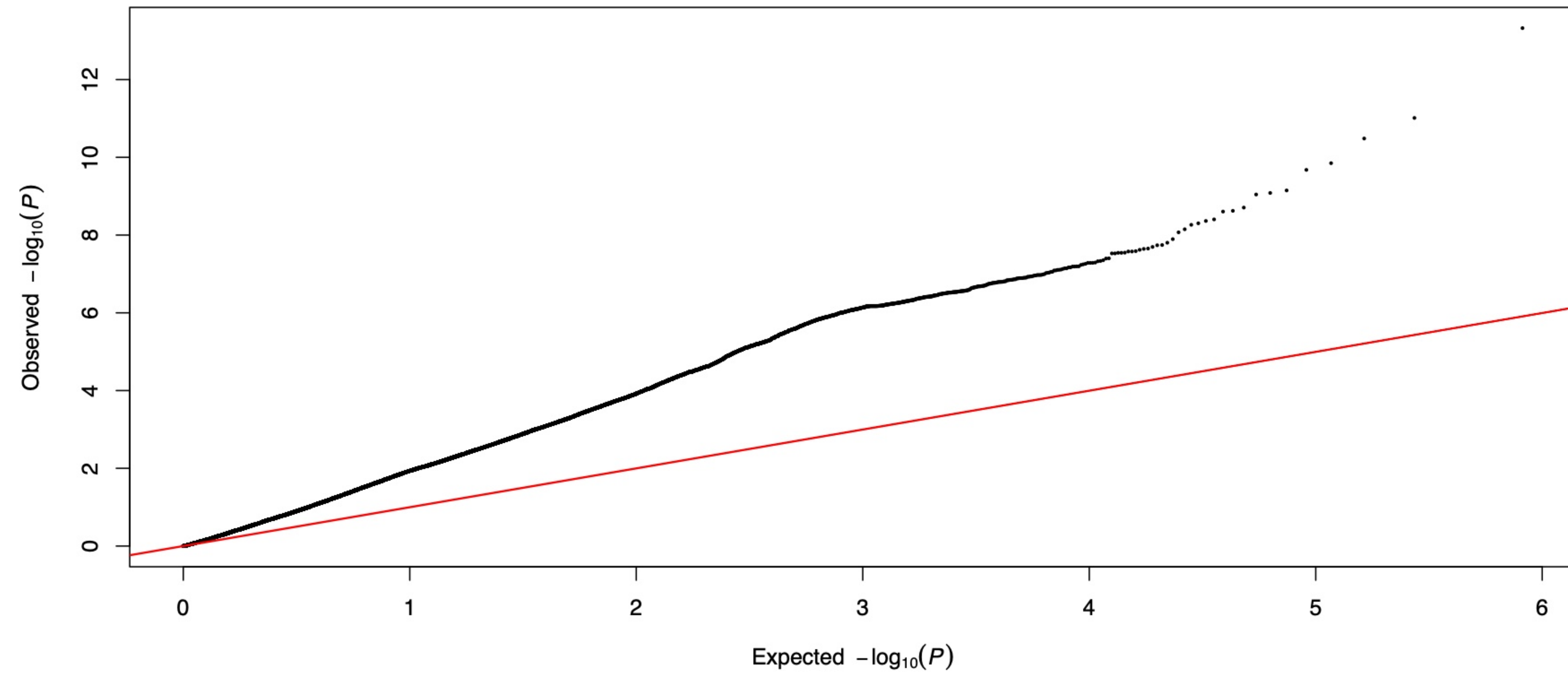
DTM CV00 partition 1 fold 1: Q-Q
