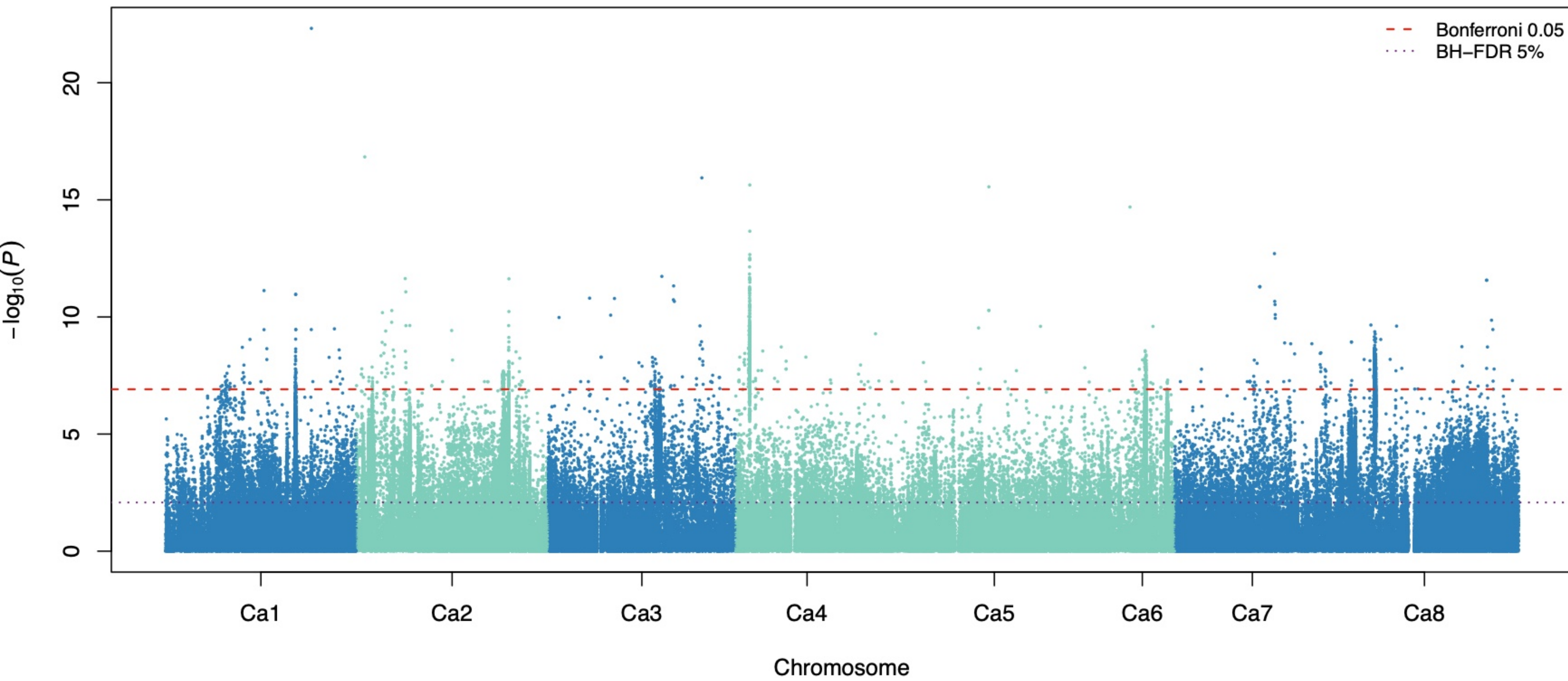
DTF CV00 partition 1 fold 1: meta-GWAS
