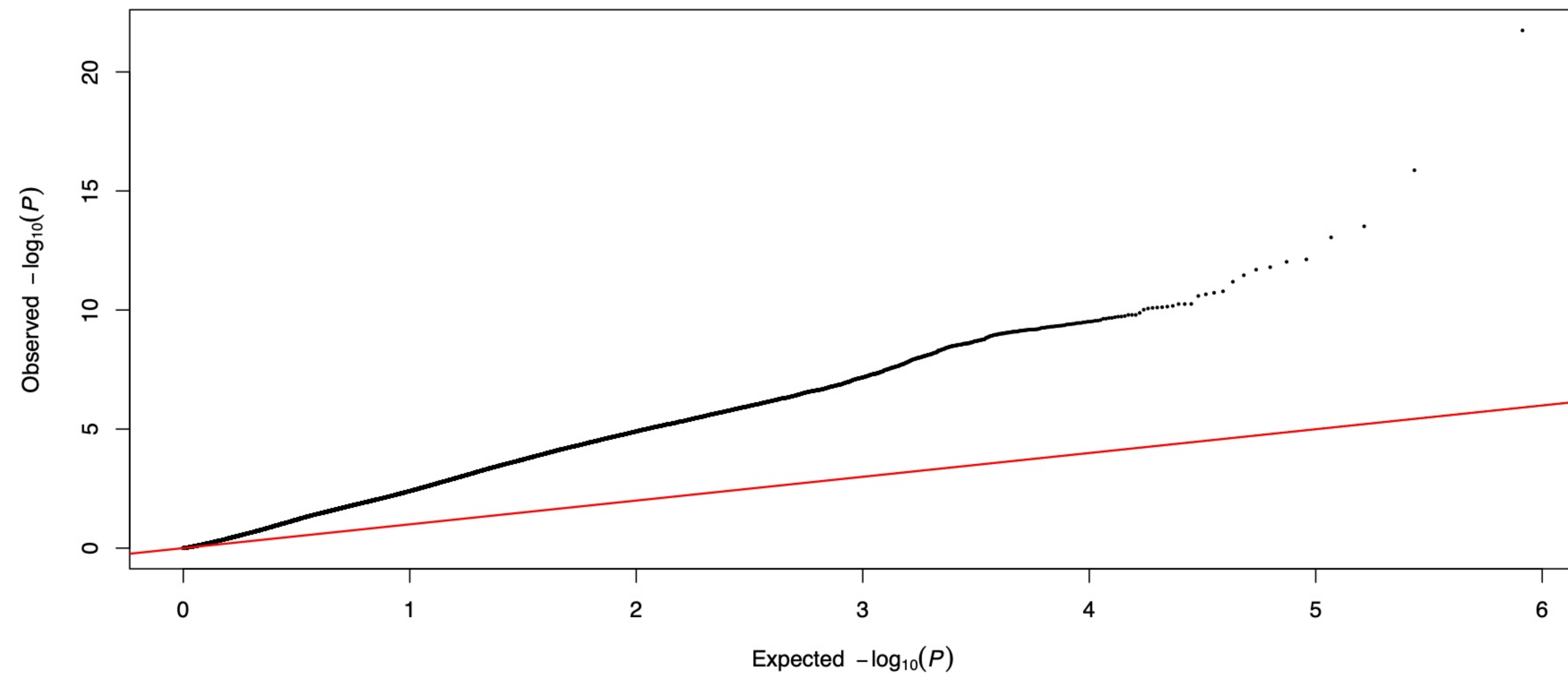
HSW CV2 partition 1 fold 1: Q-Q
