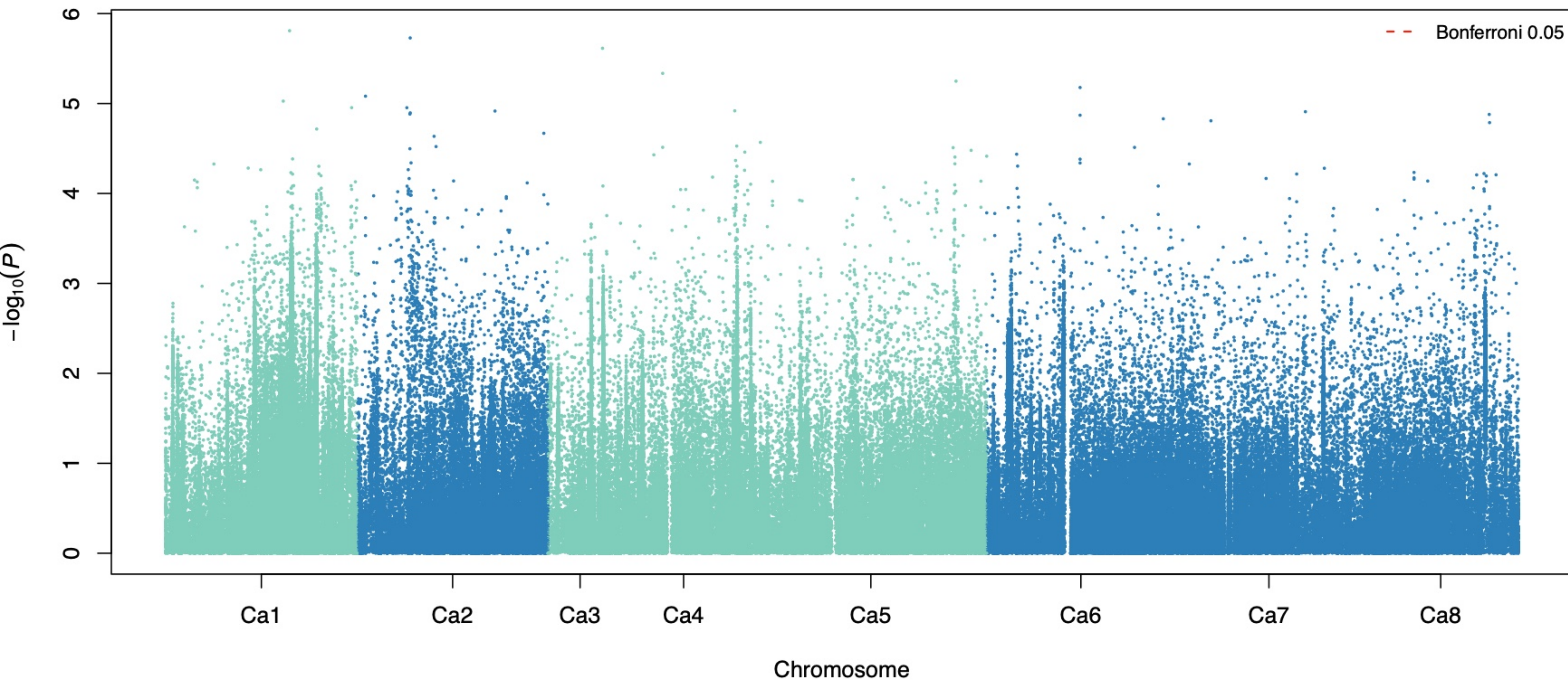
YPP CV0 partition 1 fold 1: meta-GWAS
