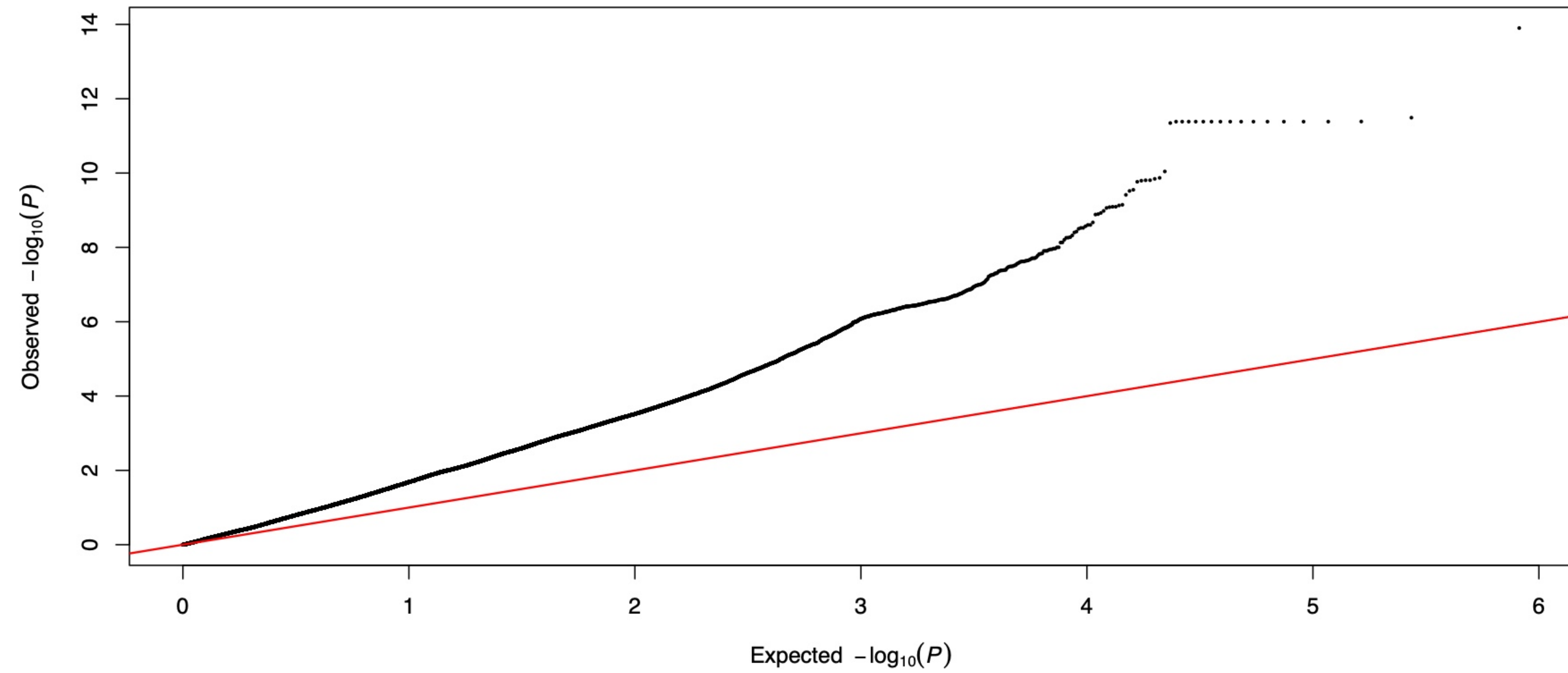
PH CV1 partition 1 fold 1: Q-Q
