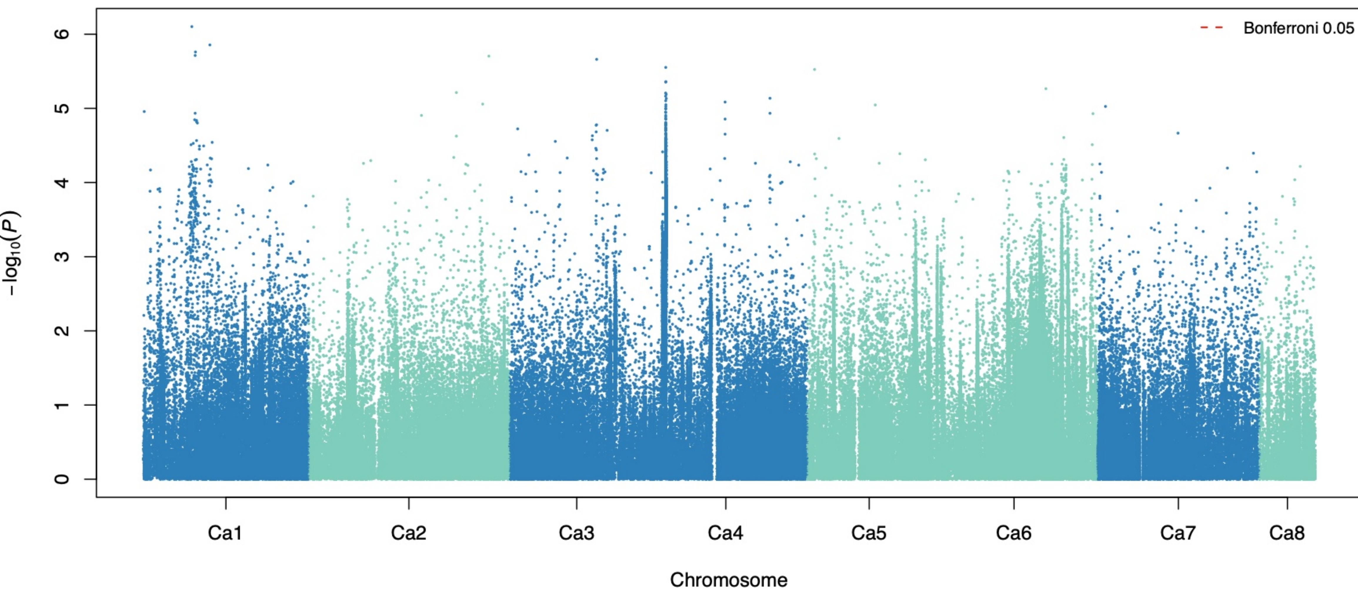
YPP CV2 partition 1 fold 1: meta-GWAS
