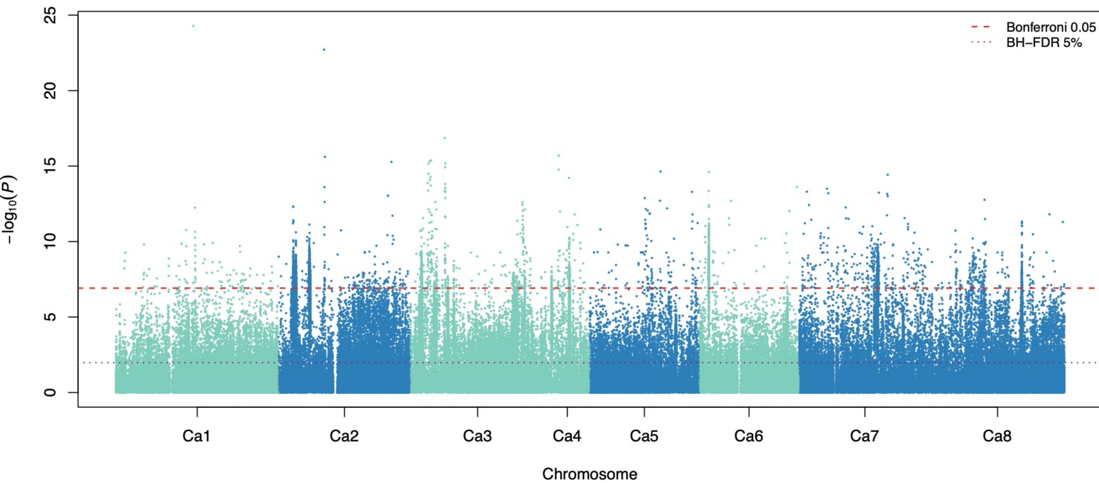
DTF CV1 partition 1 fold 1: meta-GWAS
