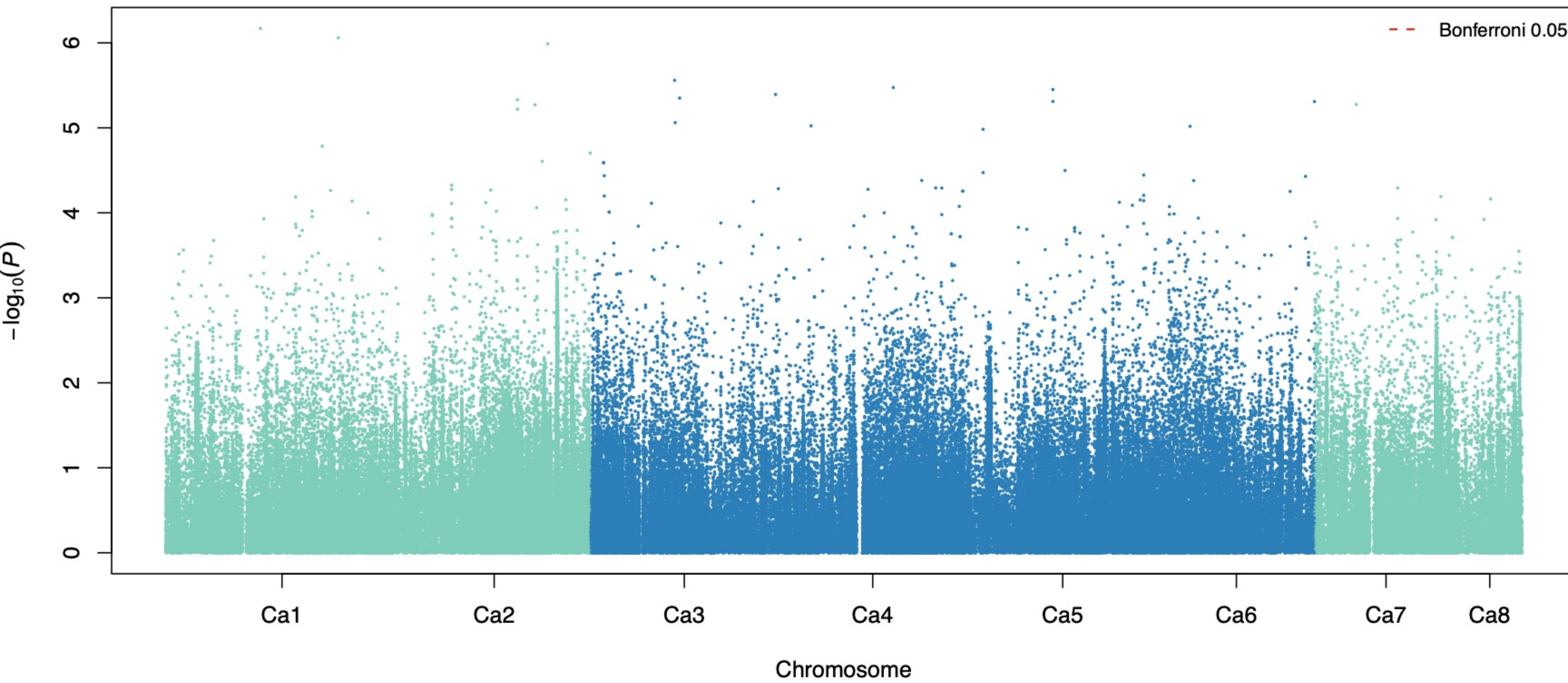
PPP CV00 partition 1 fold 1: meta-GWAS
