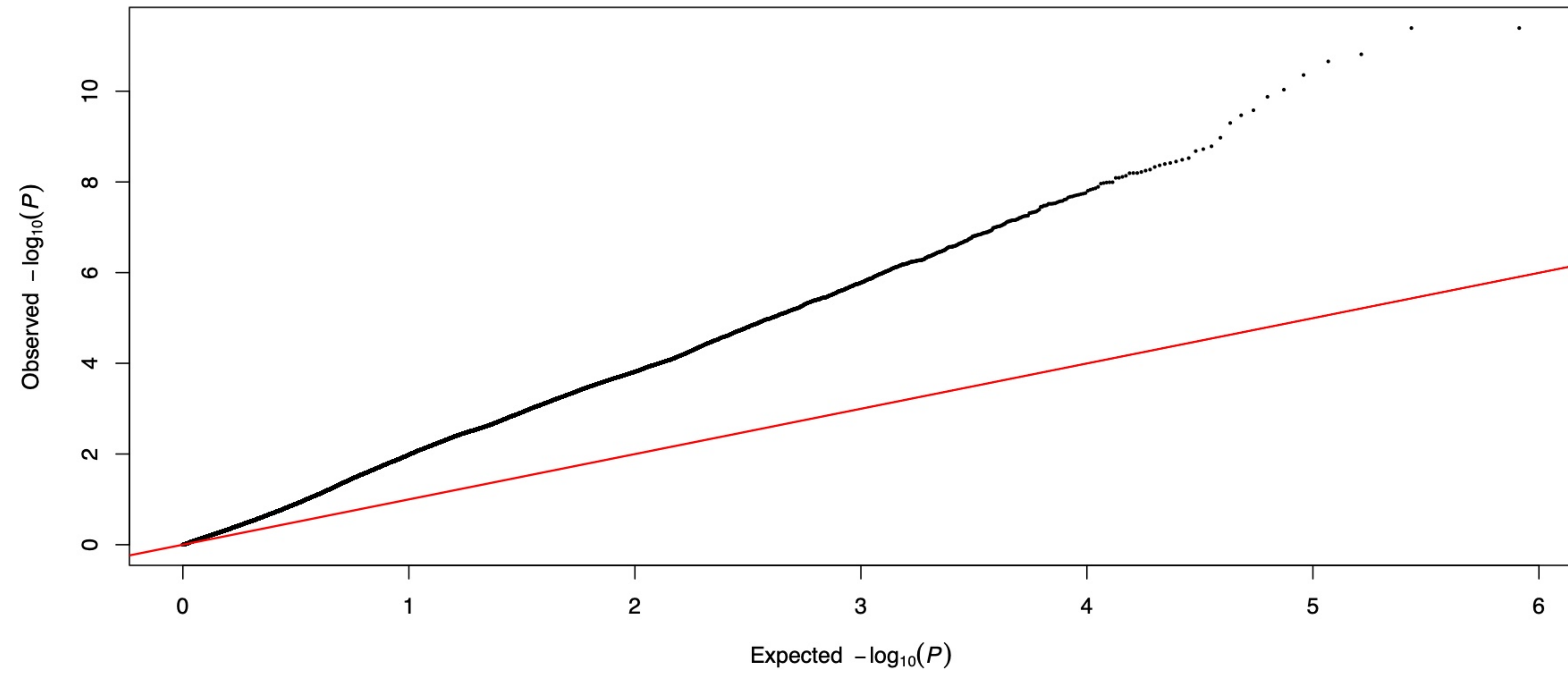
PH CV2 partition 1 fold 1: Q-Q
