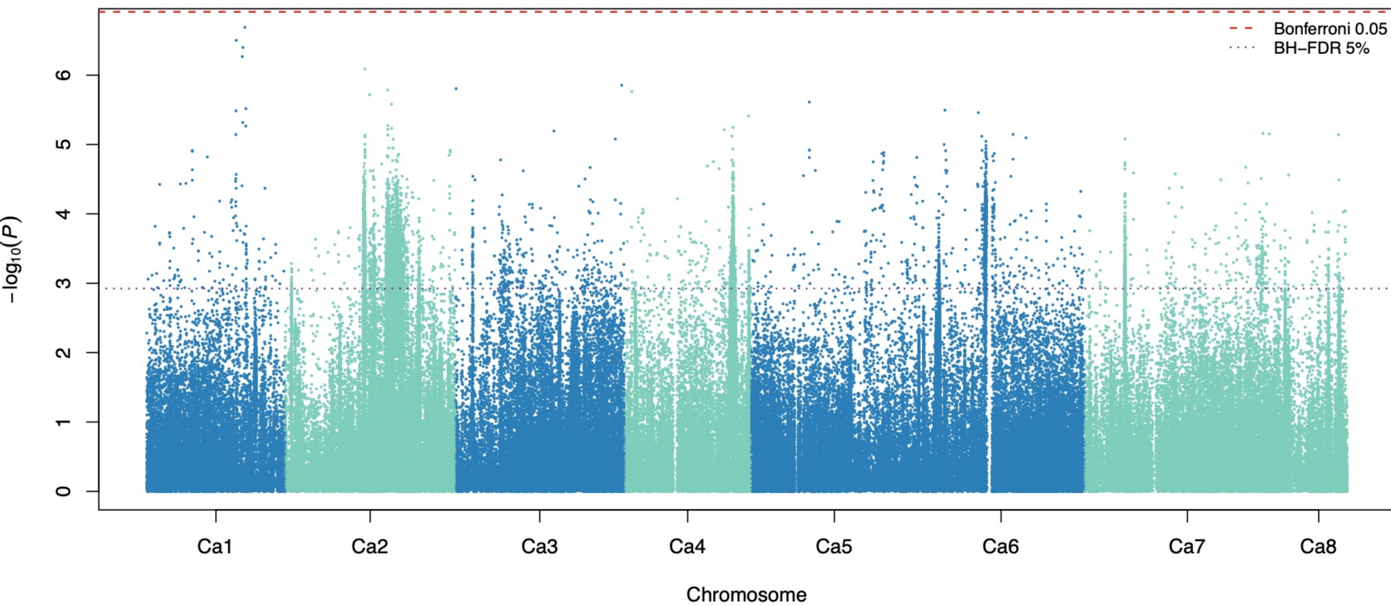
YPP CV00 partition 1 fold 1: meta-GWAS
