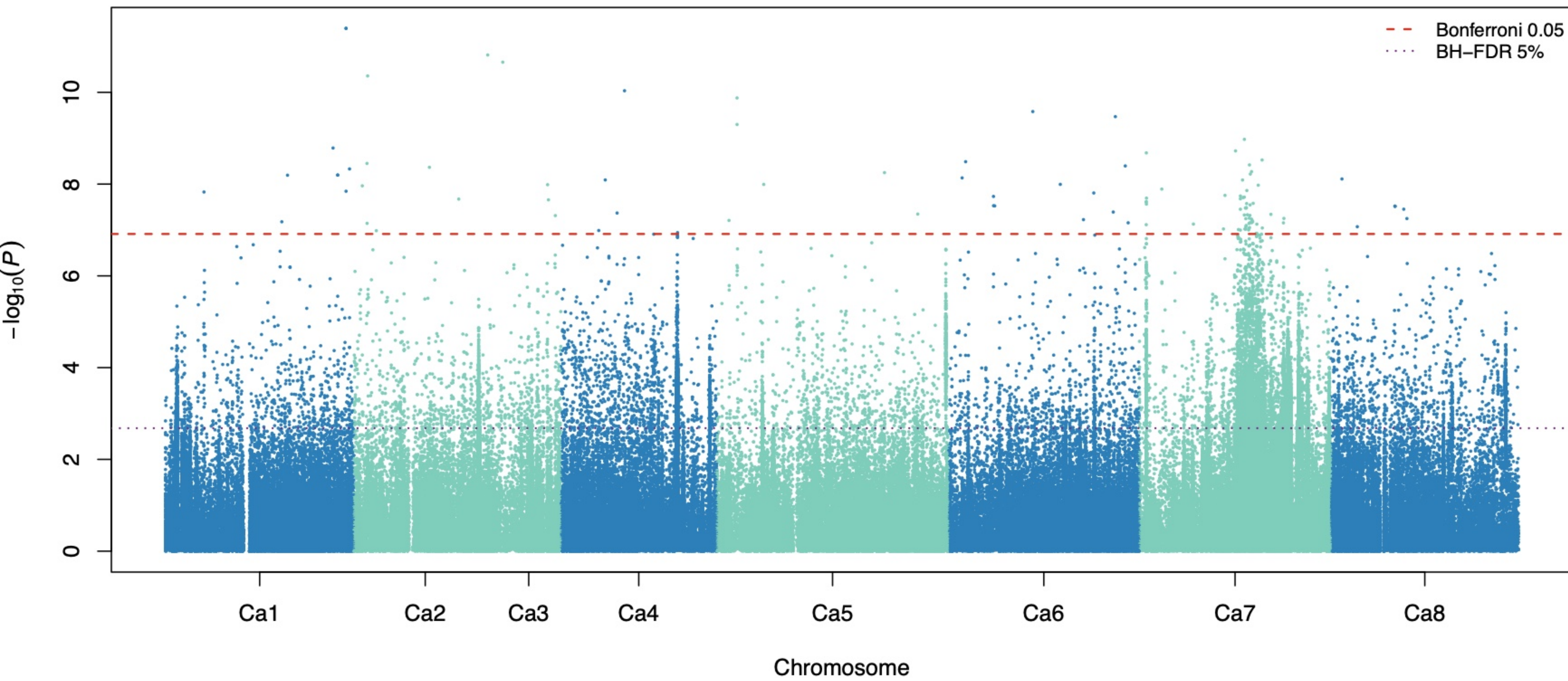
PH CV2 partition 1 fold 1: meta-GWAS
