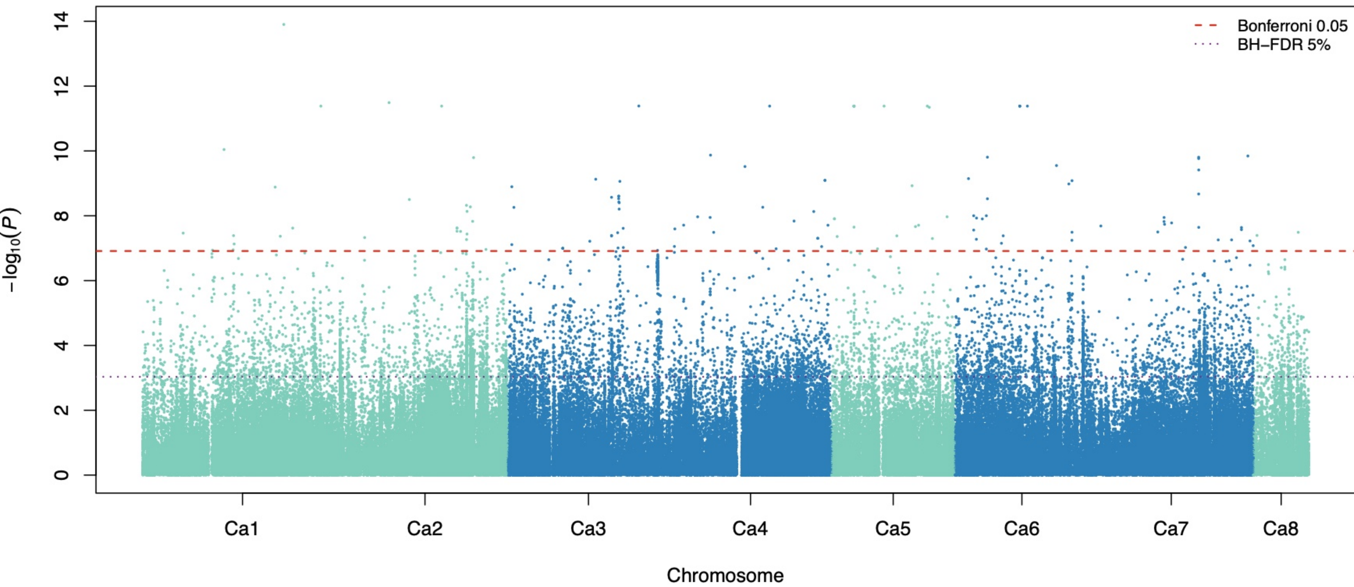
PH CV1 partition 1 fold 1: meta-GWAS
