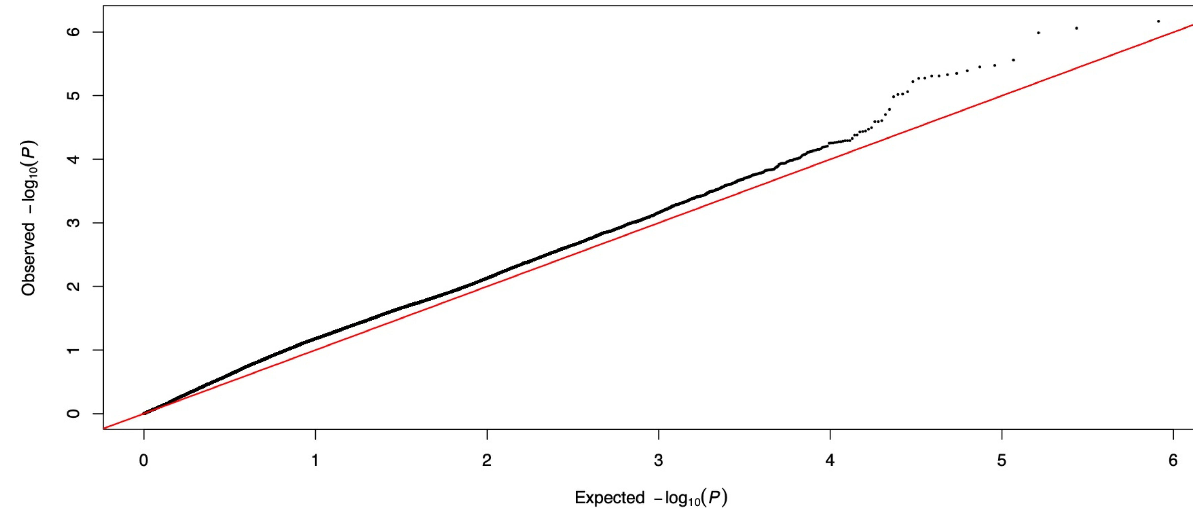
PPP CV00 partition 1 fold 1: Q-Q
