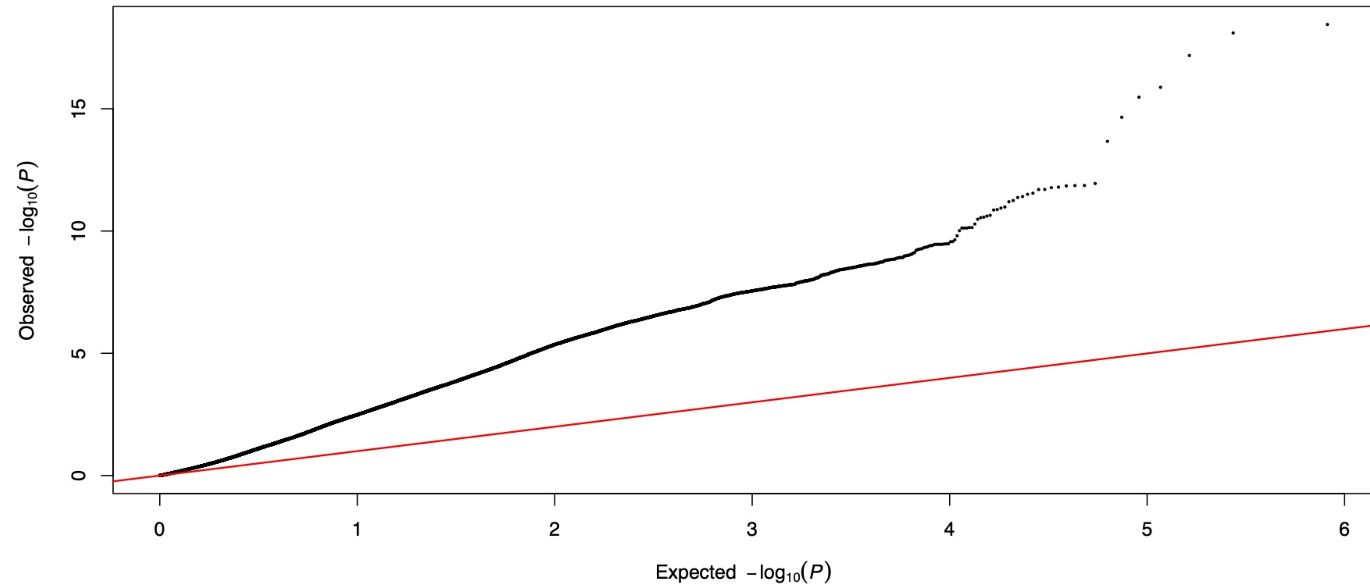
DTF CV0 partition 1 fold 1: Q-Q
