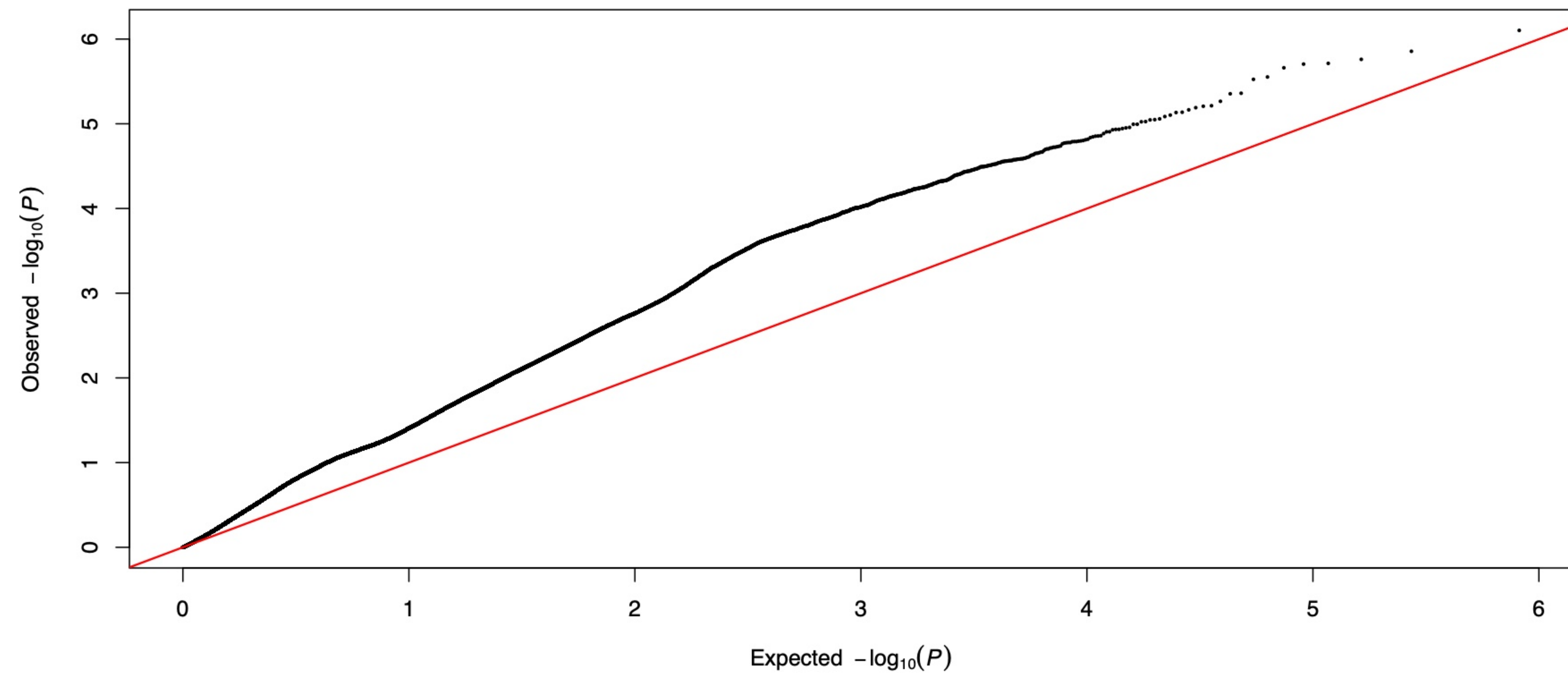
YPP CV2 partition 1 fold 1: Q-Q
