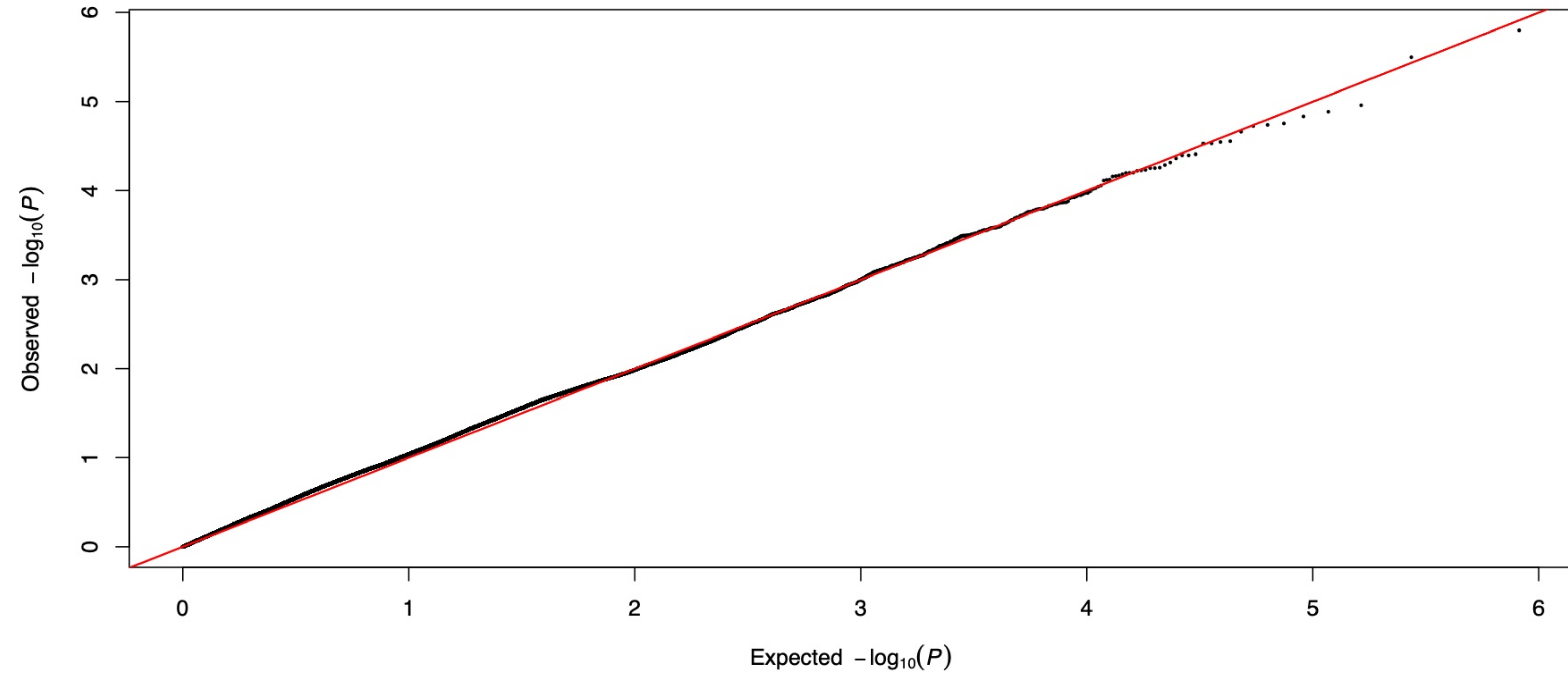
PPP CV1 partition 1 fold 1: Q-Q
