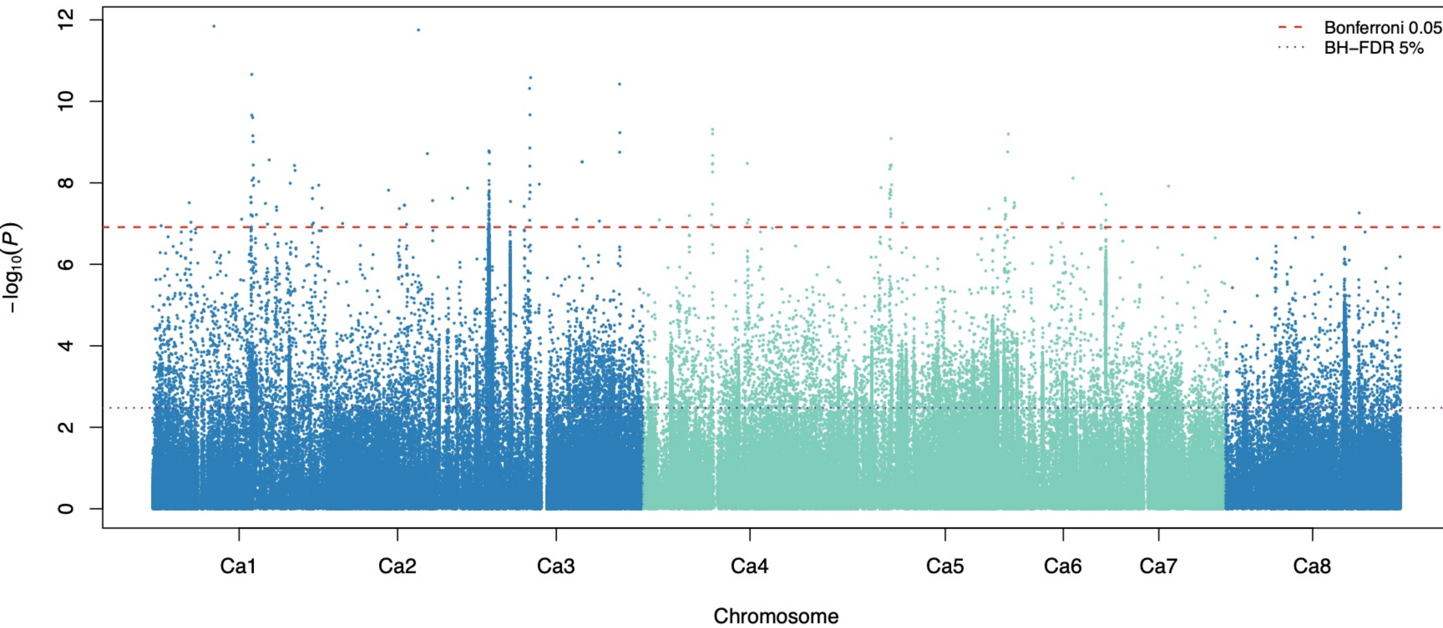
DTM CV2 partition 1 fold 1: meta-GWAS
