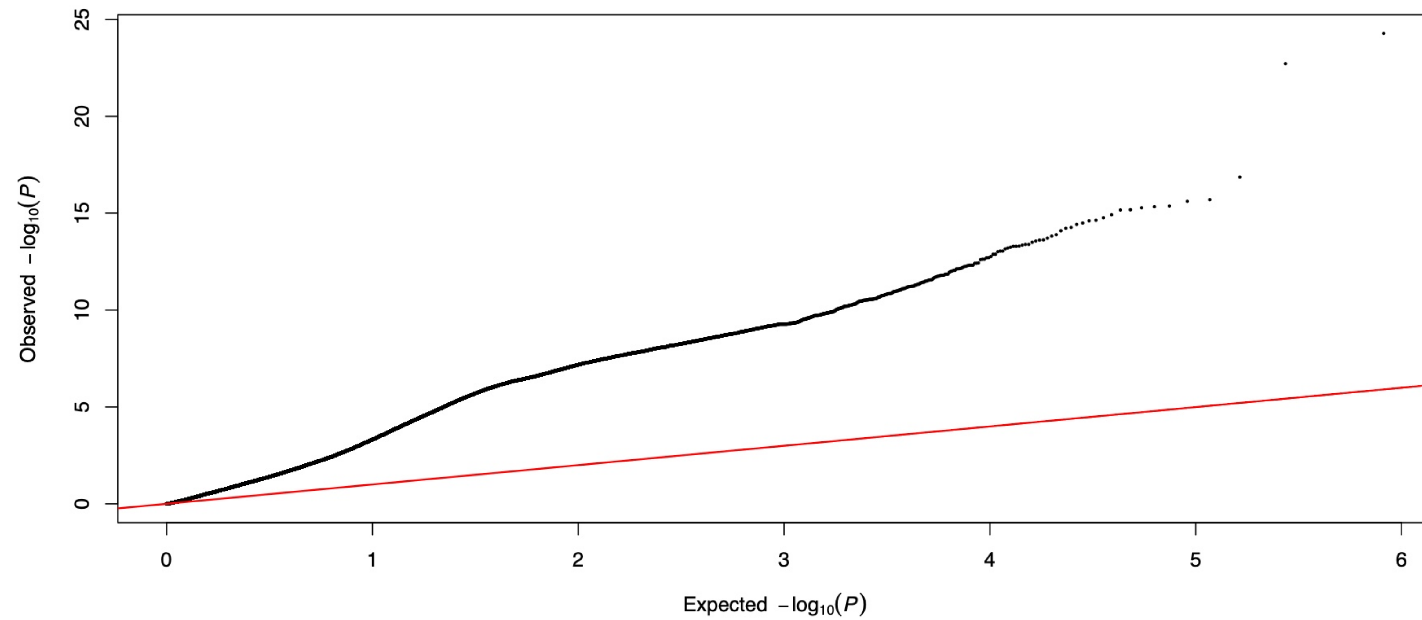
DTF CV1 partition 1 fold 1: Q-Q
