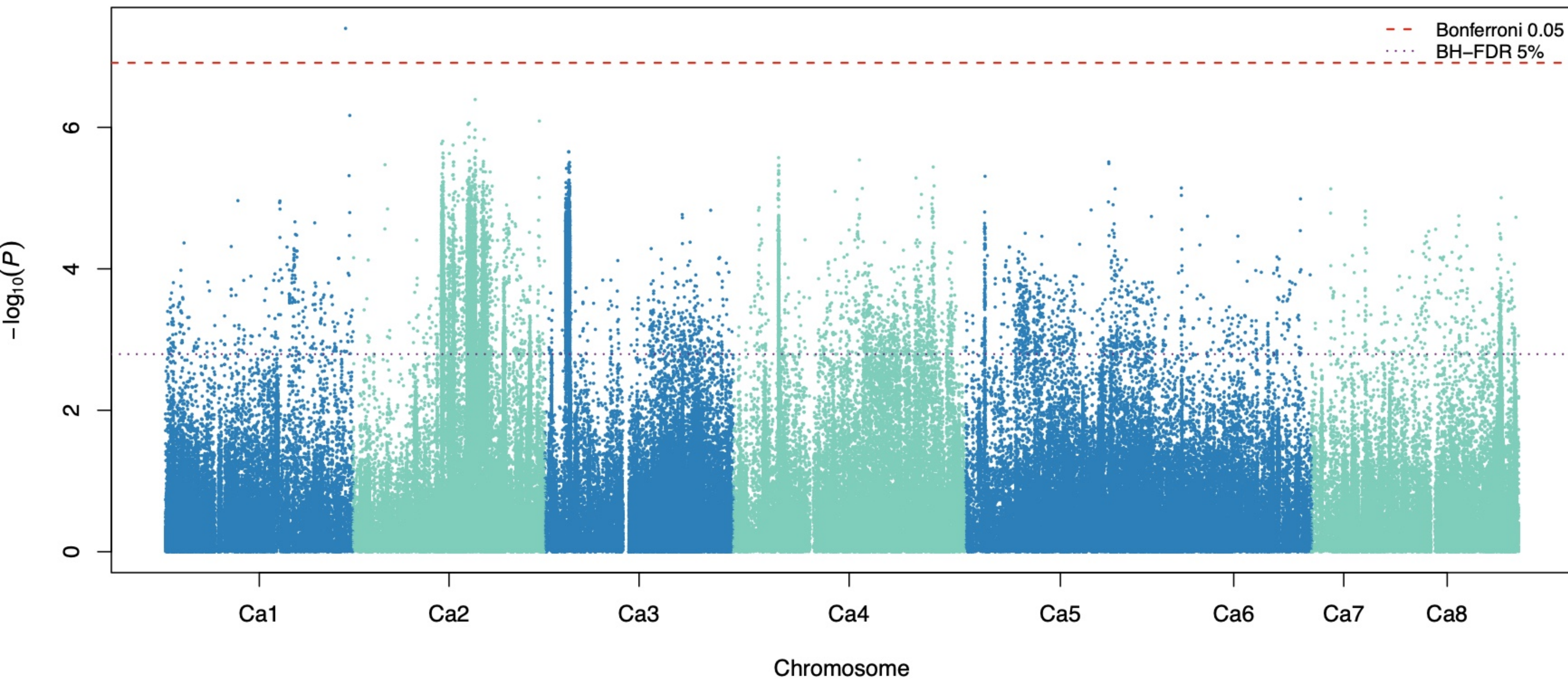
YPP CV1 partition 1 fold 1: meta-GWAS
