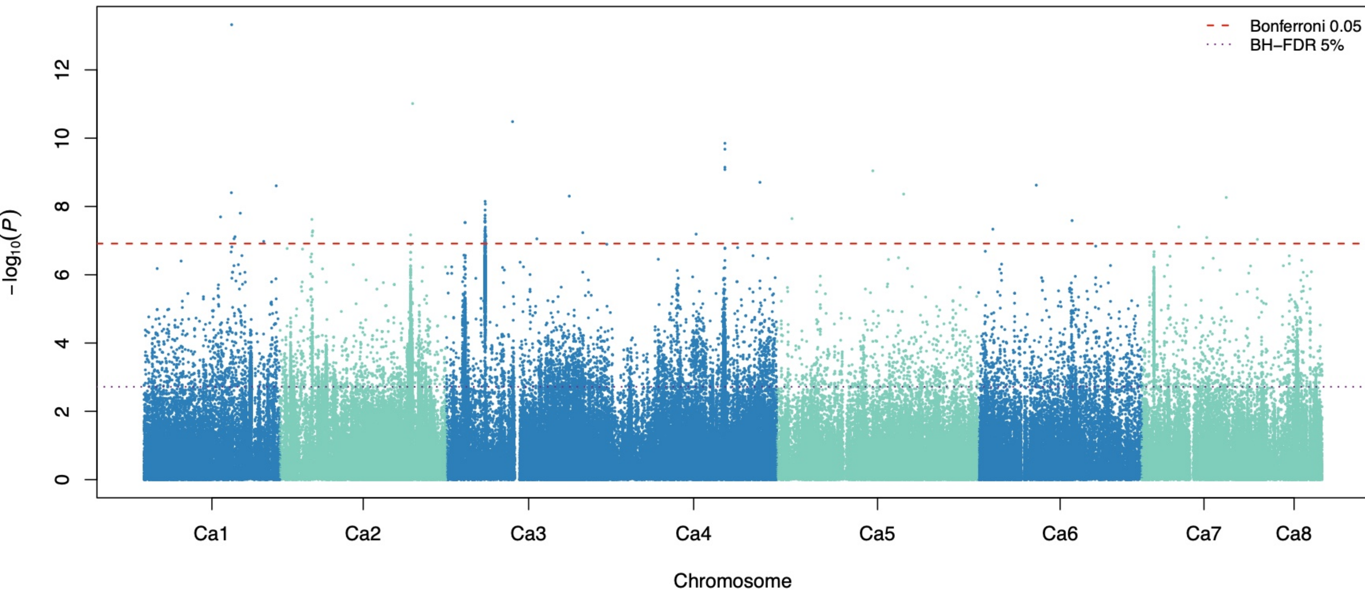
DTM CV00 partition 1 fold 1: meta-GWAS
