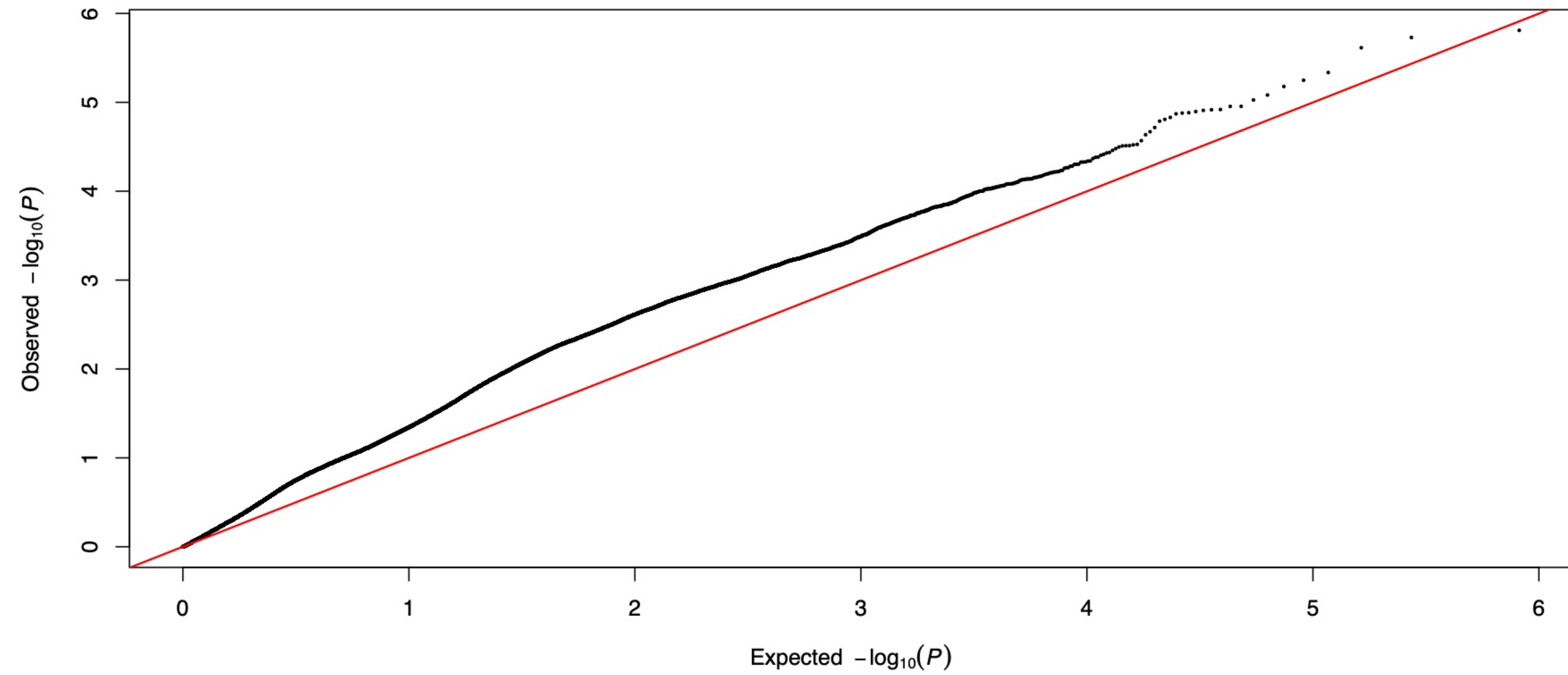
YPP CV0 partition 1 fold 1: Q-Q
