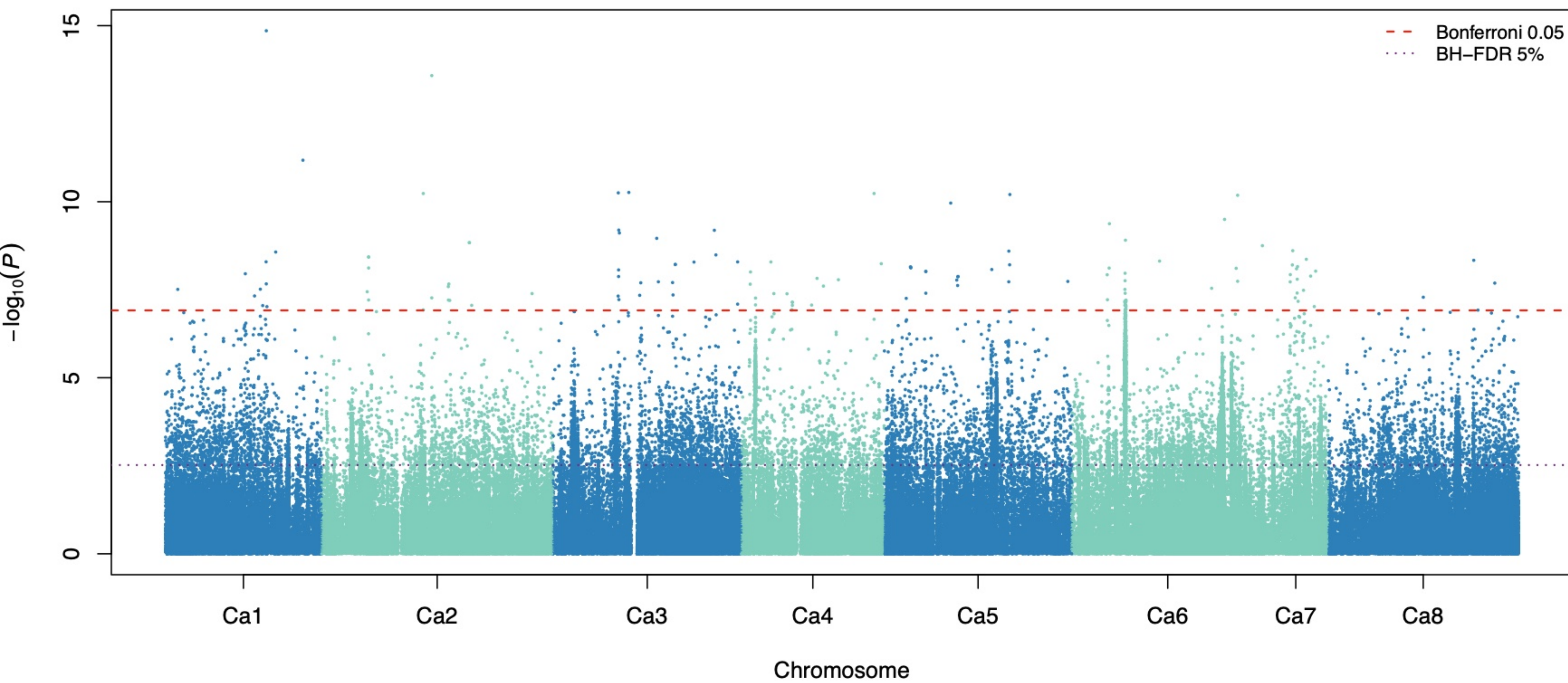
DTM CV0 partition 1 fold 1: meta-GWAS
