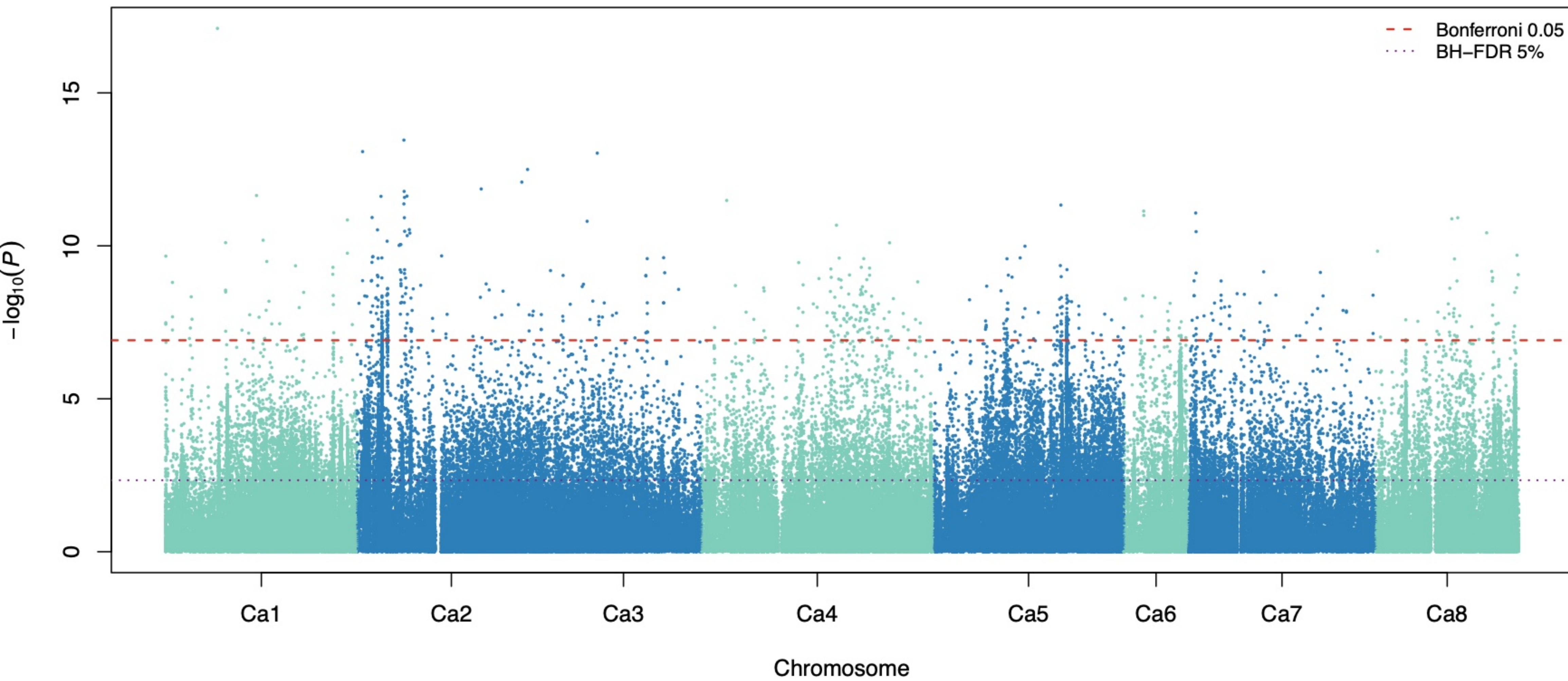
HSW CV1 partition 1 fold 1: meta-GWAS
