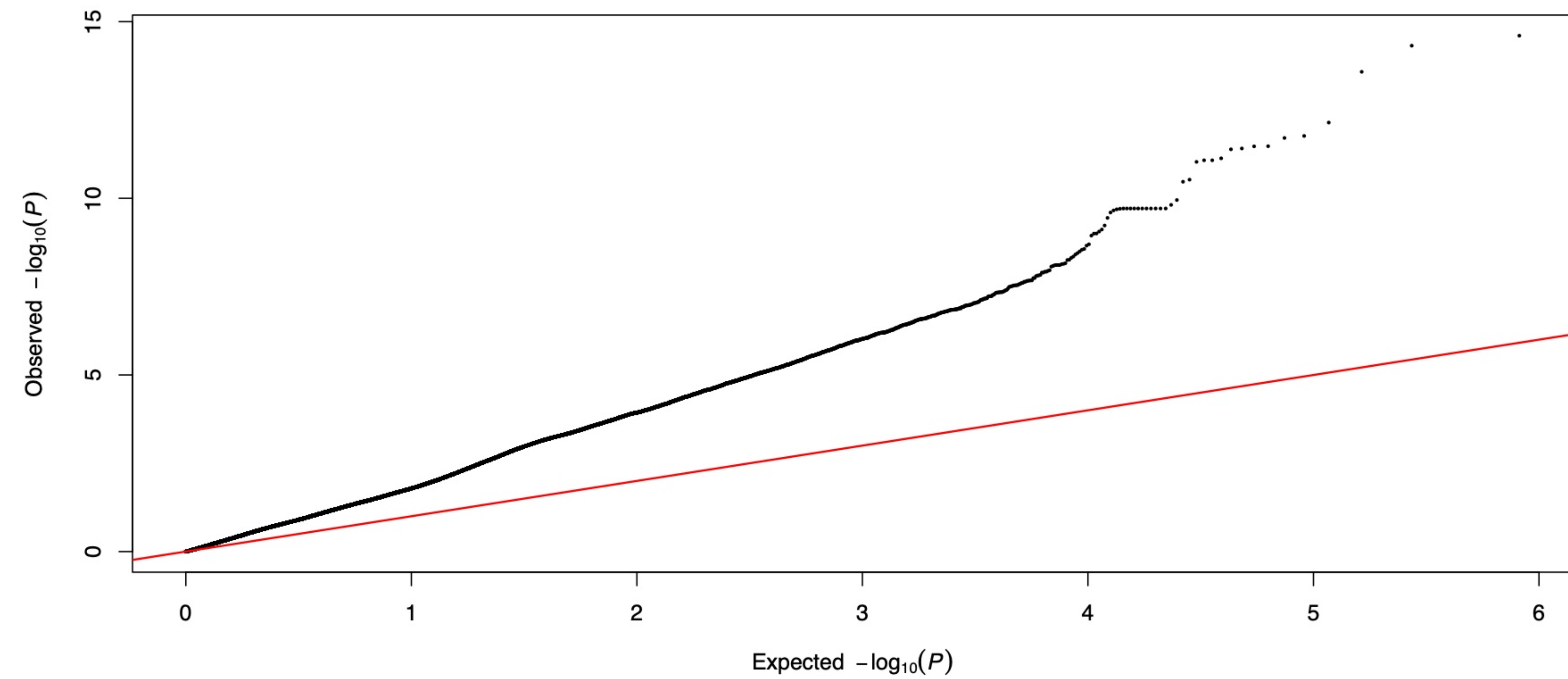
PH CV0 partition 1 fold 1: Q-Q
