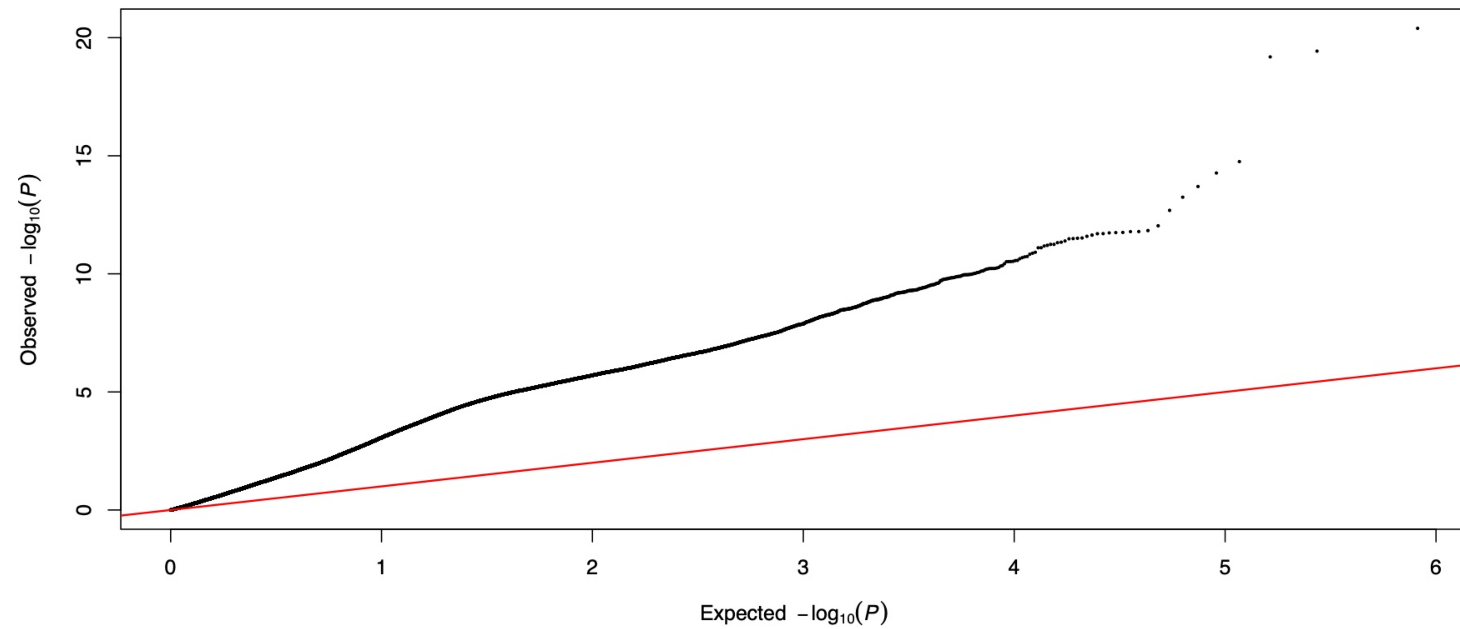
DTF CV2 partition 1 fold 1: Q-Q
