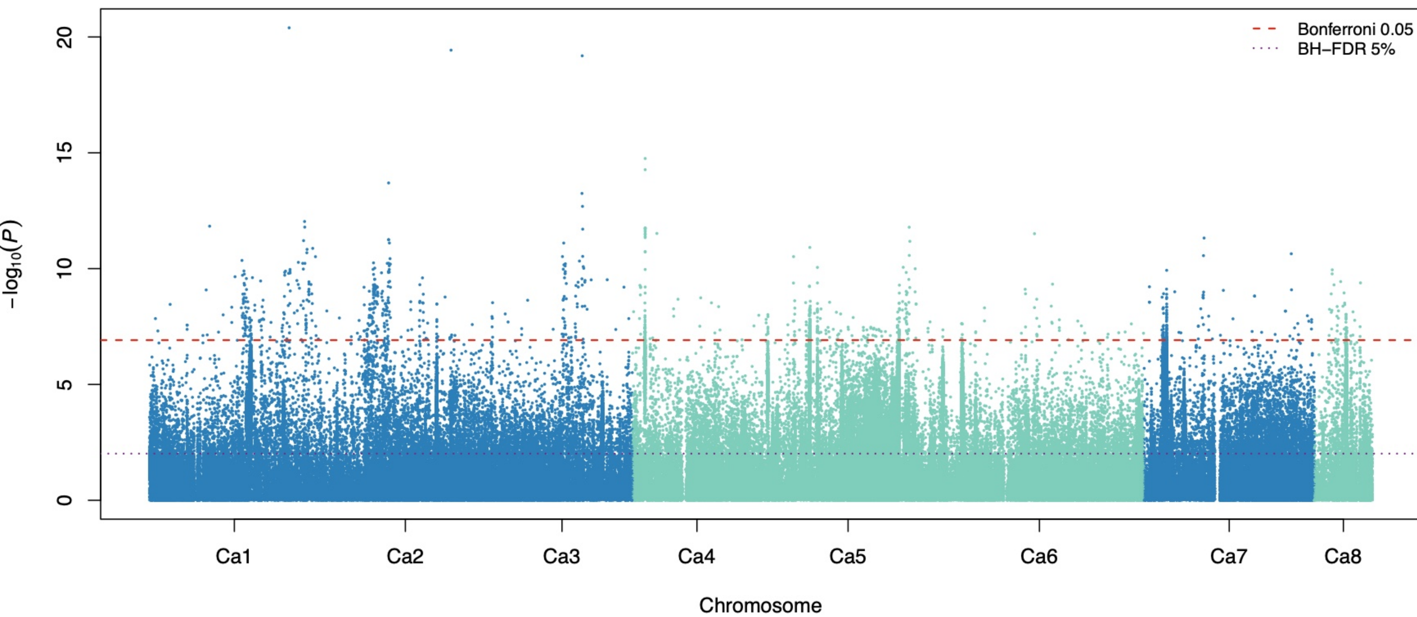
DTF CV2 partition 1 fold 1: meta-GWAS
