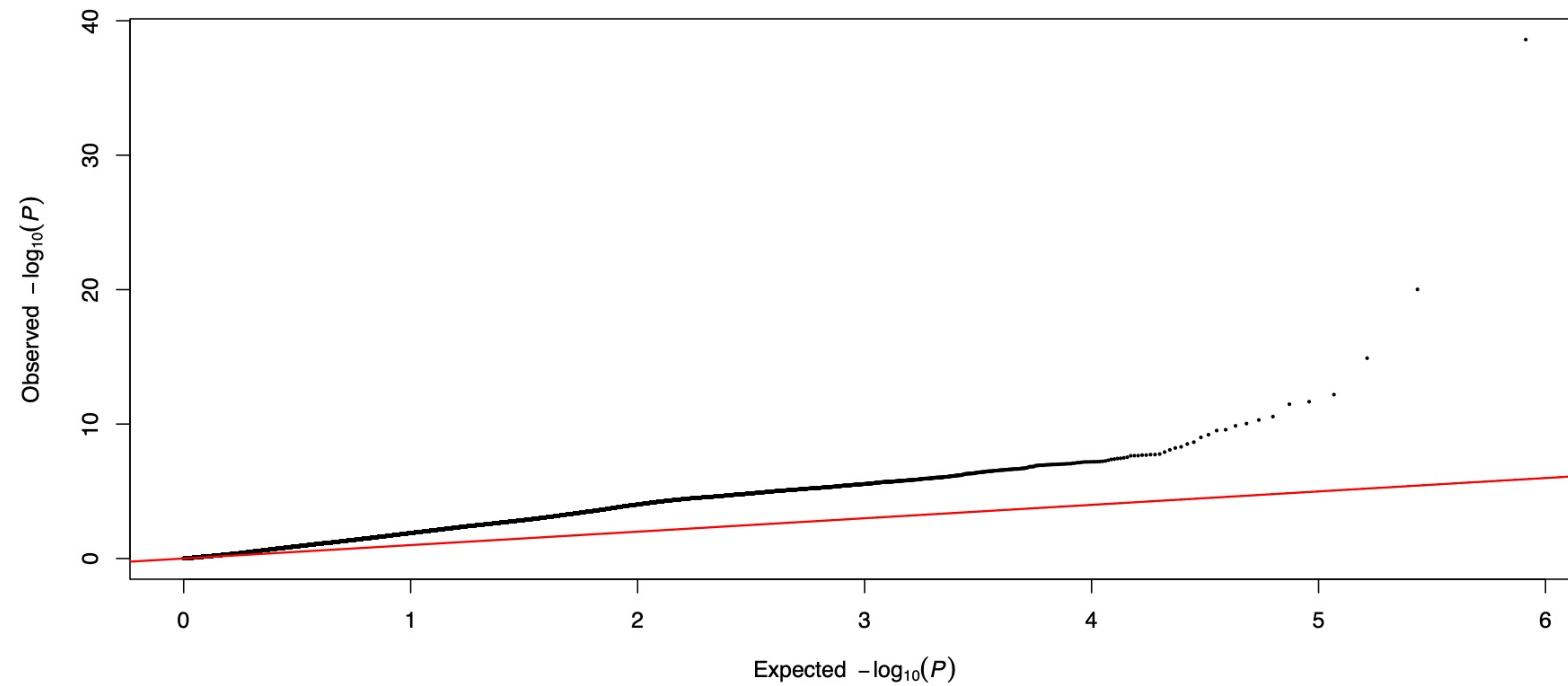
HSW CV0 partition 1 fold 1: Q-Q
