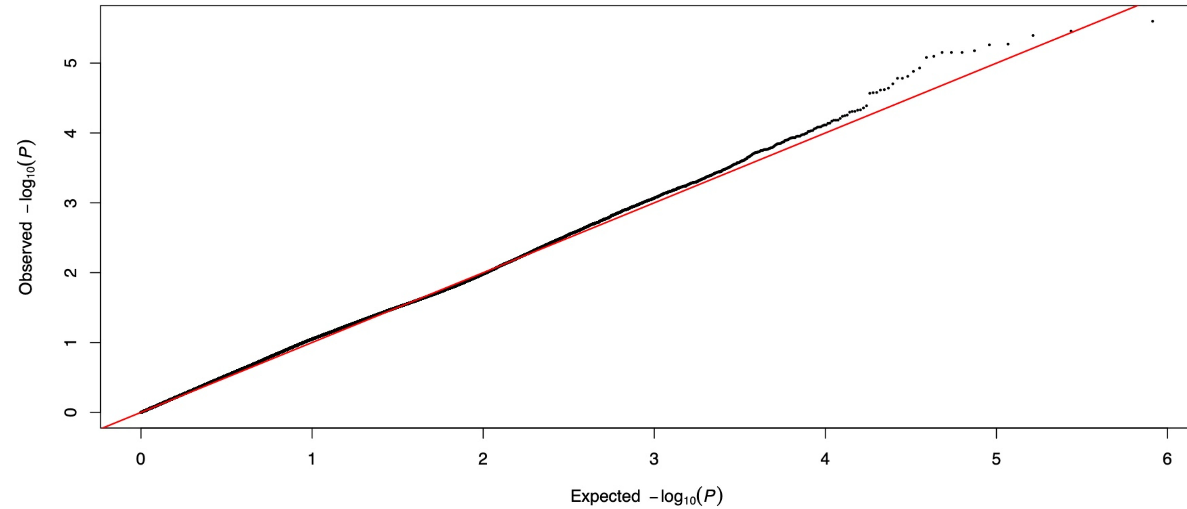
PPP CV2 partition 1 fold 1: Q-Q
