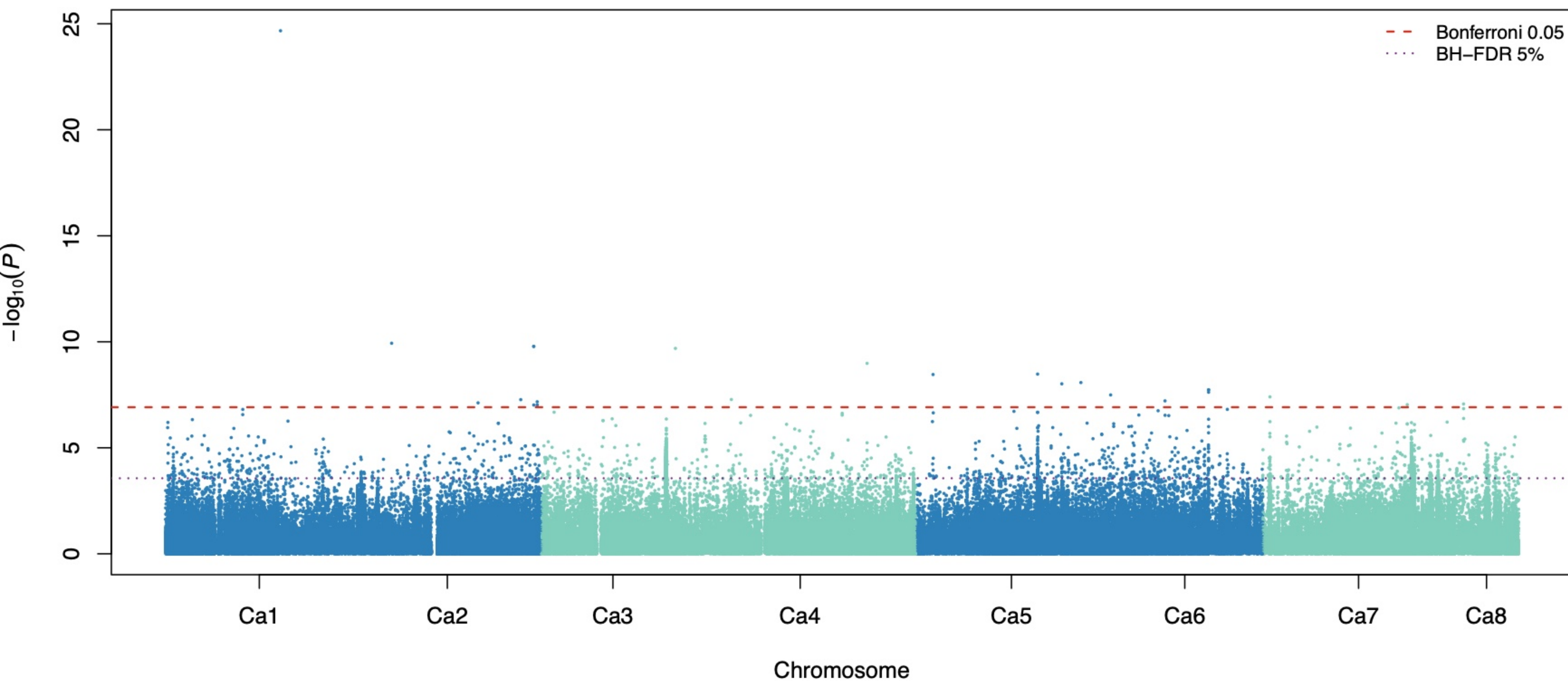
PH CV00 partition 1 fold 1: meta-GWAS
