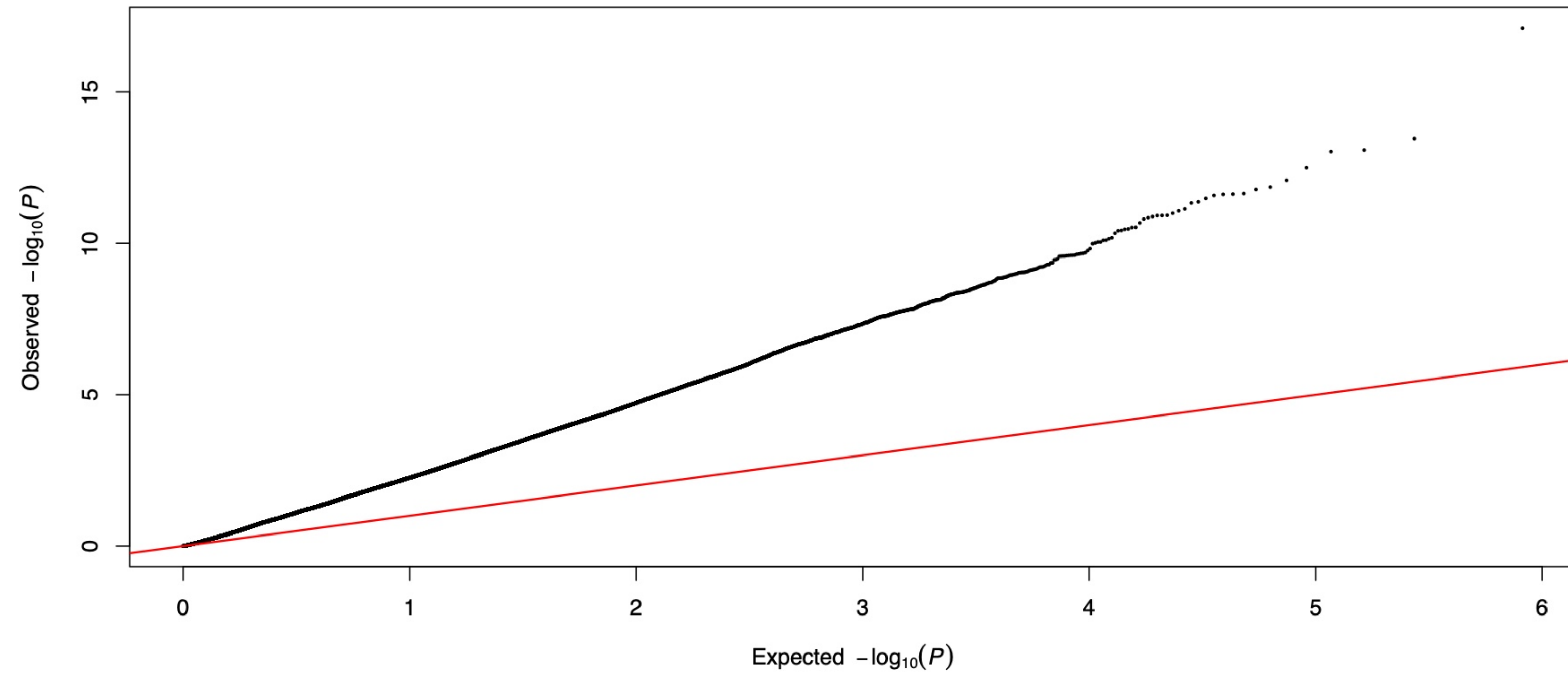
HSW CV1 partition 1 fold 1: Q-Q
