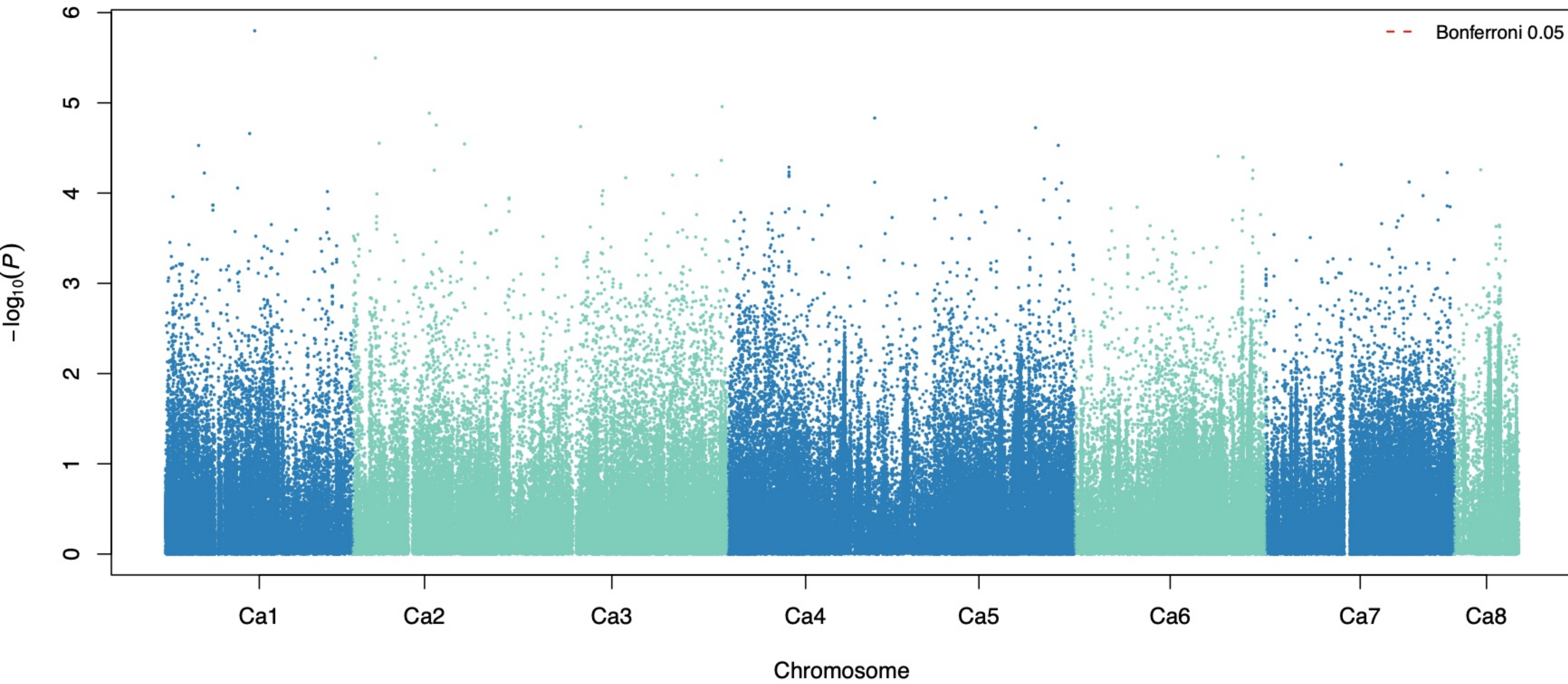
PPP CV1 partition 1 fold 1: meta-GWAS
