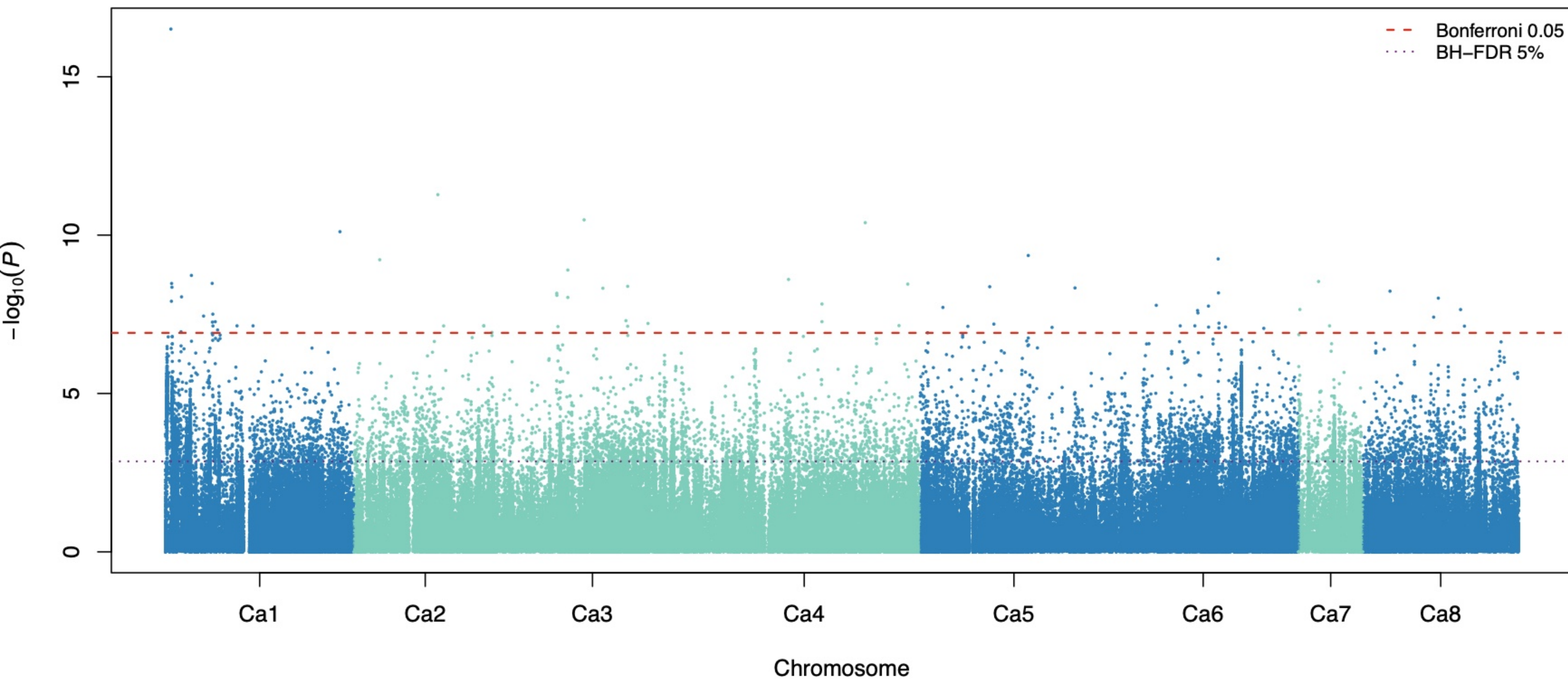
HSW CV00 partition 1 fold 1: meta-GWAS
