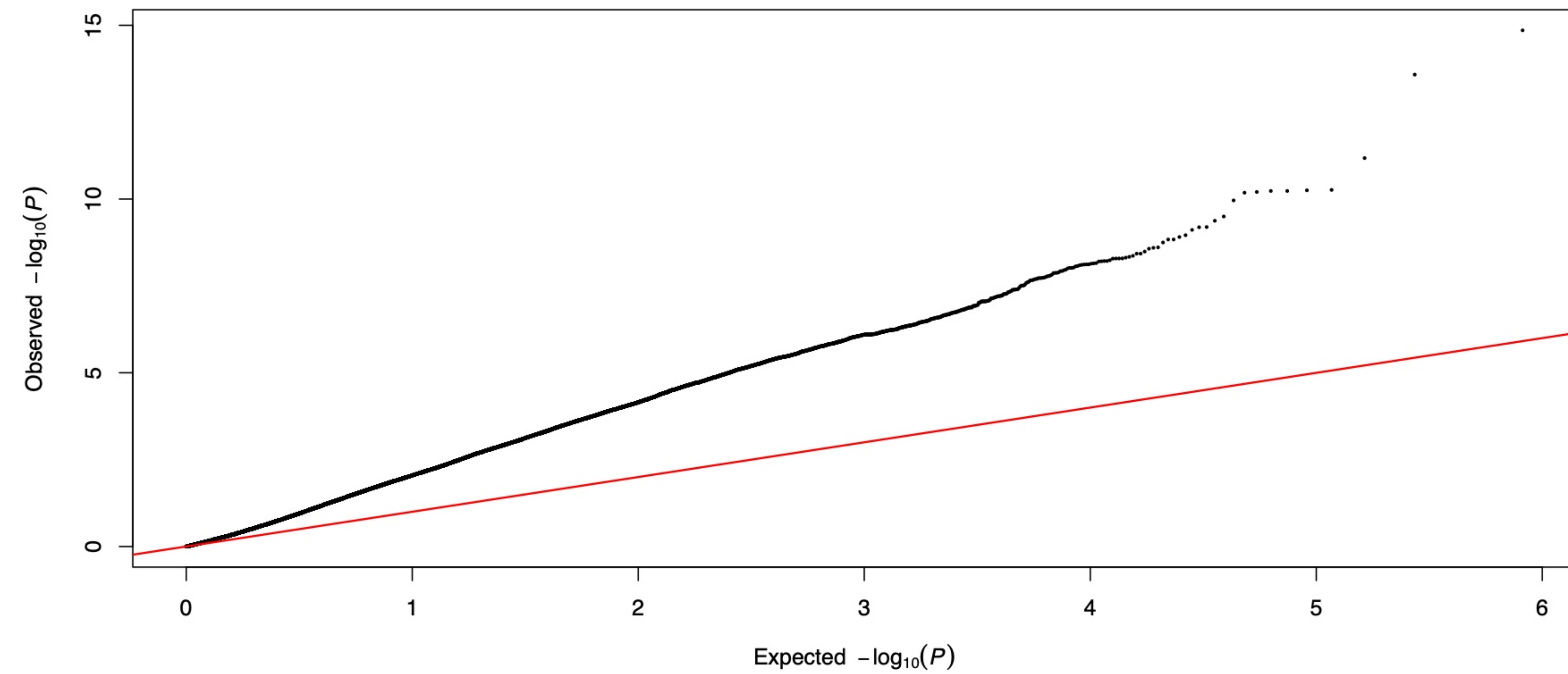
DTM CV0 partition 1 fold 1: Q-Q
