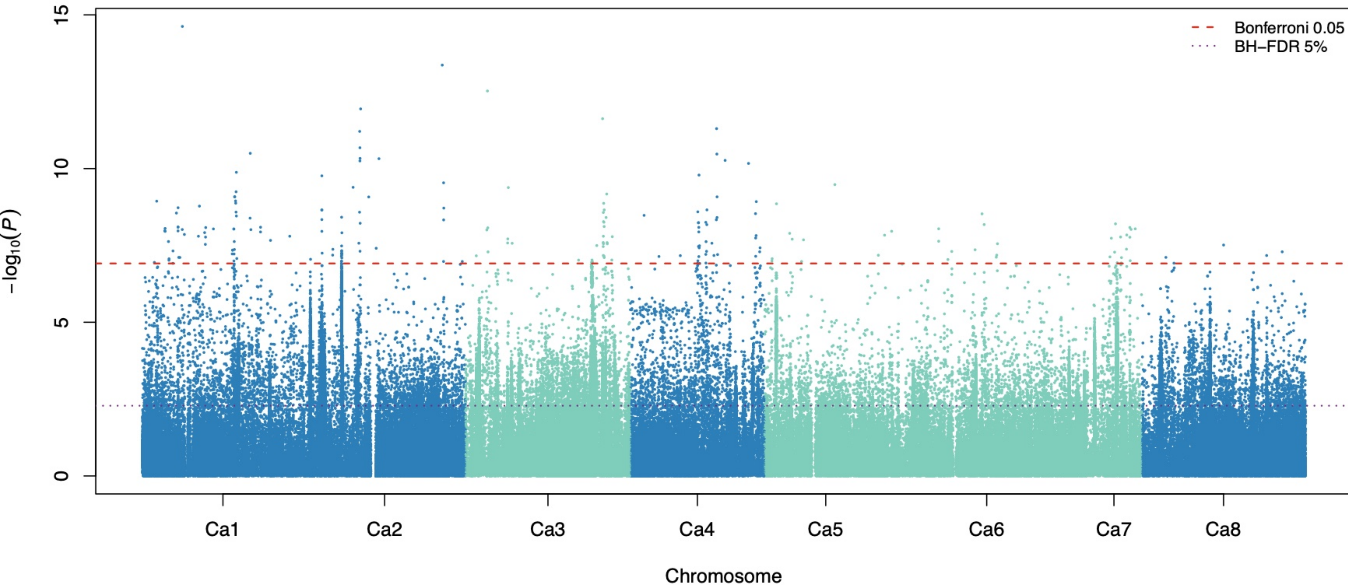
DTM CV1 partition 1 fold 1: meta-GWAS
