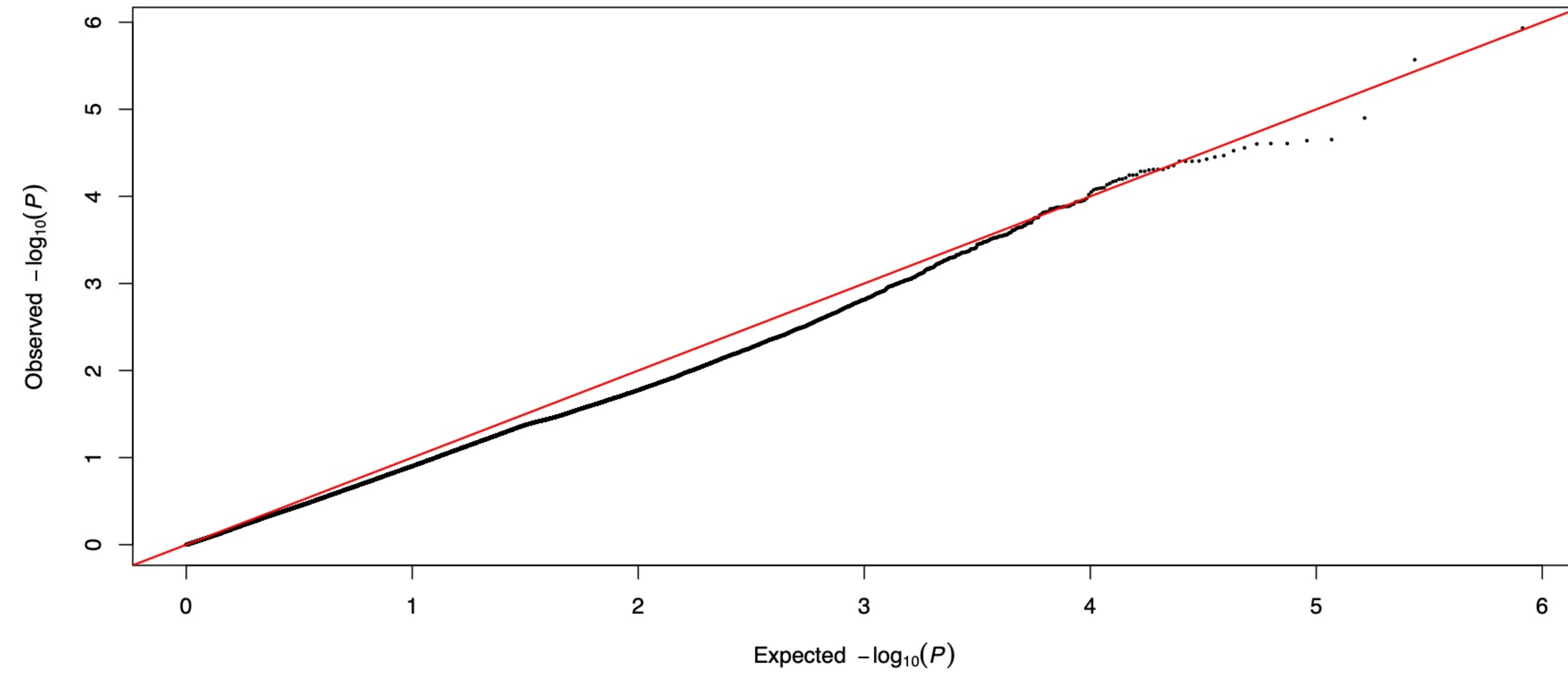
PPP CV0 partition 1 fold 1: Q-Q
