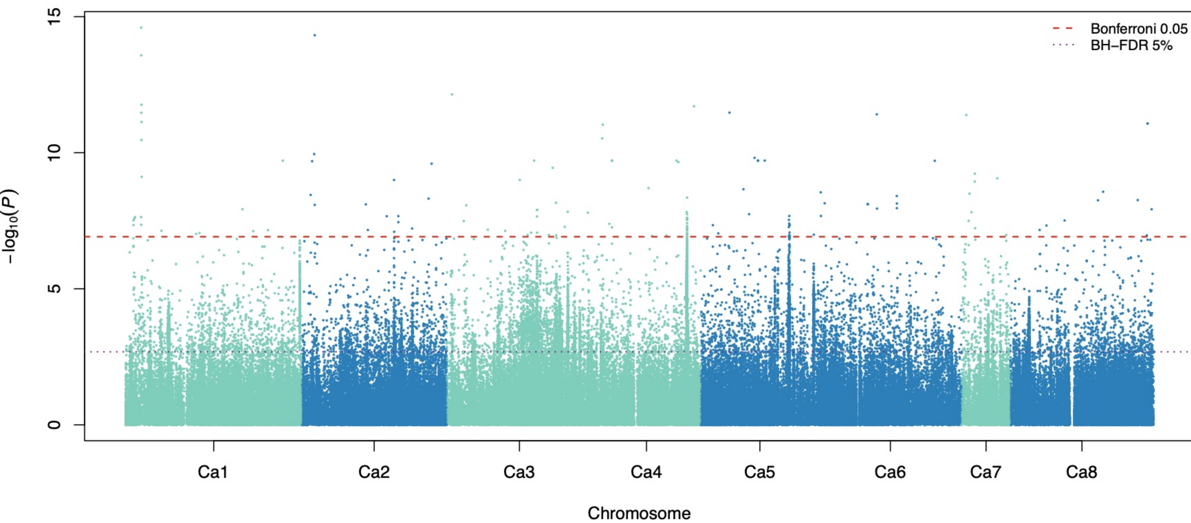
PH CV0 partition 1 fold 1: meta-GWAS
