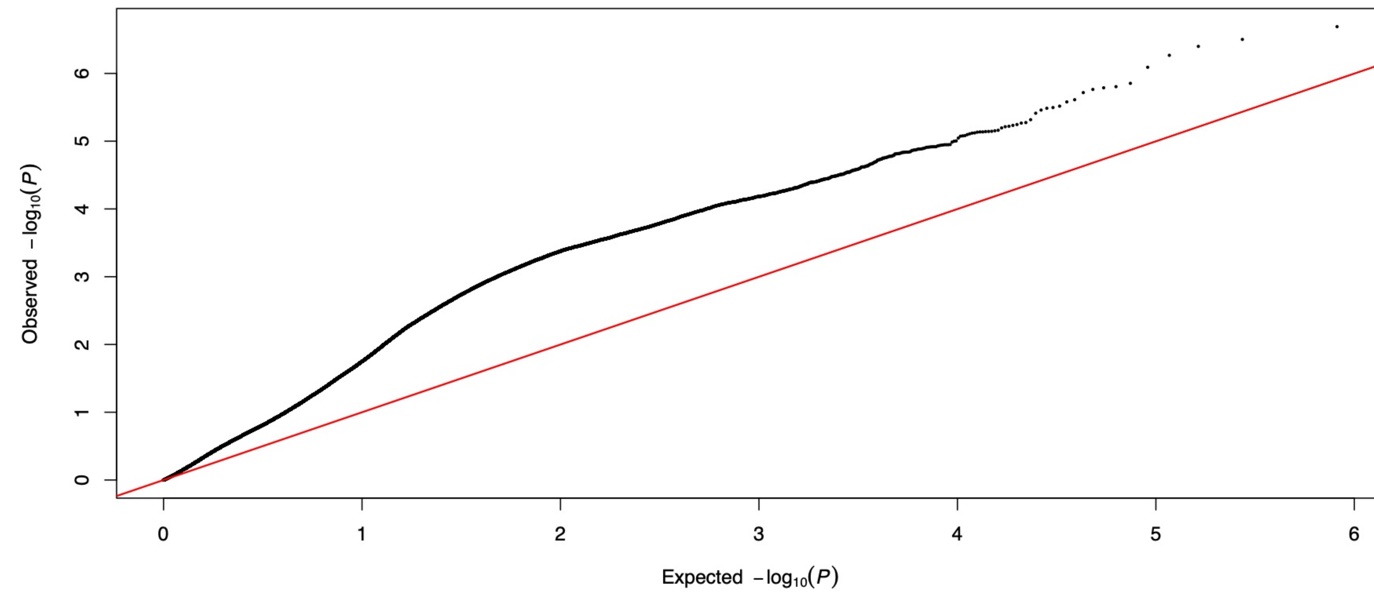
YPP CV00 partition 1 fold 1: Q-Q
