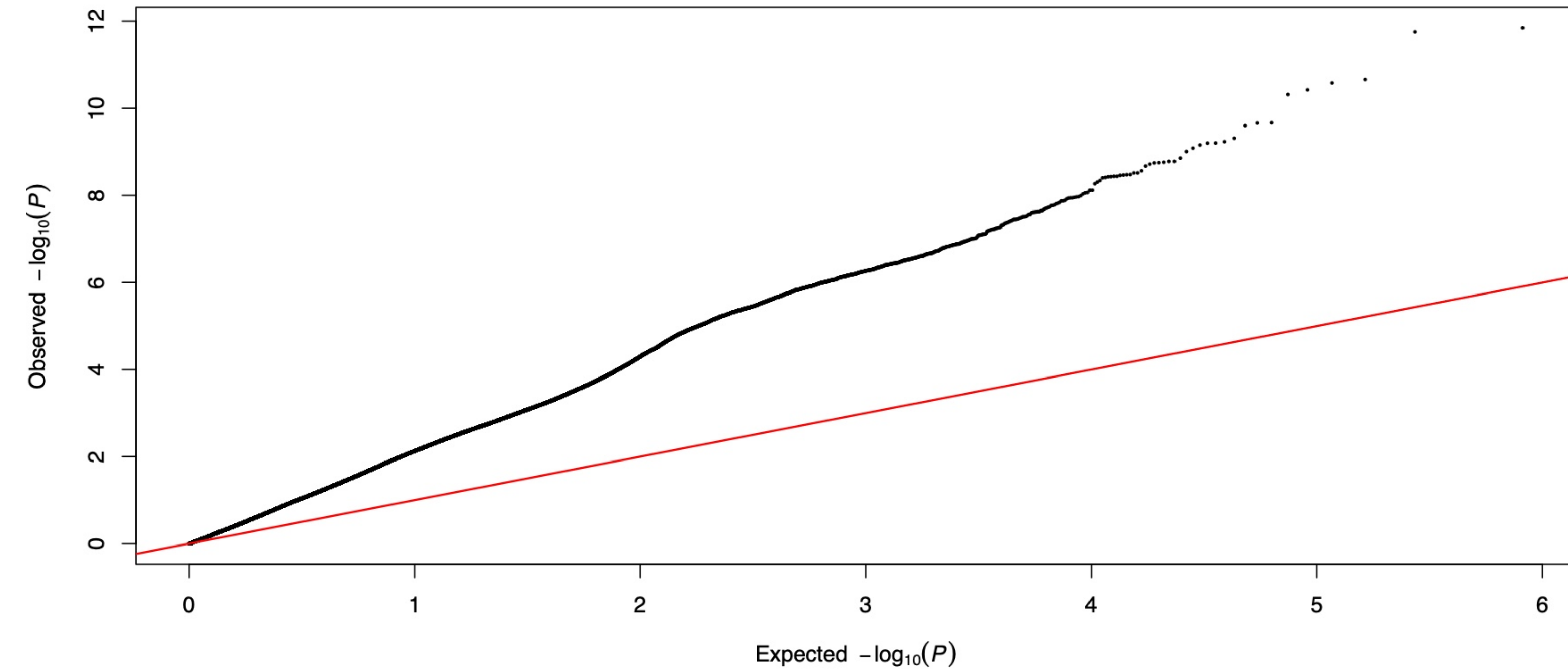
DTM CV2 partition 1 fold 1: Q-Q
