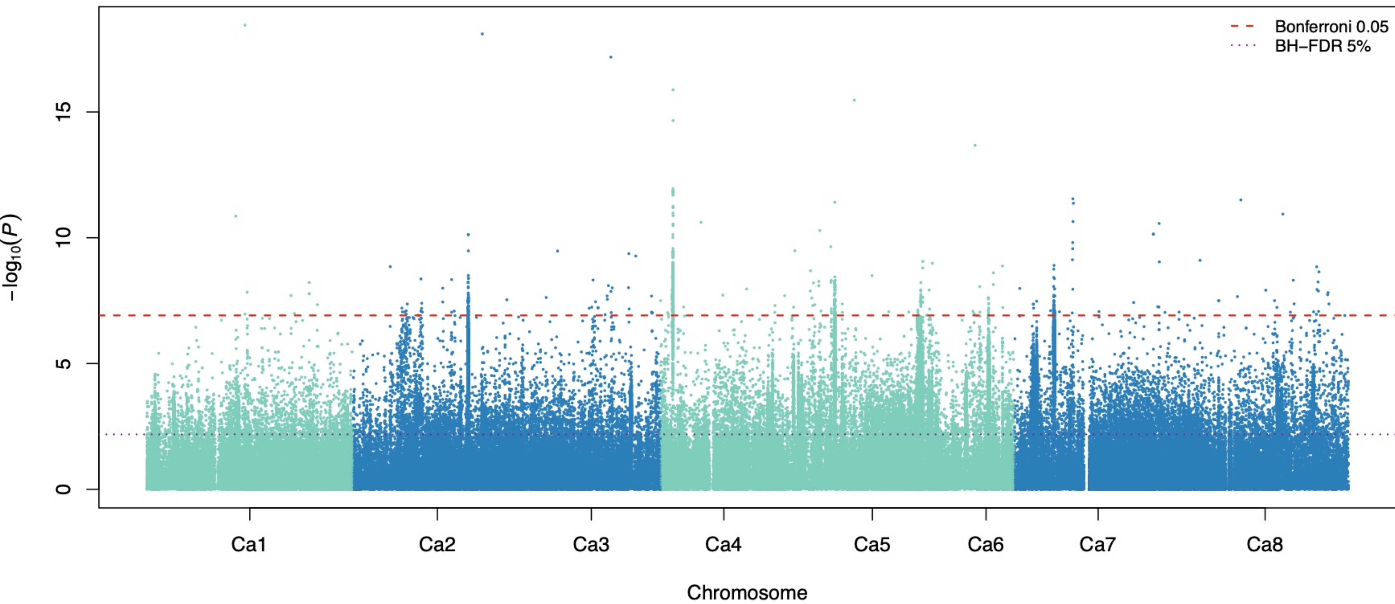
DTF CV0 partition 1 fold 1: meta-GWAS
