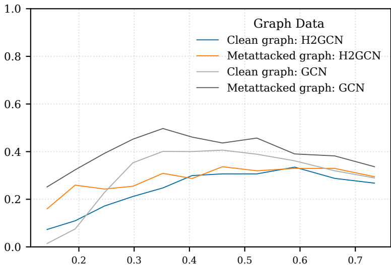
Misclassification rate
