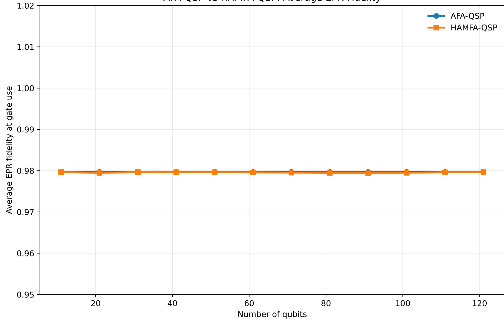
AFA-QSP vs HAMFA-QSP: Average EPR Fidelity
