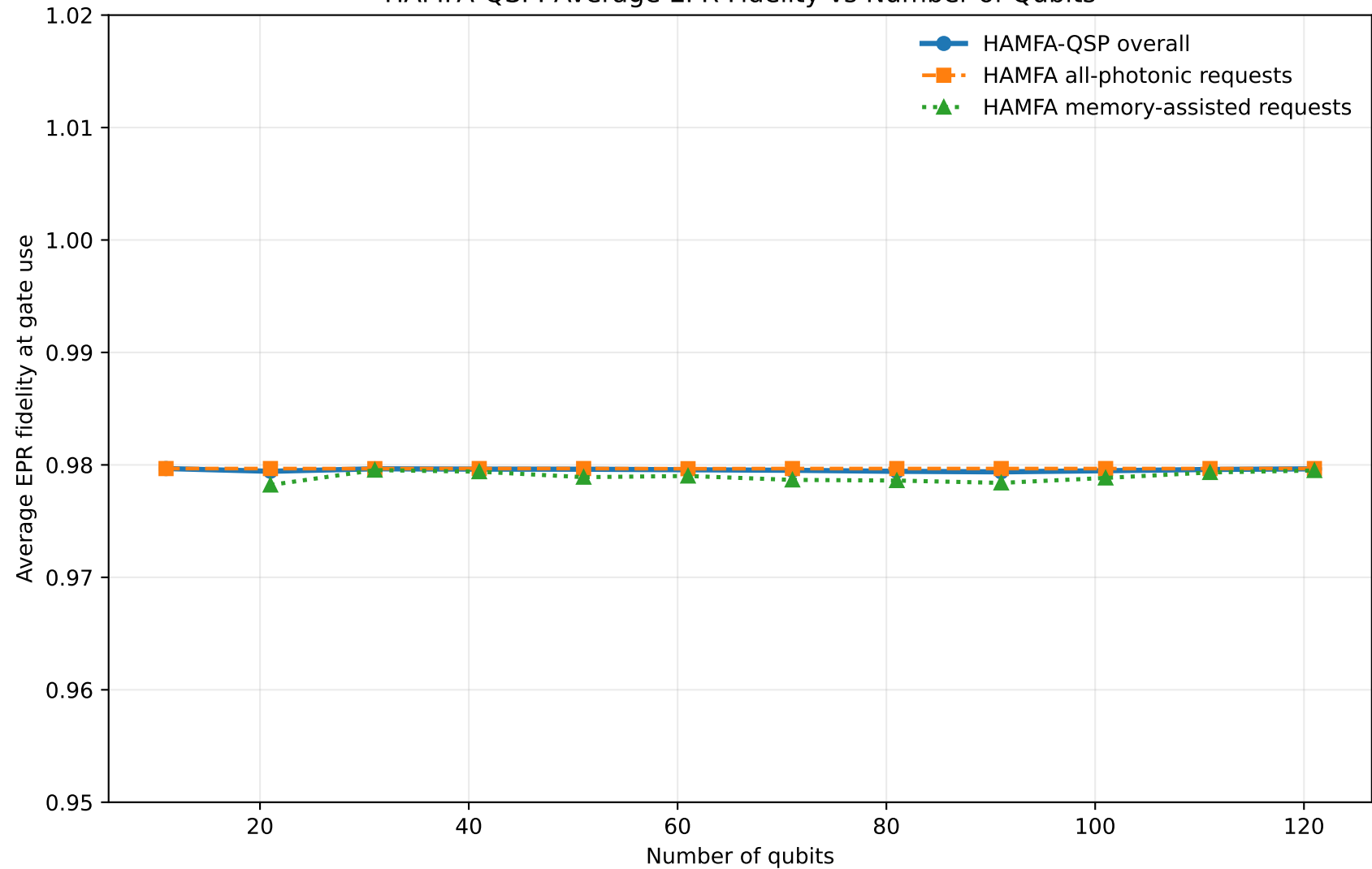
HAMFA-QSP: Average EPR Fidelity vs Number of Qubits
