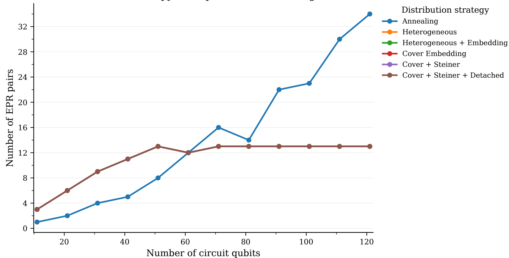
EPR cost across pytket-dqc distribution strategies
