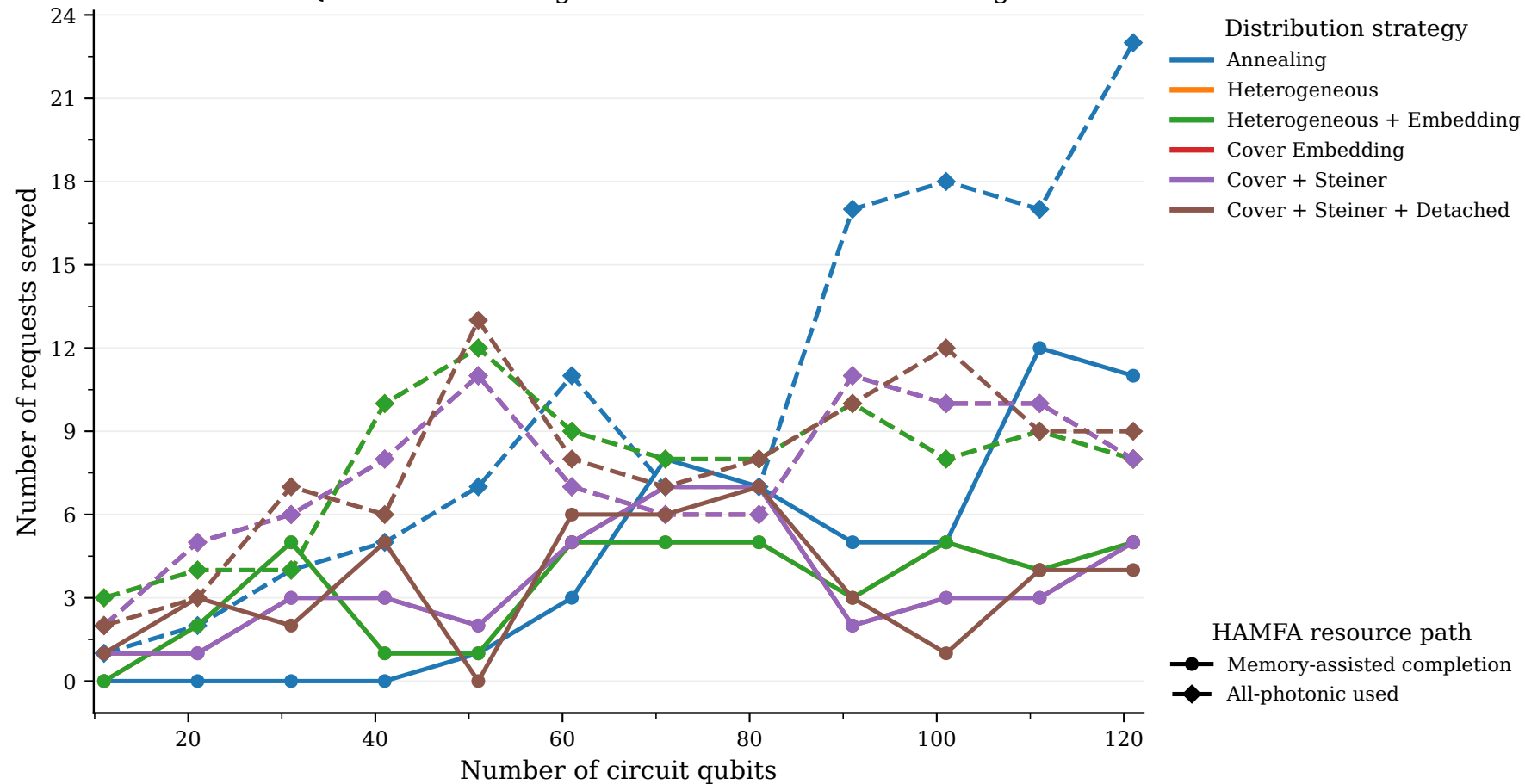
HAMFA-QSP resource usage across all distribution strategies
