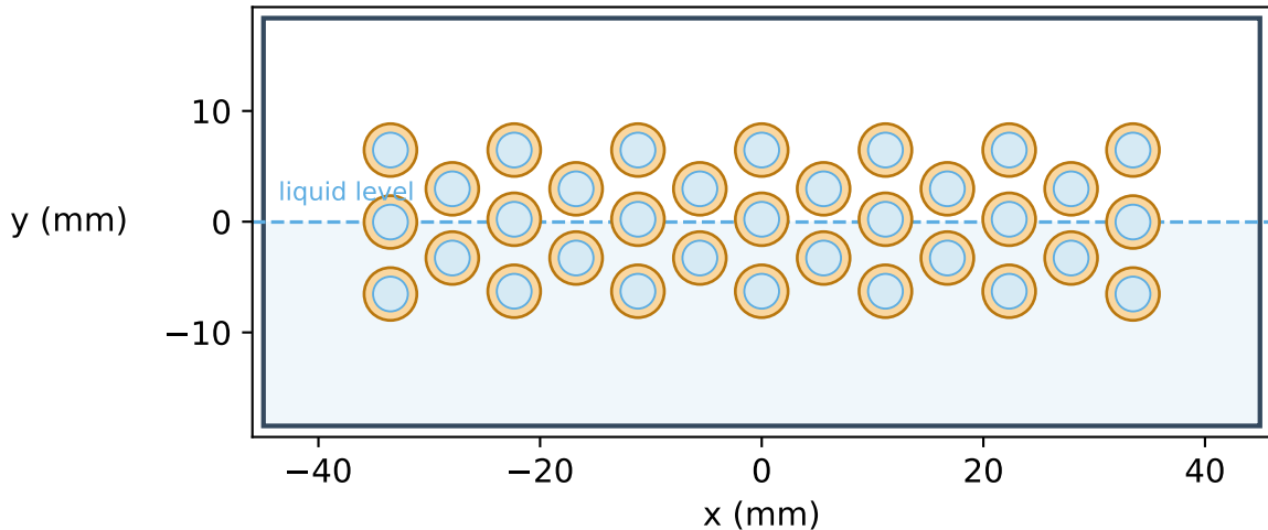
33-tube condenser bundle 33 tubes, OD 4.76 mm, ID 3.137 mm
