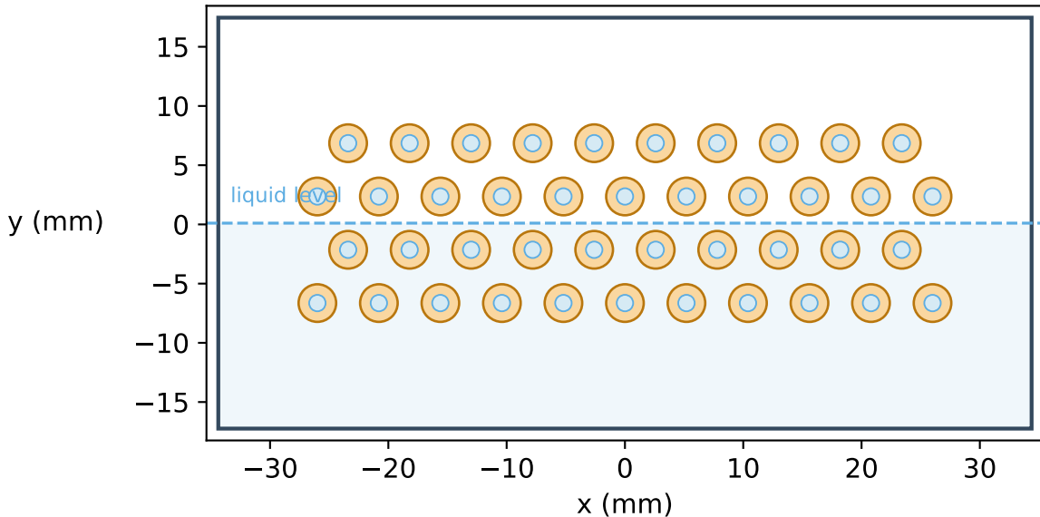
42-tube condenser bundle 42 tubes, OD 3.175 mm, ID 1.39 mm
