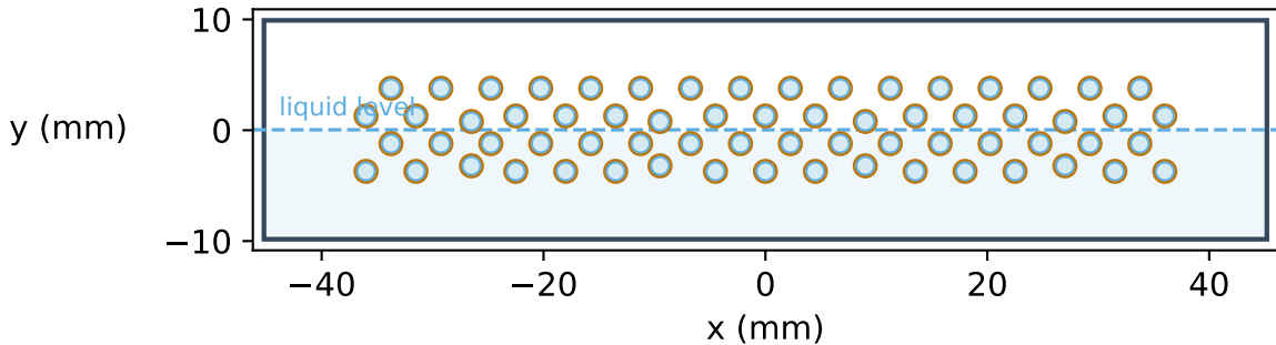
66-tube condenser bundle 66 tubes, OD 2.0 mm, ID 1.6 mm
