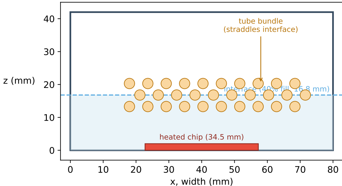
Computational domain, front (x-z) section chamber 80 x 80 x 42 mm, gravity along -z
