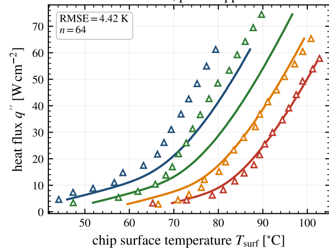
42-tube, plain copper
