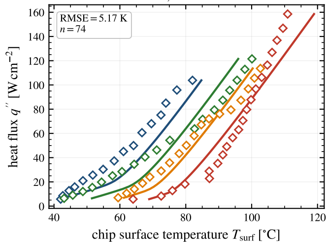
42-tube, microchannel
