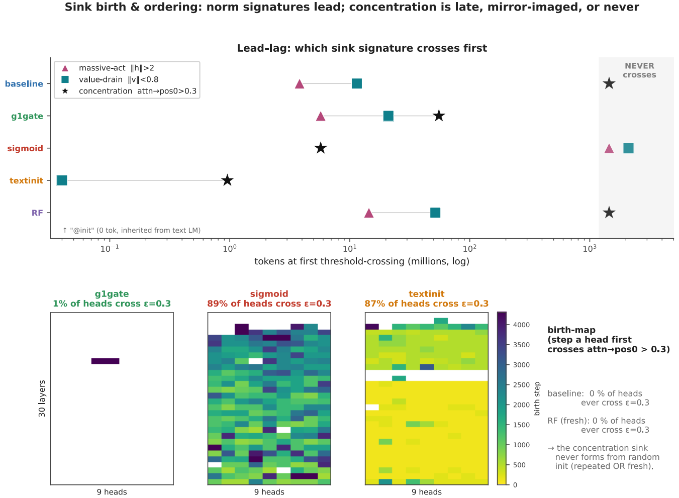
Figure 2: Sink birth & ordering. Top: tokens at which each signature first crosses a per-head threshold (massive-act h > 2 , value-drain v < 0.8 , concentration \text{attn} \rightarrow \text{pos0} > 0.3 ; log scale). In the softmax-from-scratch arms (baseline, g1gate, RF) the norm signatures cross within the first \sim 4 –50M tokens while concentration never crosses (baseline, RF) or barely does (g1gate). sigmoid is the mirror image: concentration crosses at \sim 6 M tokens and the norm signatures never do. textinit starts with value-drain already present at 0 tokens (inherited) and crosses concentration before 1M. Bottom: birth-maps, the step at which each (layer, head) first crosses the concentration threshold. 0% of baseline and RF heads ever cross; 1% of g1gate heads, vs. 89% (sigmoid) and 87% (textinit).
