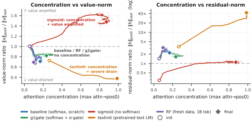
Figure 2: Decoupling phase-portrait. Every arm in concentration-against-value-norm space (left) and against the residual-norm ratio (right, log scale). Circles mark initialization, diamonds the final checkpoint (about 100M tokens, 60M for textinit , 1B for RF ), seed 0 unless labelled. The horizontal axis is the maximum attention \rightarrow pos0 over heads, not Table 1’s fraction, so an arm can sit off zero here with \text{Sink}^\epsilon = 0.000 . Smoothed paths, raw end markers (Appendix F). Were the three signatures one phenomenon, these trajectories would move along one direction.
