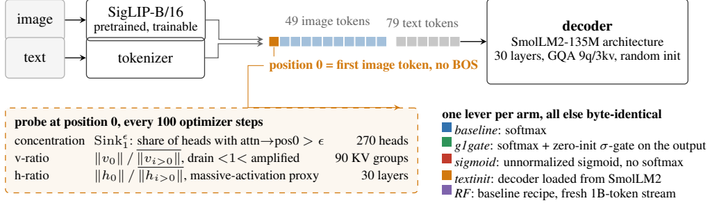
Figure 1: Setup. A pretrained SigLIP-B/16 encoder feeds 49 image tokens, then 79 text tokens, into a randomly initialized decoder of the SmolLM2-135M architecture. There is no BOS token, so position 0 is the first image token. A probe reads three signatures there every 100 steps, each at its own granularity. Four levers change one thing each, and RF repeats the baseline recipe on a fresh 1B-token stream.
