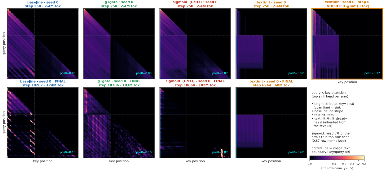
Figure 3: The sink stripe. Query \times key attention of each arm's top sink head, row-normalized, seed 0. Panels carry their seed, step and token count. Top row is early training (step 250, about 2.4M tokens), bottom row the final checkpoint. The cyan line marks key = pos0, the dotted line the image-to-text boundary. The pos0 stripe is absent in baseline throughout and strong in textinit (attn \rightarrow pos0 = 0.62 at its final checkpoint). The rightmost panel shows it already present at step 0 in textinit, inherited from the text language model. The sigmoid column uses head L7H3 , that arm's top sink head on the fixed probe batch. Its heat maps come from an auxiliary streaming batch, while every printed sigmoid number comes from the fixed probe batch (Appendix D).
