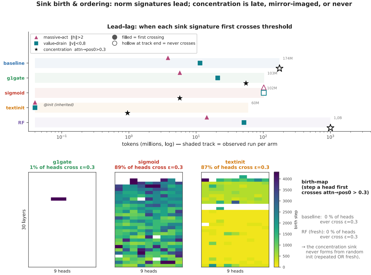
Figure 2: Sink birth and ordering. Seed 0 throughout. Top: time-to-event tracks spanning the tokens over which we observed each arm (60M to 1B). A filled marker is the first probe at which a signature crossed its per-head threshold ( h > 2 , v < 0.8 , \text{attn} \rightarrow \text{pos0} > 0.3 ). A hollow marker at a track’s end means it never crossed. Crossing times are interval-censored at the 100-step probe cadence, so two signatures crossing within one interval should not be read as ordered. Bottom: birth-maps, the step at which each (layer, query-head) pair first crosses the concentration threshold. No baseline and no RF head ever crosses. 1% of glgate heads do, against 89% for sigmoid and 87% for textinit.
