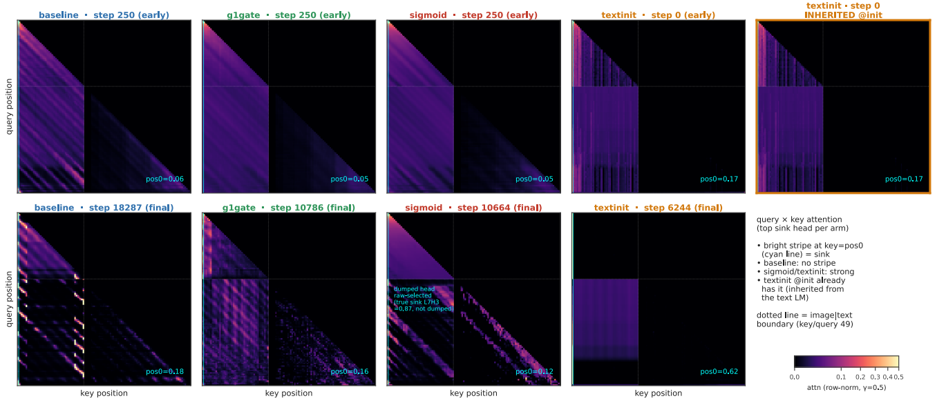
Figure 3: The sink stripe. Query × key attention of the top sink head per arm (row-normalized), early (top row) vs. final (bottom row); the cyan line marks key = pos0 and the dotted line the image|text boundary. The pos0 stripe is absent in baseline throughout, total in textinit (attn→pos0 = 0.62 at its final checkpoint), and, rightmost panel, already present at step 0 in textinit, inherited from the text LM. The sigmoid panel shows a head selected by raw (unnormalized) gate score rather than the arm’s true top sink head and understates sigmoid’s concentration (annotation in panel); we draw no claim about sigmoid from this figure. Its concentration is established in Tables 1–2 and Figure 2.
