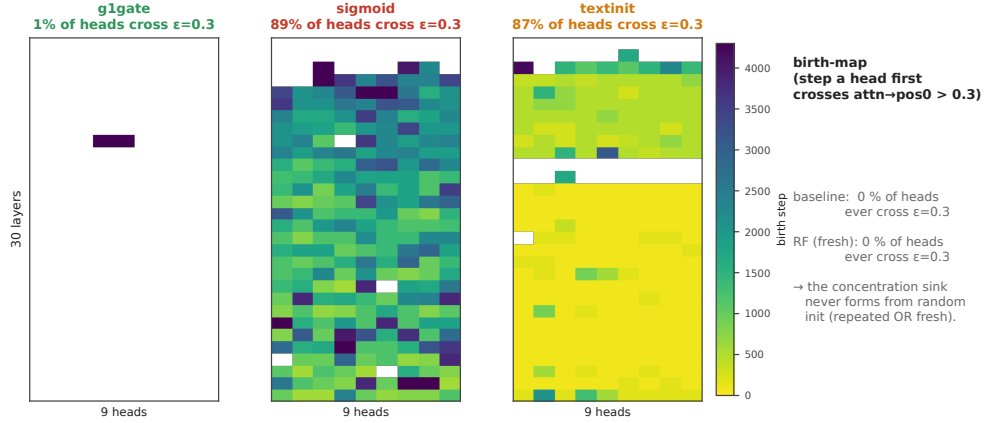
Figure 7: Figure A5: Birth-maps. The step at which each (layer, query-head) pair first crosses the concentration threshold ( \text{attn} \rightarrow \text{pos0} > 0.3 ), seed 0, for the three arms in which any head crosses. No baseline and no RF head ever crosses. 1% of gigate heads do, against 89% for sigmoid and 87% for textinit . This is the head-level view behind Fig. A4.
