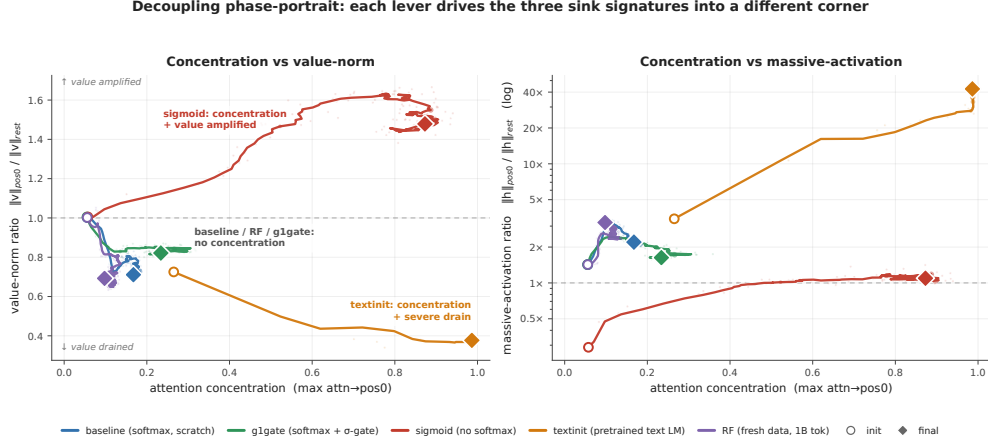
Figure 1: Figure 1: Decoupling phase-portrait. Every arm in concentration-against-value-norm space (left) and against the residual-norm ratio (right, log scale). Circles mark initialization, diamonds the final checkpoint (about 100M tokens, 60M for textinit , 1B for RF ). Seed 0 unless labelled. The horizontal axis is the maximum attention \rightarrow pos0 over heads, not Table 1’s fraction above threshold , so an arm can sit off zero here with Sink ^e = 0.000. Paths smoothed, end markers raw (Appendix D). Were the three signatures one phenomenon, these trajectories would move along one direction.
