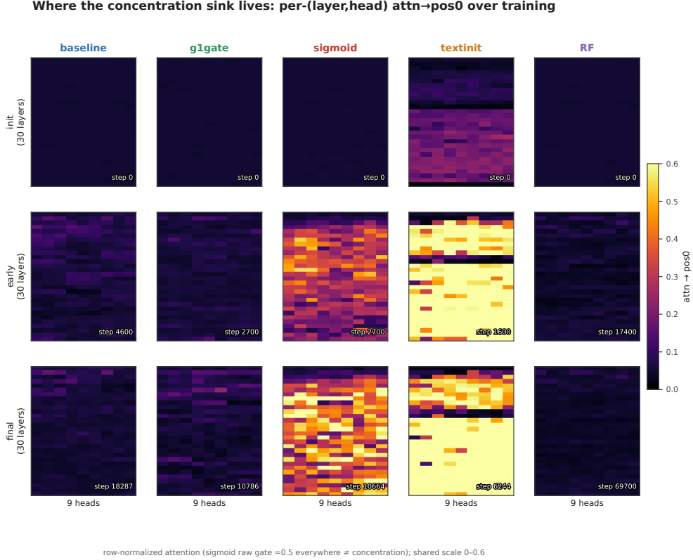
Figure 3: Figure A1: Where concentration lives in the network. Mean attention to pos0 for each of the 270 (layer, query-head) pairs through training, row-normalized, seed 0 for every arm, run to each arm’s final checkpoint (174M tokens baseline, 103M g1gate, 102M sigmoid, 60M textinit, 1B RF). baseline and RF stay cold throughout. textinit is hot from initialization. sigmoid lights up a band of mid-network layers.
