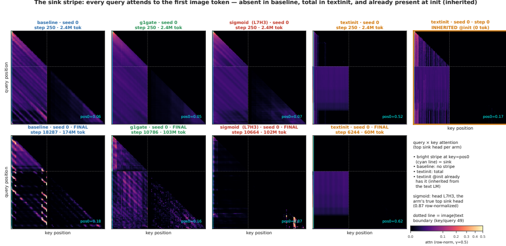
Figure 2: Figure 2: The sink stripe. Query \times key attention of each arm’s top sink head, row-normalized, seed 0. Top row is early training (step 250, about 2.4M tokens), bottom row the final checkpoint. The cyan line marks key = pos0, the dotted line the image-to-text boundary. The stripe is absent in baseline throughout, strong in textinit (attn \rightarrow pos0 = 0.62 at its final checkpoint), and already present at step 0 in textinit (rightmost panel), inherited from the text LM. The sigmoid column’s heat maps come from an auxiliary streaming batch, while every printed sigmoid number comes from the fixed probe batch (Appendix D).
