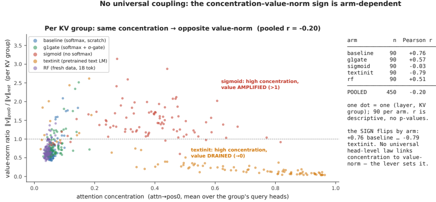
Figure 4: Figure A2: No consistent-sign head-level relationship. Concentration against value-norm ratio for each (layer, KV-group) pair at each arm’s final checkpoint, seed 0, at n = 90 pairs per arm. Grouping this way avoids triplicating each value-norm observation across the 3 query heads that share it, so these correlations are descriptive and we report no p-values (§3.3). The sign of the correlation flips by arm, from +0.76 in baseline to −0.79 in textinit (Table 3). The pooled cloud is weak, at −0.20, only because arms of opposite sign cancel. Do not read it as an uncorrelated cloud. Most individual arms show a strong |r| .
