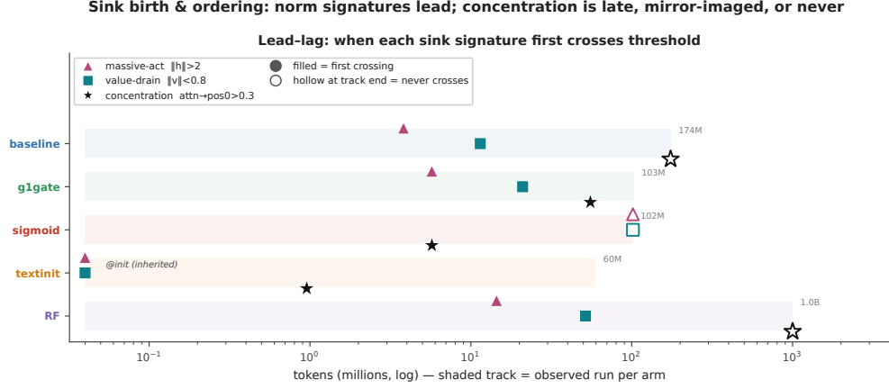
Figure 6: Figure A4: When each signature first crosses threshold. Seed 0 throughout. Time-to-event tracks spanning the tokens over which we observed each arm (60M to 1B). A filled marker is the first probe at which a signature crossed its threshold ( h>2 , v<0.8 , \text{attn} \rightarrow \text{pos0}>0.3 ). A hollow marker at a track’s end means it never crossed. Crossing times are interval-censored at the 100-step probe cadence (head-level map in Fig. A5).
