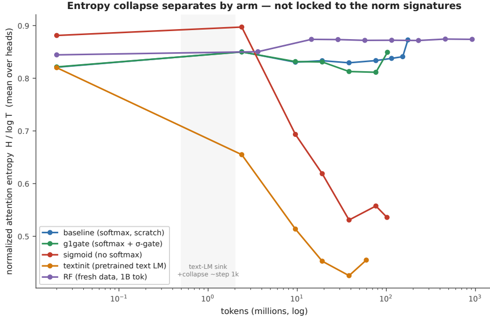
Figure 5: Figure A3: Entropy collapse tracks concentration only. Mean attention entropy through training, seed 0, to each arm’s final checkpoint. Only sigmoid and textinit collapse. baseline, g1gate, and RF stay flat. The entropy-collapse correlate from the text-LM literature therefore follows the concentration axis, not the norm axes.
