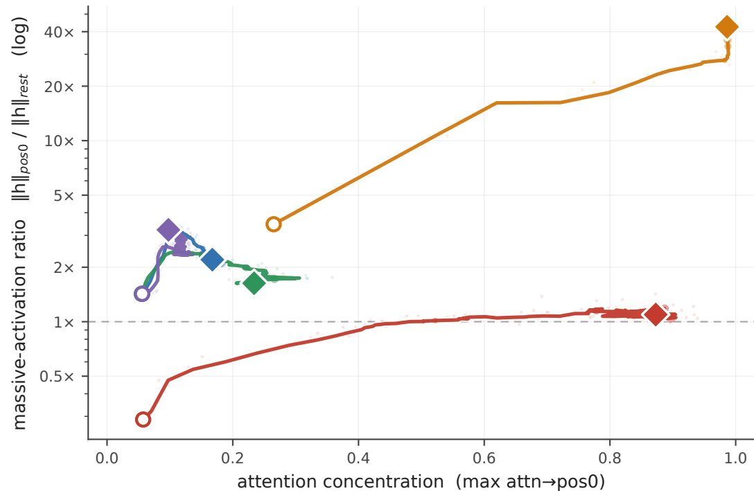
Concentration vs massive-activation
