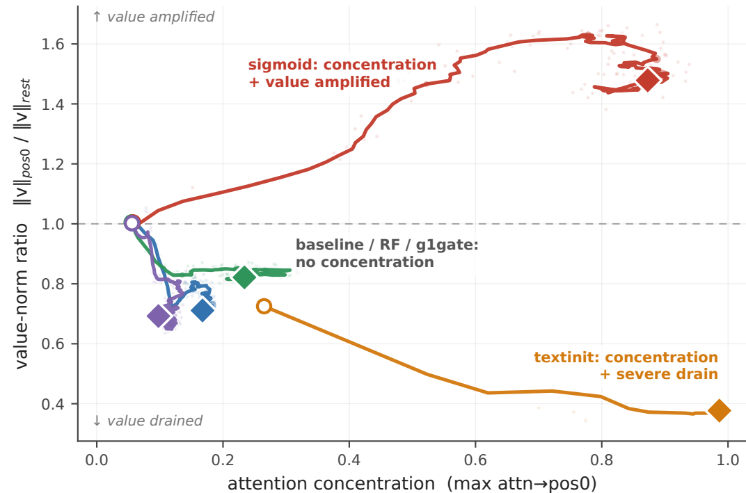
Concentration vs value-norm
