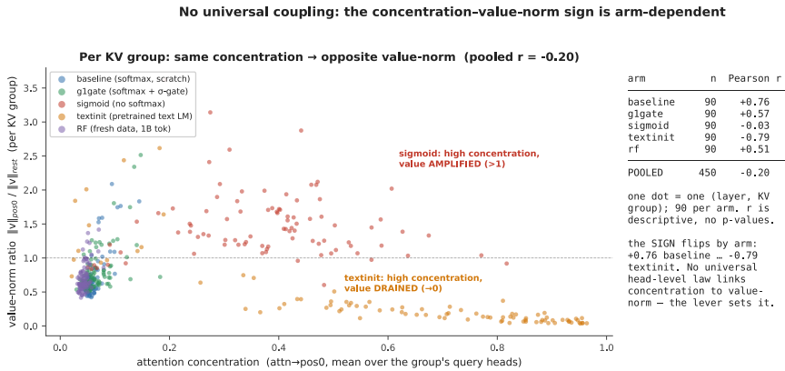
Figure A2: No consistent-sign head-level relationship. Concentration against value-norm ratio for each (layer, KV-group) pair at each arm's final checkpoint, seed 0, at n = 90 pairs per arm. Grouping this way avoids triplicating each value-norm observation across the 3 query heads that share it, so these correlations are descriptive and we report no p-values (§3.3). The sign of the correlation flips by arm, from +0.76 in baseline to -0.79 in textinit (Table 3). The pooled cloud is weak, at -0.20, only because arms of opposite sign cancel. Do not read it as an uncorrelated cloud. Most individual arms show a strong |r| .
