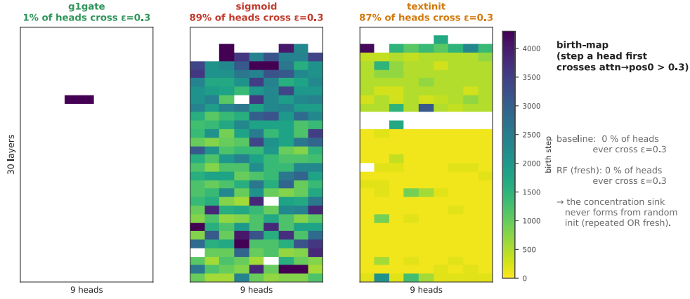
Figure A5: Birth-maps. The step at which each (layer, query-head) pair first crosses the concentration threshold ( \text{attn} \rightarrow \text{pos0} > 0.3 ), seed 0, for the three arms in which any head crosses. No baseline and no RF head ever crosses. 1% of g1gate heads do, against 89% for sigmoid and 87% for textinit . This is the head-level view behind Fig. A4.
