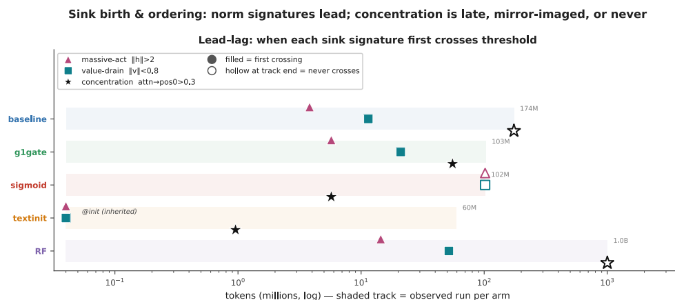
Figure A4: When each signature first crosses threshold. Seed 0 throughout. Time-to-event tracks spanning the tokens over which we observed each arm (60M to 1B). A filled marker is the first probe at which a signature crossed its threshold ( h>2 , v<0.8 , \text{attn} \rightarrow \text{pos0} > 0.3 ). A hollow marker at a track's end means it never crossed. Crossing times are interval-censored at the 100-step probe cadence (head-level map in Fig. A5).
