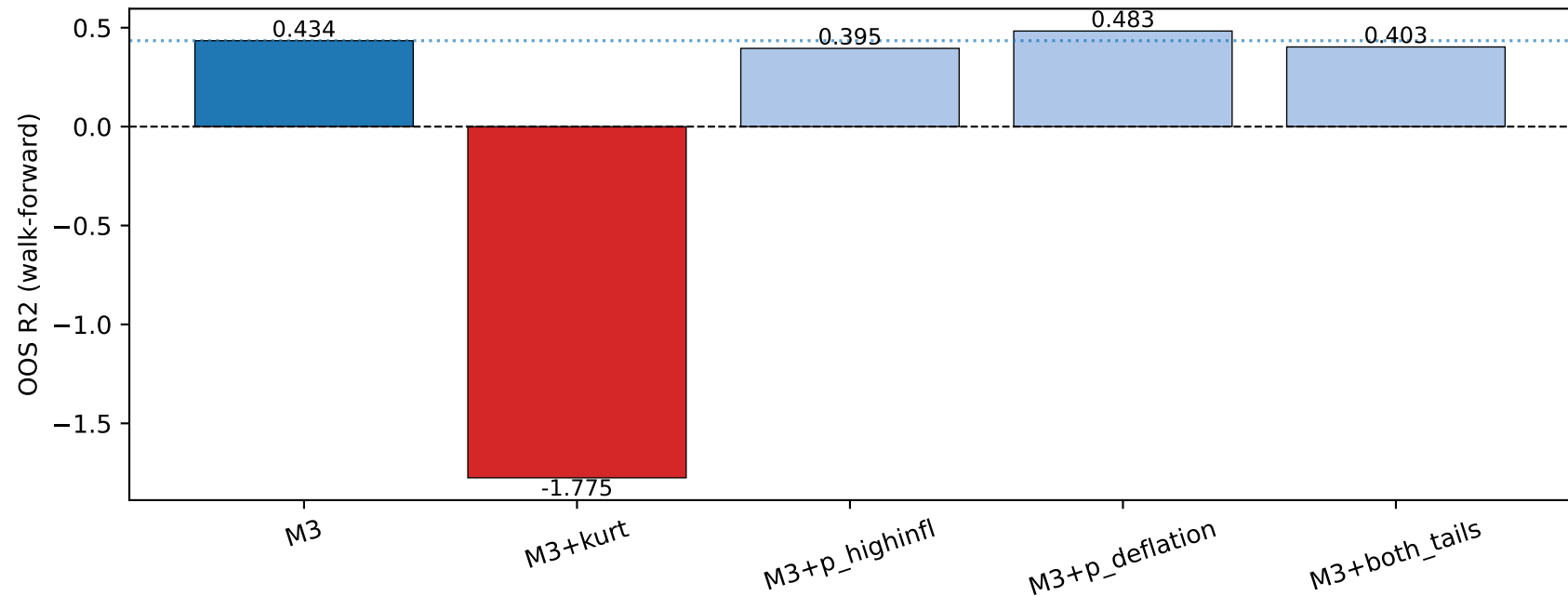
KW: OOS R2 -- M3 vs augmented models (red = overfits OOS, blue = chosen M3)
