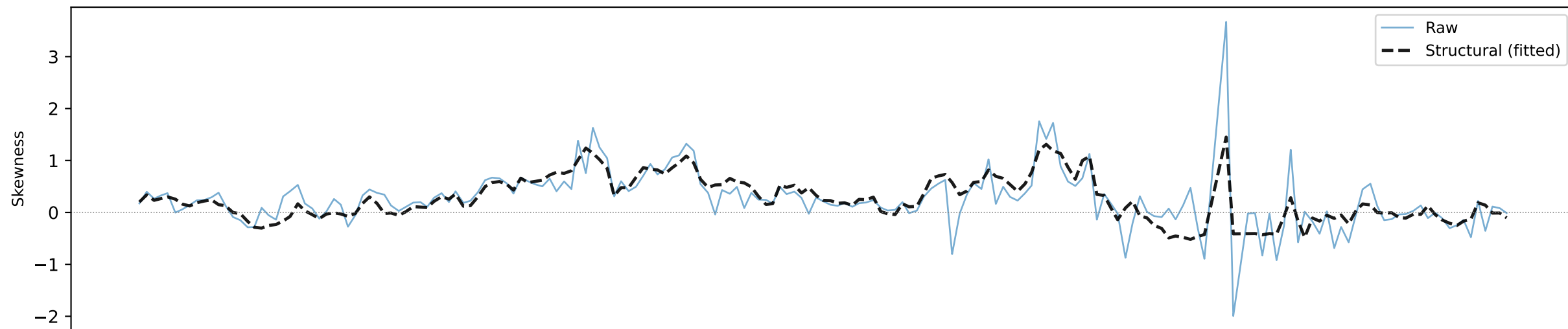
Raw vs Structural skewness (M3: skew ~ mean + var + mean^2)
