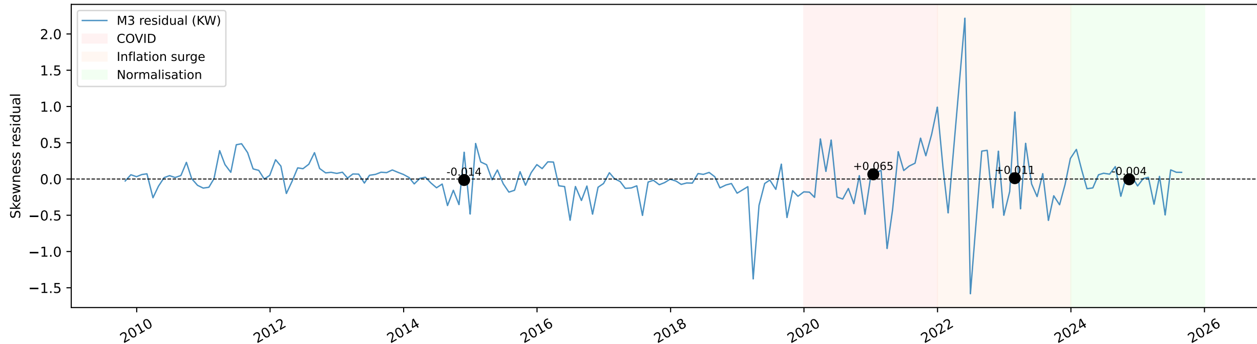
M3 residuals over time (KW) -- era means near zero
