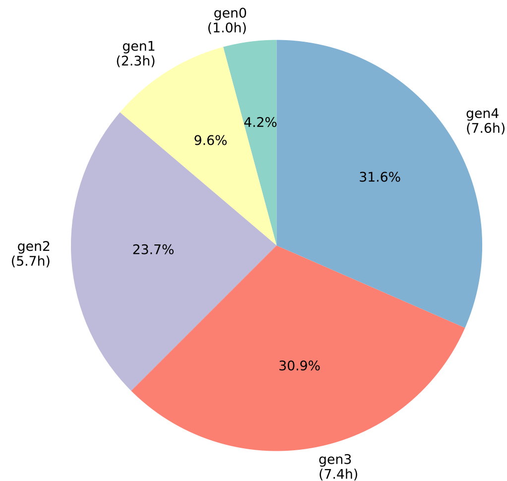
Mongoose ASE Distribution (Total Fuzz: 24.0h)
