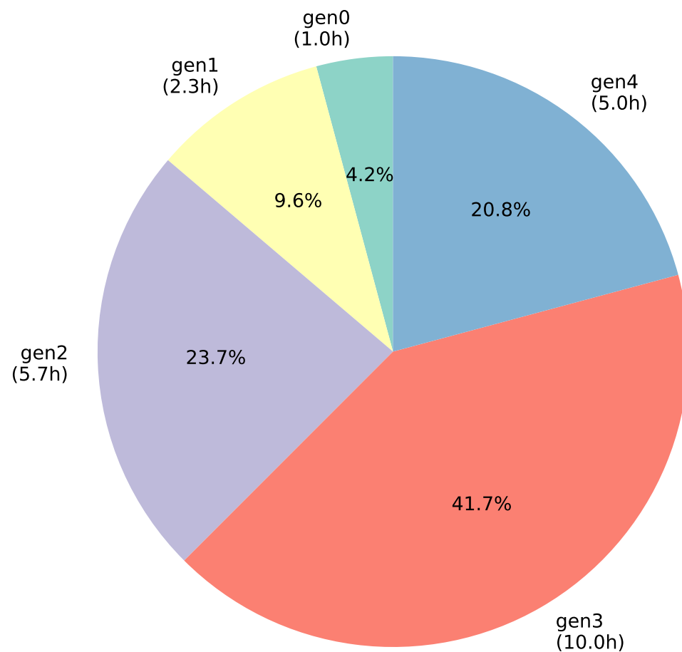
Mosquitto ASE Distribution (Total Fuzz: 24.0h)
