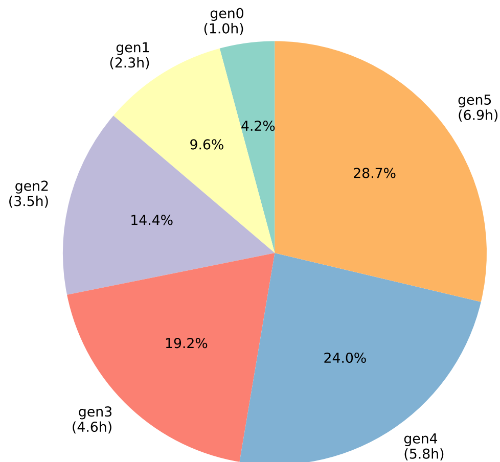
FlashMQ ASE Distribution (Total Fuzz: 24.0h)
