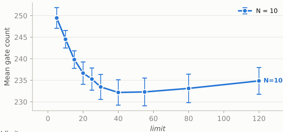
(b) Final result vs scout limit (mean ± SD, gen 3000)
