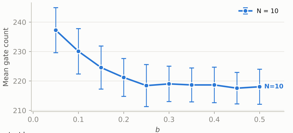
(b) Final result vs spiral constant b (mean \pm SD, gen 3000)
