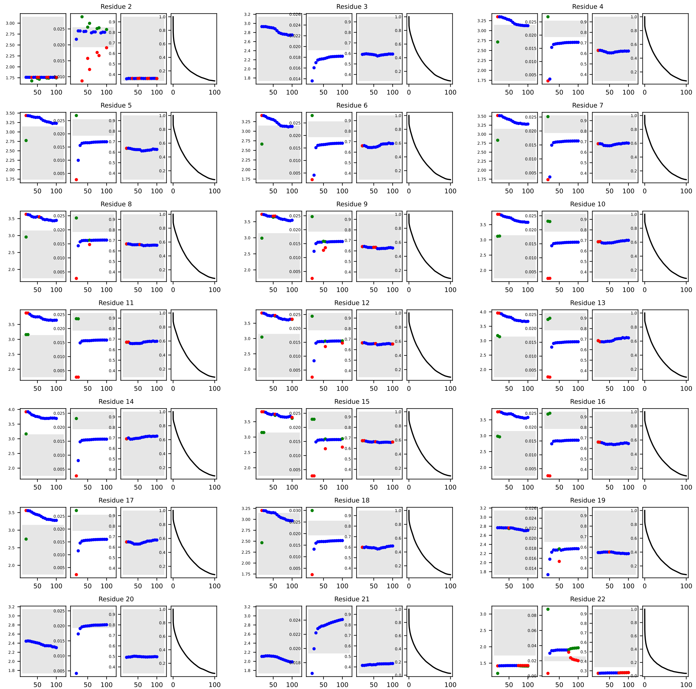
aa-new_90_t_all, simulation length: 3000 ns
