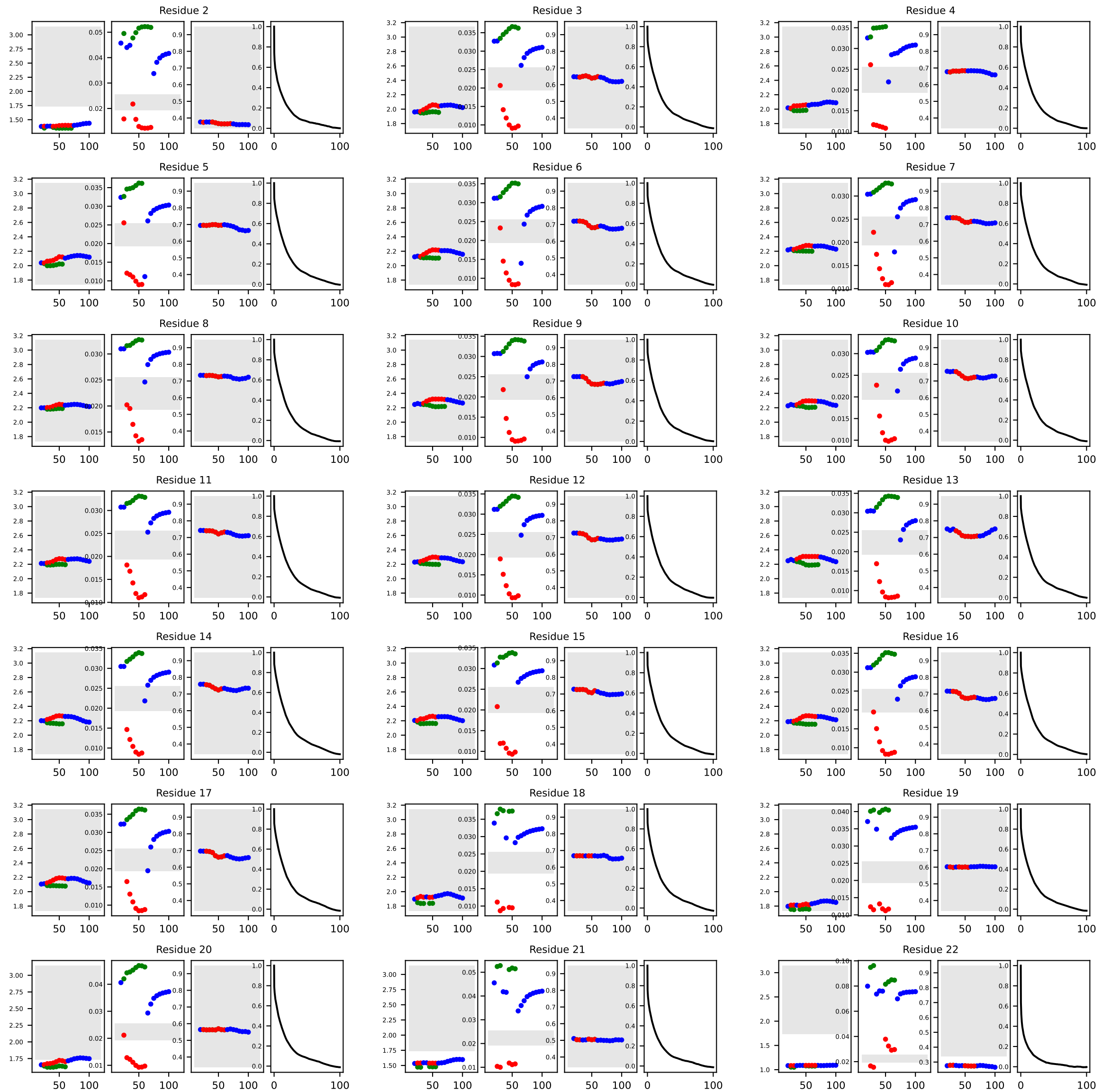
aa_50_b_all, simulation length: 3000 ns
