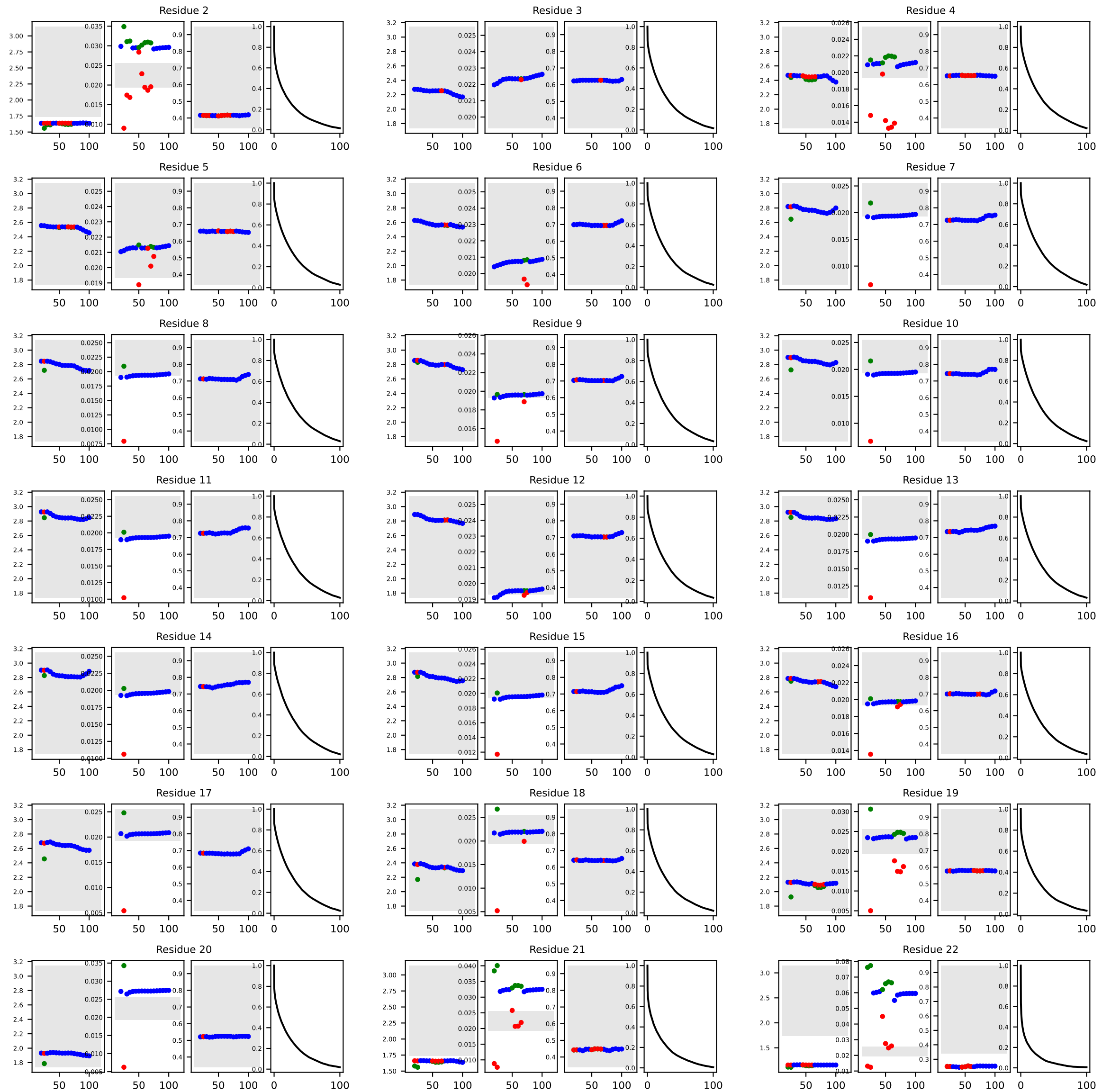
aa_70_2_all, simulation length: 6000 ns
