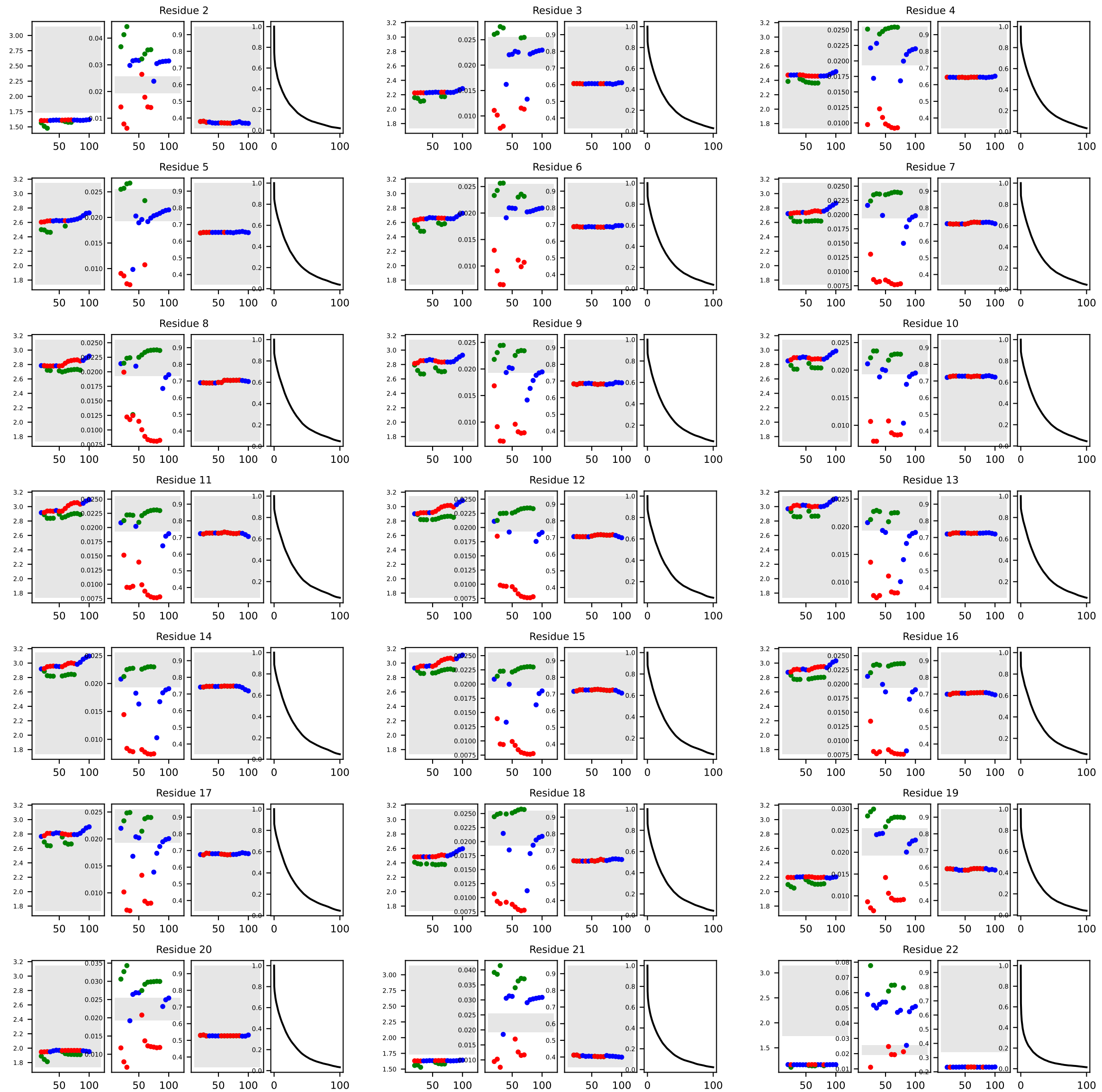
aa_70_3_all, simulation length: 6000 ns
