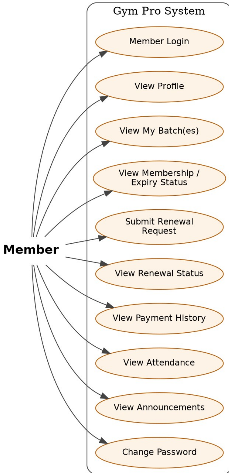
Fig 4.1(b): Use-case diagram – Member
