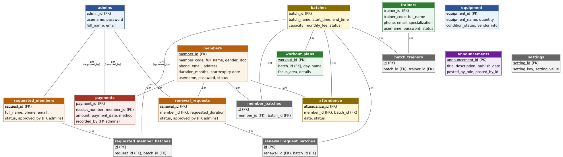
Fig 4.3: Entity-Relationship Diagram of GYM PRO database
