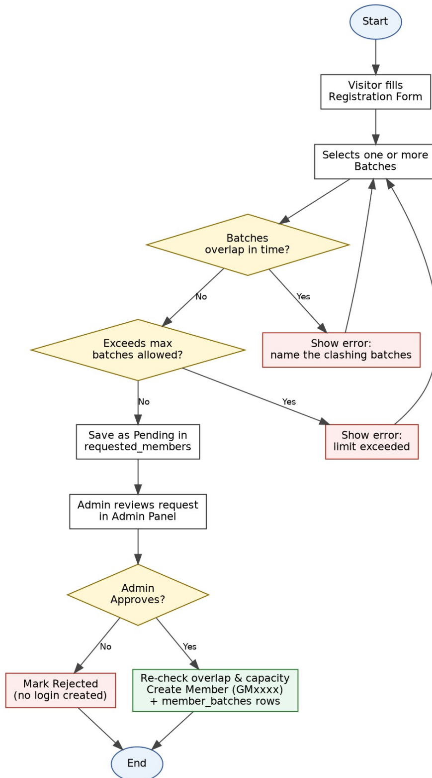
Fig 4.5: Flowchart of the Registration & Approval process
